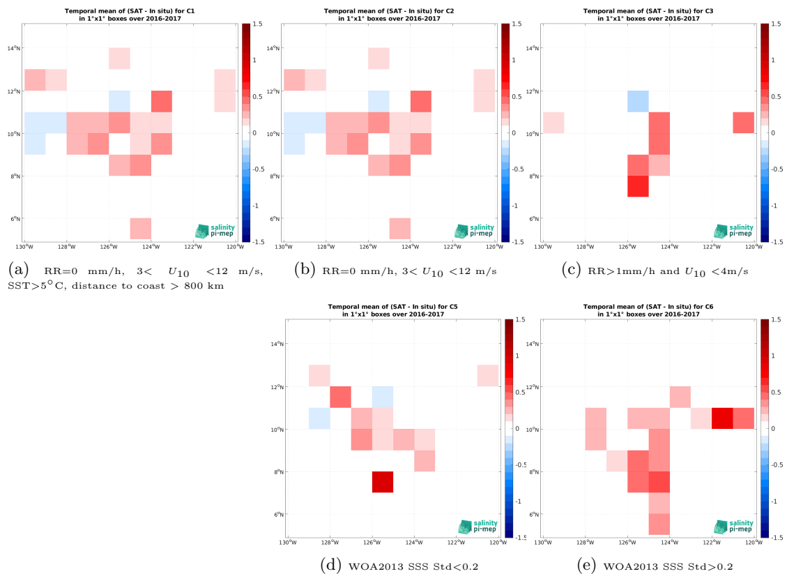
Figure 12: Temporal mean gridded over spatial boxes of size 1^\circ \times 1^\circ of \Delta\text{SSS} (SMOS SSS L3 v332 - 9 Days (CATDS-CPDC) - Salinity Snake (SPURS 2)) for 5 different subdatasets corresponding to:RR=0 mm/h, 3 < U_{10} < 12 m/s, SST>5°C, distance to coast > 800 km (a), RR=0 mm/h, 3 < U_{10} < 12 m/s (b), RR>1mm/h and U_{10} < 4 m/s (c), WOA2013 SSS Std<0.2 (d), WOA2013 SSS Std>0.2 (e).
