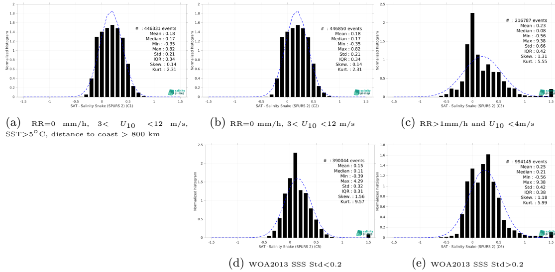
Figure 13: Normalized histogram of \Delta SSS (SMOS SSS L3 v332 - 9 Days (CATDS-CPDC) - Salinity Snake (SPURS 2)) for 5 different subdatasets corresponding to: RR=0 mm/h, 3 < U_{10} < 12 m/s, SST>5°C, distance to coast > 800 km (a), RR=0 mm/h, 3 < U_{10} < 12 m/s (b), RR>1mm/h and U_{10} < 4 m/s (c), WOA2013 SSS Std<0.2 (d), WOA2013 SSS Std>0.2 (e).
