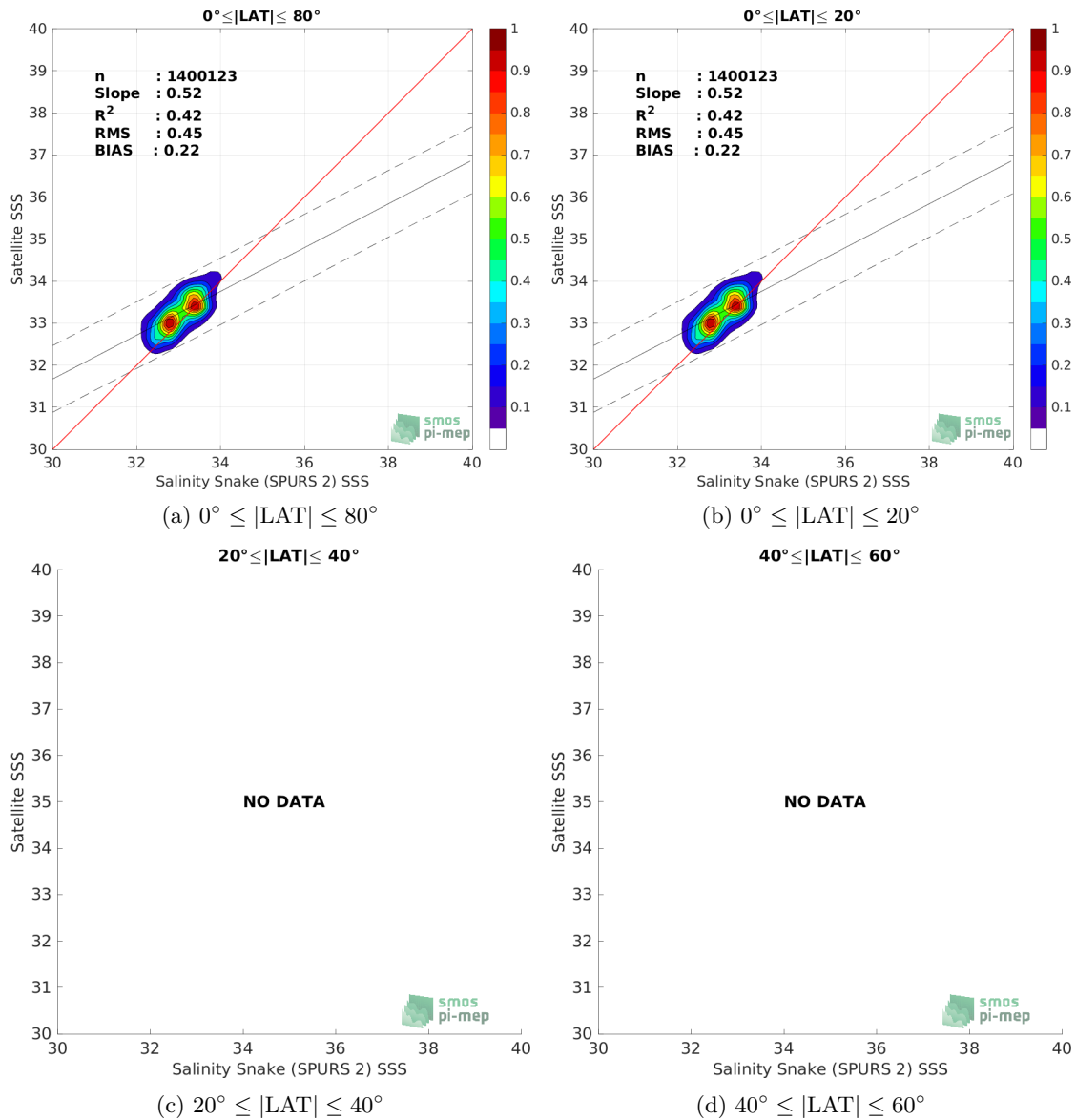
Figure 9: Contour maps of the concentration of SMOS SSS L3 v332 - 9 Days (CATDS-CPDC) SSS (y-axis) versus Salinity Snake (SPURS 2) SSS (x-axis) at match-up pairs for different latitude bands. For each plot, the red line shows x=y . The black thin and dashed lines indicate a linear fit through the data cloud and the \pm 95\% confidence levels, respectively. The number match-up pairs n , the slope and R^2 coefficient of the linear fit, the root mean square (RMS) and the mean bias between satellite and in situ data are indicated for each latitude band in each plots.
