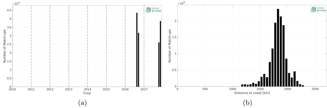
Figure 1: Number of match-ups between Salinity Snake (SPURS 2) and SMOS SSS L3 v332 - 9 Days (CATDS-CPDC) SSS as a function of time (a) and as function of the distance to coast (b) over the SPURS 2 Pi-MEP region and for the full satellite product period.
