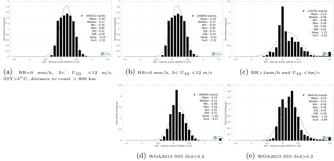
Figure 13: Normalized histogram of \Delta SSS (SMOS SSS L3 v332 - 9 Days (CATDS-CPDC) - Salinity Snake (SPURS 2)) for 5 different subdatasets corresponding to: RR=0 mm/h, 3 < U_{10} < 12 m/s, SST>5°C, distance to coast > 800 km (a), RR=0 mm/h, 3 < U_{10} < 12 m/s (b), RR>1mm/h and U_{10} < 4 m/s (c), WOA2013 SSS Std<0.2 (d), WOA2013 SSS Std>0.2 (e).
