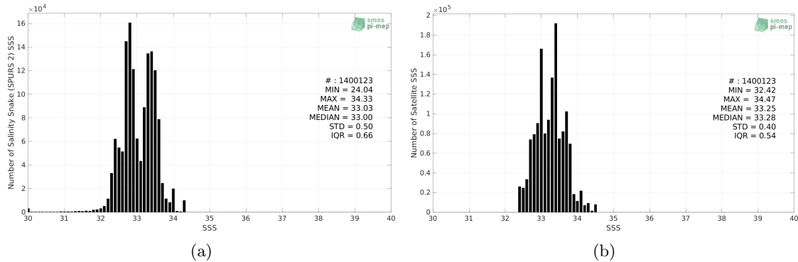
Figure 2: Histograms of SSS from Salinity Snake (SPURS 2) (a) and SMOS SSS L3 v332 - 9 Days (CATDS-CPDC) (b) considering all match-up pairs per bins of 0.1 over the SPURS 2 Pi-MEP region and for the full satellite product period.
