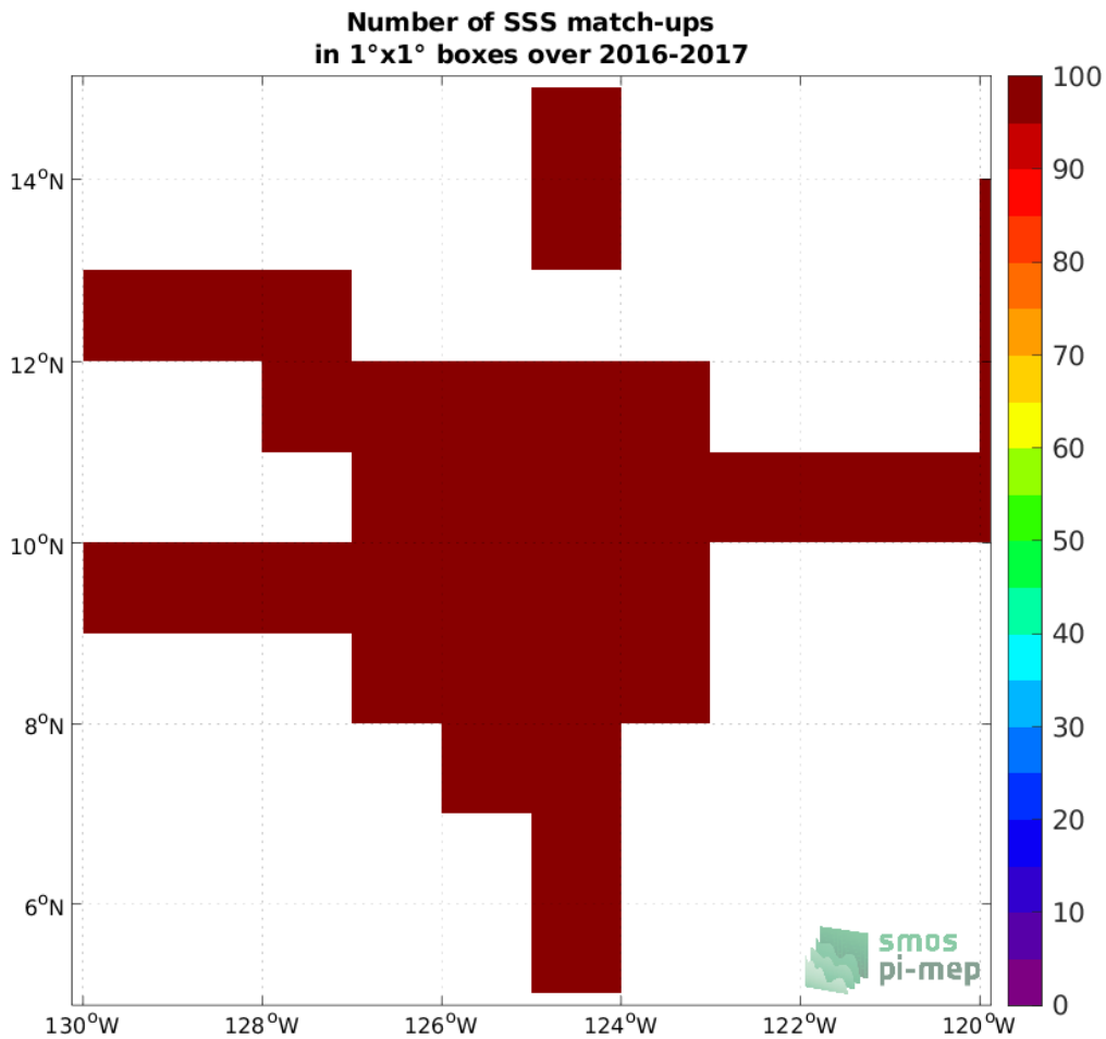
Figure 4: Number of SSS match-ups between Salinity Snake (SPURS 2) SSS and the SMOS SSS L3 v332 - 9 Days (CATDS-CPDC) SSS product for the SPURS 2 Pi-MEP region over 1°x1° boxes and for the full satellite product period.
