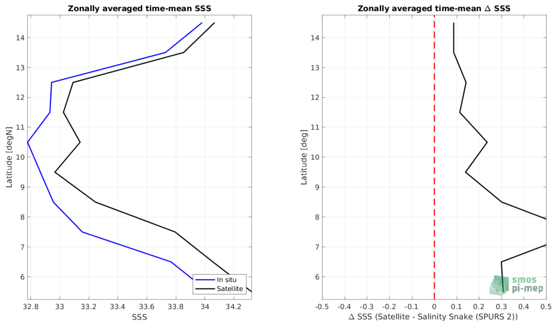
Figure 8: Left panel: Zonal mean SSS from SMOS SSS L3 v332 - 9 Days (CATDS-CPDC) satellite product (black) and from Salinity Snake (SPURS 2) (blue). Right panel: Zonal mean of \Delta SSS (Satellite - Salinity Snake (SPURS 2)) for all the collected Pi-MEP match-up pairs estimated over the full satellite product period.
