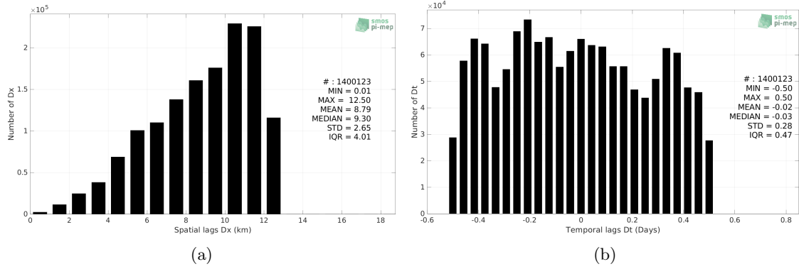
Figure 5: Histograms of the spatial (a) and temporal (b) lags between the location/time of the Salinity Snake (SPURS 2) measurement and the date of the corresponding SMOS SSS L3 v332 - 9 Days (CATDS-CPDC) SSS pixel.
