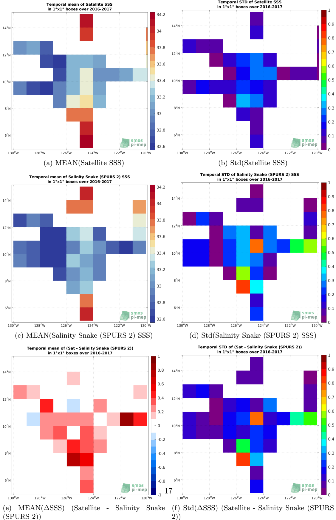
Figure 6: Temporal mean (left) and Std (right) of SSS from SMOS SSS L3 v332 - 9 Days (CATDS-CPDC) (top), Salinity Snake (SPURS 2) (middle), and of \Delta SSS (Satellite - Salinity Snake (SPURS 2)). Only match-up pairs are used to generate these maps.
