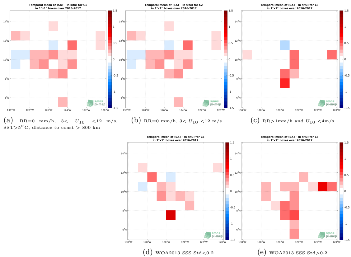
Figure 12: Temporal mean gridded over spatial boxes of size 1^\circ \times 1^\circ of \Delta SSS (SMOS SSS L3 v332 - 9 Days (CATDS-CPDC) - Salinity Snake (SPURS 2)) for 5 different subdatasets corresponding to:RR=0 mm/h, 3 < U_{10} < 12 m/s, SST >5^\circ C, distance to coast > 800 km (a), RR=0 mm/h, 3 < U_{10} < 12 m/s (b), RR >1 mm/h and U_{10} < 4 m/s (c), WOA2013 SSS Std <0.2 (d), WOA2013 SSS Std >0.2 (e).
