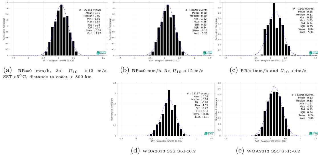
Figure 15: Normalized histogram of \Delta SSS (SMOS SSS L3 v332 - 9 Days (CATDS-CPDC) - Seaglider (SPURS 2)) for 5 different subdatasets corresponding to: RR=0 mm/h, 3 < U_{10} < 12 m/s, SST>5°C, distance to coast > 800 km (a), RR=0 mm/h, 3 < U_{10} < 12 m/s (b), RR>1mm/h and U_{10} < 4 m/s (c), WOA2013 SSS Std<0.2 (d), WOA2013 SSS Std>0.2 (e).
