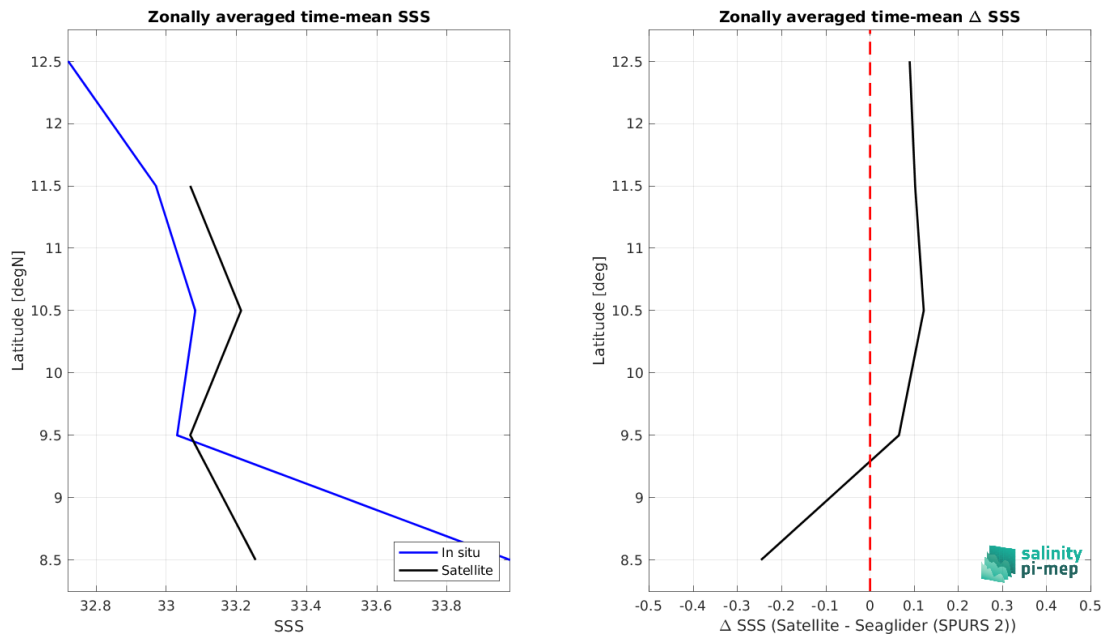
Figure 9: Left panel: Zonal mean SSS from SMOS SSS L3 v332 - 9 Days (CATDS-CPDC) satellite product (black) and from Seaglider (SPURS 2) (blue). Right panel: Zonal mean of \Delta SSS (Satellite - Seaglider (SPURS 2)) for all the collected Pi-MEP match-up pairs estimated over the full satellite product period.
