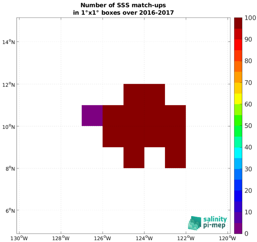
Figure 5: Number of SSS match-ups between Seagliders (SPURS 2) SSS and the SMOS SSS L3 v332 - 9 Days (CATDS-CPDC) SSS product for the SPURS 2 Pi-MEP region over 1^\circ \times 1^\circ boxes and for the full satellite product period.
