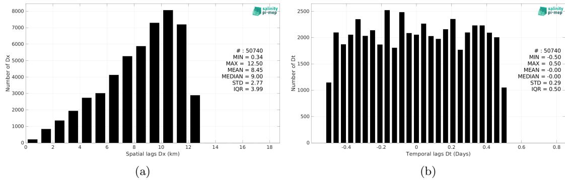
Figure 6: Histograms of the spatial (a) and temporal (b) lags between the location/time of the Seaglider (SPURS 2) measurement and the date of the corresponding SMOS SSS L3 v332 - 9 Days (CATDS-CPDC) SSS pixel.
