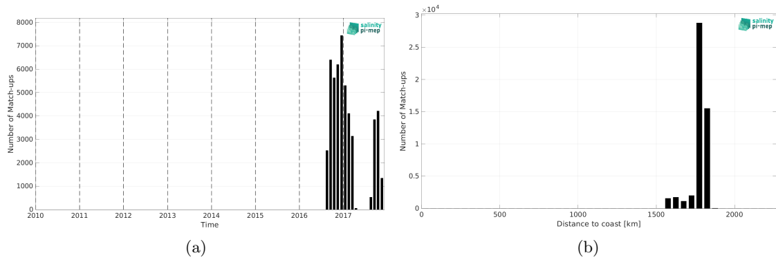
Figure 2: Number of match-ups between Seaglider (SPURS 2) and SMOS SSS L3 v332 - 9 Days (CATDS-CPDC) SSS as a function of time (a) and as function of the distance to coast (b) over the SPURS 2 Pi-MEP region and for the full satellite product period.
