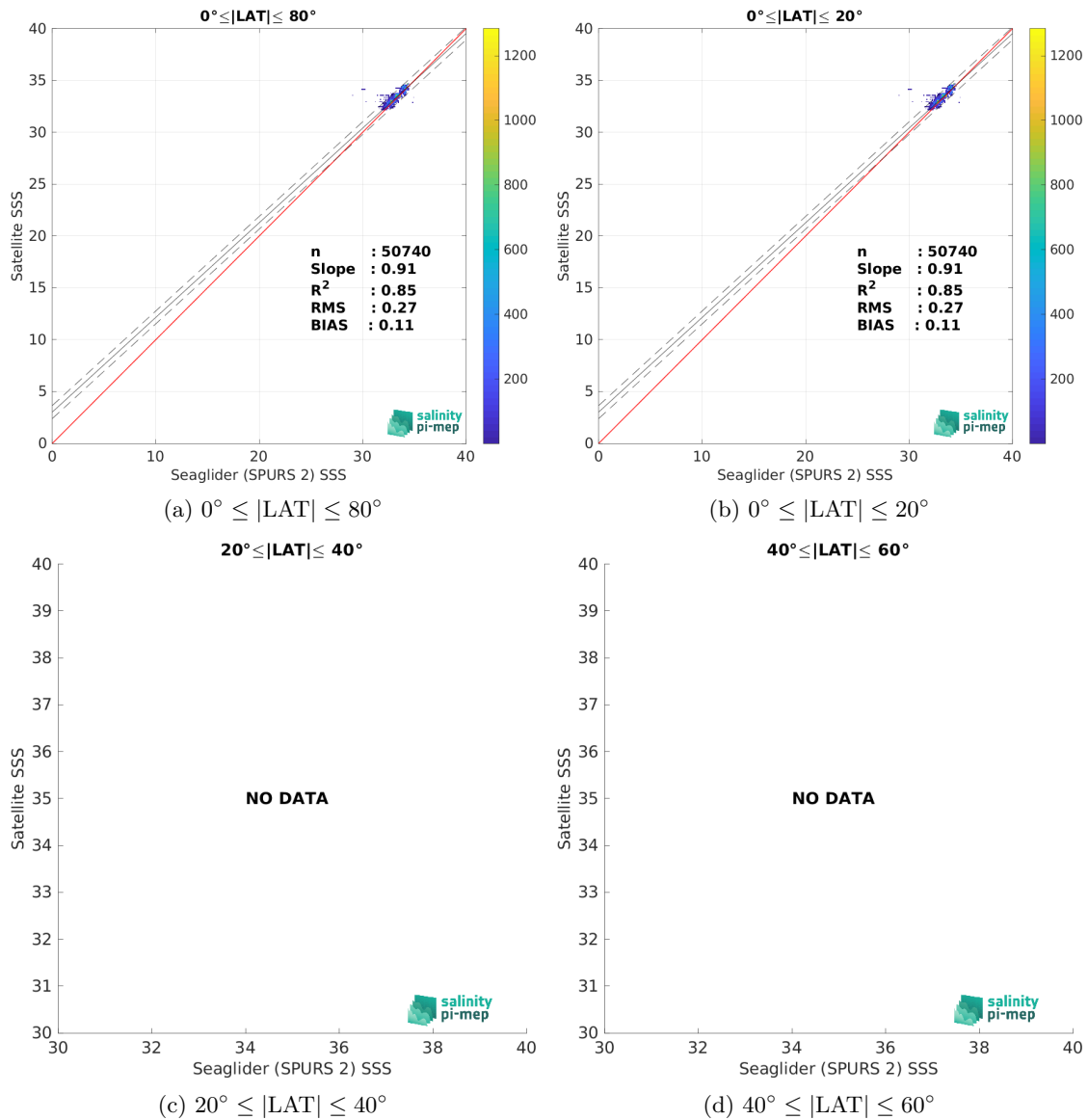
Figure 10: Contour maps of the concentration of SMOS SSS L3 v332 - 9 Days (CATDS-CPDC) SSS (y-axis) versus Seaglider (SPURS 2) SSS (x-axis) at match-up pairs for different latitude bands. For each plot, the red line shows x=y . The black thin and dashed lines indicate a linear fit through the data cloud and the \pm 95\% confidence levels, respectively. The number match-up pairs n , the slope and R^2 coefficient of the linear fit, the root mean square (RMS) and the mean bias between satellite and in situ data are indicated for each latitude band in each plots.
