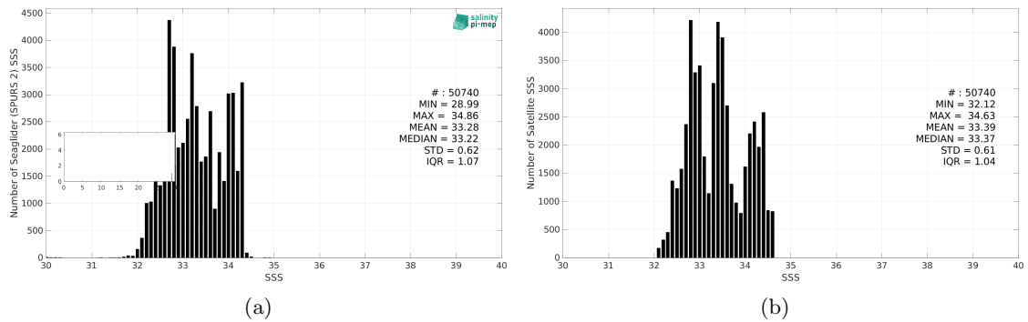
Figure 3: Histograms of SSS from Seaglider (SPURS 2) (a) and SMOS SSS L3 v332 - 9 Days (CATDS-CPDC) (b) considering all match-up pairs per bins of 0.1 over the SPURS 2 Pi-MEP region and for the full satellite product period.
