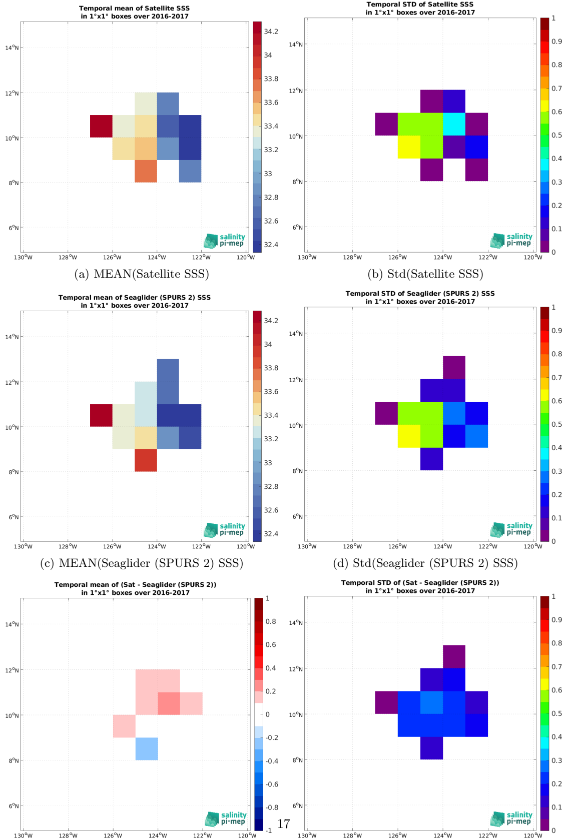
Figure 7: Temporal mean (left) and Std (right) of SSS from SMOS SSS L3 v332 - 9 Days (CATDS-CPDC) (top), Seaglider (SPURS 2) (middle), and of \Delta SSS (Satellite - Seaglider (SPURS 2)). Only match-up pairs are used to generate these maps.
