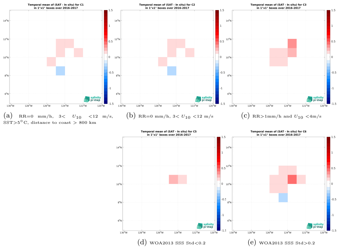
Figure 14: Temporal mean gridded over spatial boxes of size 1^\circ \times 1^\circ of \Delta\text{SSS} (SMOS SSS L3 v332 - 9 Days (CATDS-CPDC) - Seaglider (SPURS 2)) for 5 different subdatasets corresponding to:RR=0 mm/h, 3 < U_{10} < 12 m/s, SST>5°C, distance to coast > 800 km (a), RR=0 mm/h, 3 < U_{10} < 12 m/s (b), RR>1mm/h and U_{10} < 4 m/s (c), WOA2013 SSS Std<0.2 (d), WOA2013 SSS Std>0.2 (e).
