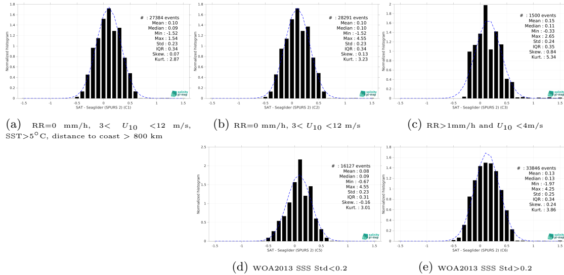
Figure 15: Normalized histogram of \Delta\text{SSS} (SMOS SSS L3 v332 - 9 Days (CATDS-CPDC) - Seaglider (SPURS 2)) for 5 different subdatasets corresponding to: RR=0 mm/h, 3 < U_{10} < 12 m/s, SST>5°C, distance to coast > 800 km (a), RR=0 mm/h, 3 < U_{10} < 12 m/s (b), RR>1mm/h and U_{10} < 4 m/s (c), WOA2013 SSS Std<0.2 (d), WOA2013 SSS Std>0.2 (e).
