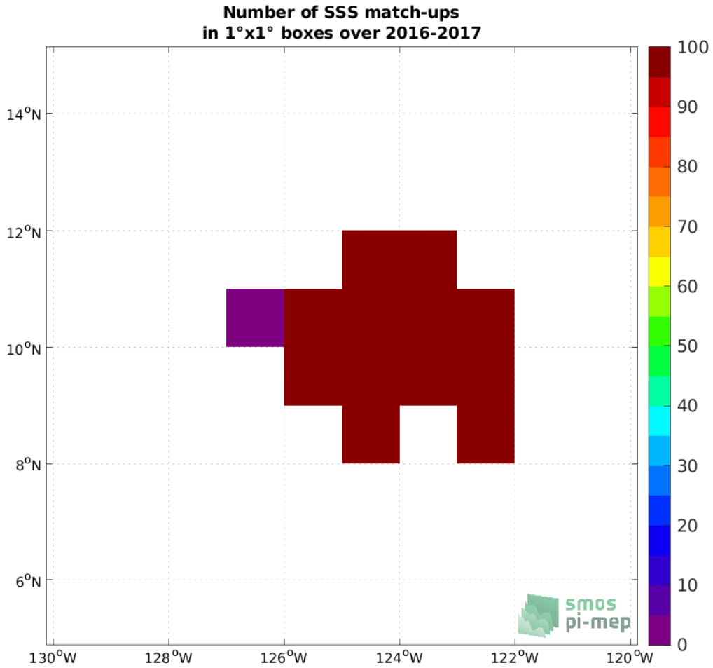
Figure 4: Number of SSS match-ups between Seagliders (SPURS 2) SSS and the SMOS SSS L3 v332 - 9 Days (CATDS-CPDC) SSS product for the SPURS 2 Pi-MEP region over 1°x1° boxes and for the full satellite product period.
