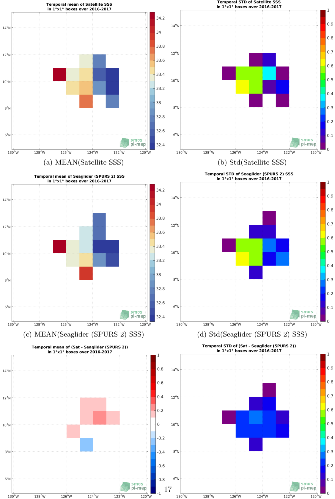
(e) MEAN( \Delta SSS) (Satellite - Seaglider (SPURS 2)) (f) Std( \Delta SSS) (Satellite - Seaglider (SPURS 2)) Figure 6: Temporal mean (left) and Std (right) of SSS from SMOS SSS L3 v332 - 9 Days (CATDS-CPDC) (top), Seaglider (SPURS 2) (middle), and of \Delta SSS (Satellite - Seaglider (SPURS 2)). Only match-up pairs are used to generate these maps.
