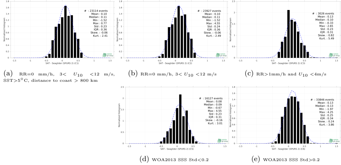
Figure 13: Normalized histogram of \Delta SSS (SMOS SSS L3 v332 - 9 Days (CATDS-CPDC) - Seaglider (SPURS 2)) for 5 different subdatasets corresponding to: RR=0 mm/h, 3 < U_{10} < 12 m/s, SST > 5°C, distance to coast > 800 km (a), RR=0 mm/h, 3 < U_{10} < 12 m/s (b), RR > 1mm/h and U_{10} < 4 m/s (c), WOA2013 SSS Std < 0.2 (d), WOA2013 SSS Std > 0.2 (e).
