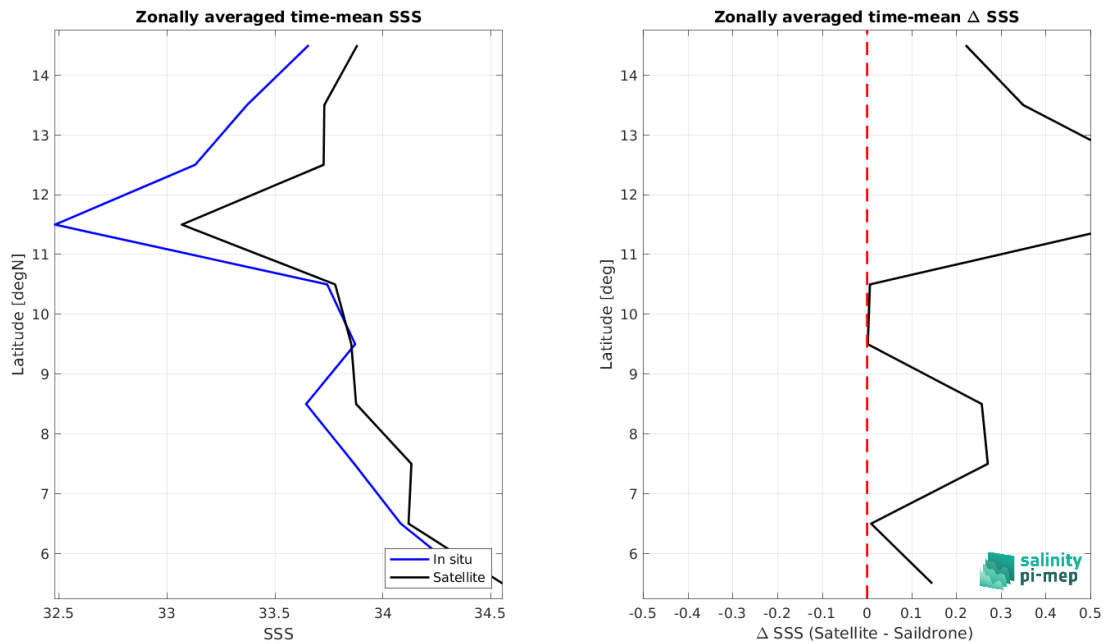
Figure 9: Left panel: Zonal mean SSS from SMOS SSS L3 v332 - 9 Days (CATDS-CPDC) satellite product (black) and from Sairdron (blue). Right panel: Zonal mean of \Delta SSS (Satellite - Sairdron) for all the collected Pi-MEP match-up pairs estimated over the full satellite product period.
