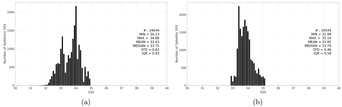
Figure 3: Histograms of SSS from Saildrone (a) and SMOS SSS L3 v332 - 9 Days (CATDS-CPDC) (b) considering all match-up pairs per bins of 0.1 over the SPURS 2 Pi-MEP region and for the full satellite product period.
