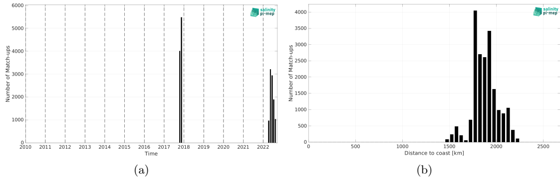
Figure 2: Number of match-ups between Saildrone and SMOS SSS L3 v332 - 9 Days (CATDS-CPDC) SSS as a function of time (a) and as function of the distance to coast (b) over the SPURS 2 Pi-MEP region and for the full satellite product period.
