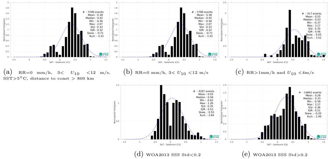
Figure 15: Normalized histogram of \Delta SSS (SMOS SSS L3 v332 - 9 Days (CATDS-CPDC) - Saildrone) for 5 different subdatasets corresponding to: RR=0 mm/h, 3 < U_{10} < 12 m/s, SST>5°C, distance to coast > 800 km (a), RR=0 mm/h, 3 < U_{10} < 12 m/s (b), RR>1mm/h and U_{10} < 4 m/s (c), WOA2013 SSS Std<0.2 (d), WOA2013 SSS Std>0.2 (e).
