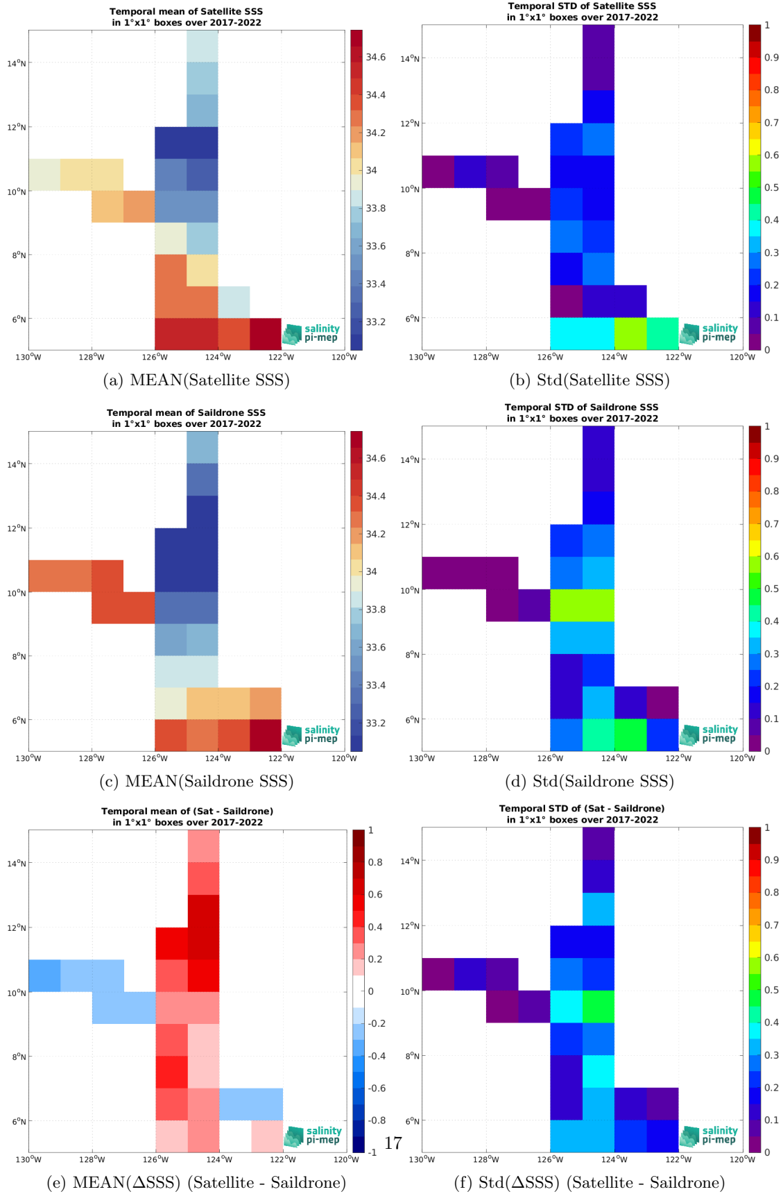
Figure 7: Temporal mean (left) and Std (right) of SSS from SMOS SSS L3 v332 - 9 Days (CATDS-CPDC) (top), Saildrone (middle), and of \Delta SSS (Satellite - Saildrone). Only match-up pairs are used to generate these maps.
