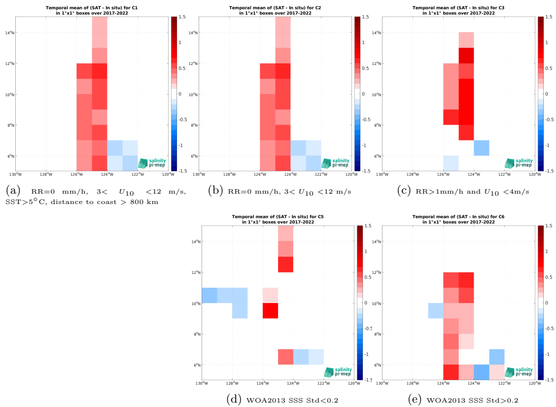
Figure 14: Temporal mean gridded over spatial boxes of size 1^\circ \times 1^\circ of \Delta\text{SSS} (SMOS SSS L3 v332 - 9 Days (CATDS-CPDC) - Sairdrone) for 5 different subdatasets corresponding to:RR=0 mm/h, 3 < U_{10} < 12 m/s, SST>5°C, distance to coast > 800 km (a), RR=0 mm/h, 3 < U_{10} < 12 m/s (b), RR>1mm/h and U_{10} < 4 m/s (c), WOA2013 SSS Std<0.2 (d), WOA2013 SSS Std>0.2 (e).
