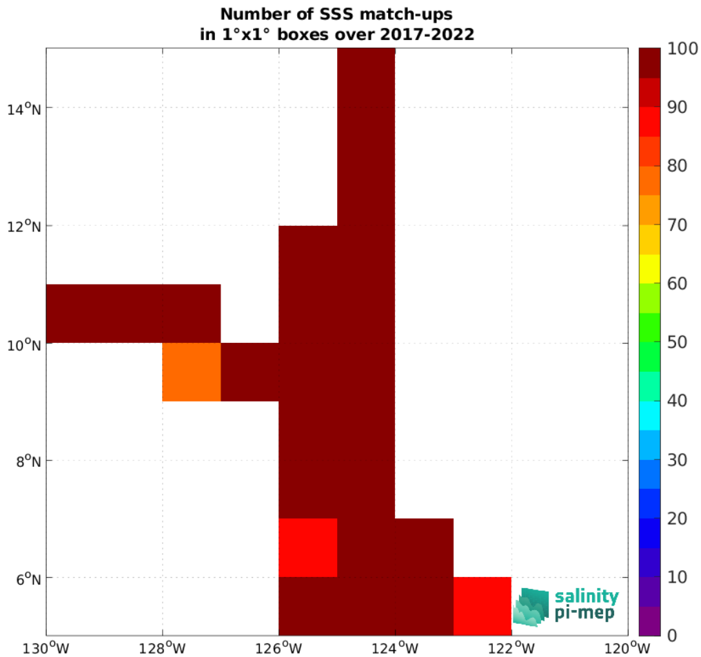
Figure 5: Number of SSS match-ups between Saildrone SSS and the SMOS SSS L3 v332 - 9 Days (CATDS-CPDC) SSS product for the SPURS 2 Pi-MEP region over 1°x1° boxes and for the full satellite product period.
