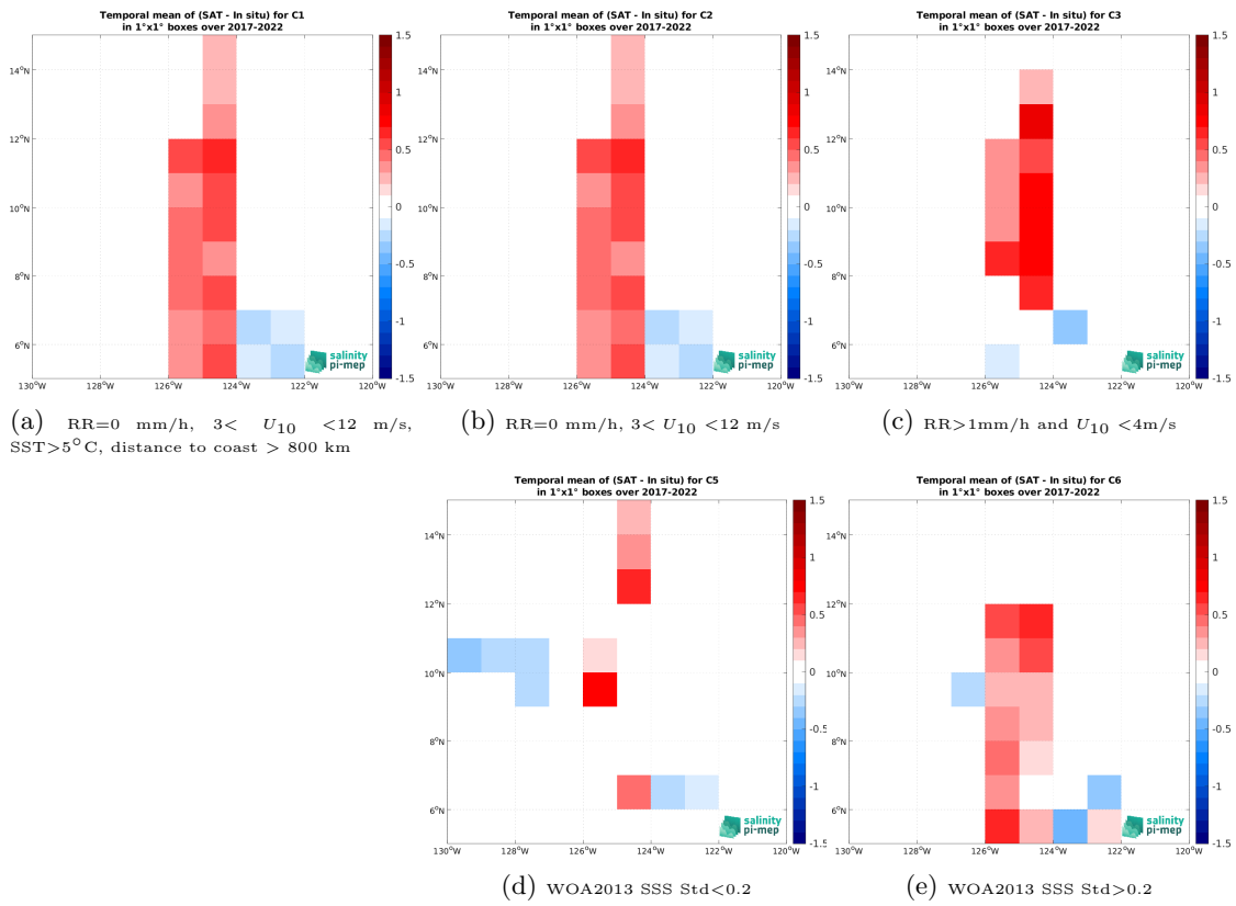
Figure 14: Temporal mean gridded over spatial boxes of size 1^\circ \times 1^\circ of \Delta SSS (SMOS SSS L3 v332 - 9 Days (CATDS-CPDC) - Sairdrone) for 5 different subdatasets corresponding to:RR=0 mm/h, 3 < U_{10} < 12 m/s, SST>5°C, distance to coast > 800 km (a), RR=0 mm/h, 3 < U_{10} < 12 m/s (b), RR>1mm/h and U_{10} < 4 m/s (c), WOA2013 SSS Std<0.2 (d), WOA2013 SSS Std>0.2 (e).
