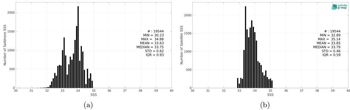
Figure 2: Histograms of SSS from Saildrone (a) and SMOS SSS L3 v332 - 9 Days (CATDS-CPDC) (b) considering all match-up pairs per bins of 0.1 over the SPURS 2 Pi-MEP region and for the full satellite product period.
