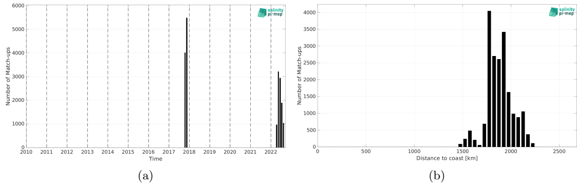
Figure 1: Number of match-ups between Saildrone and SMOS SSS L3 v332 - 9 Days (CATDS-CPDC) SSS as a function of time (a) and as function of the distance to coast (b) over the SPURS 2 Pi-MEP region and for the full satellite product period.
