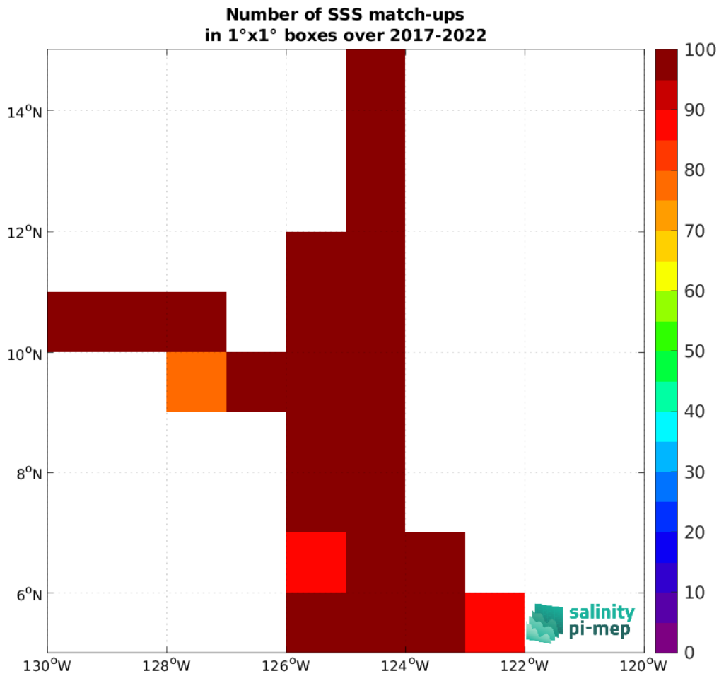
Figure 4: Number of SSS match-ups between Saildrone SSS and the SMOS SSS L3 v332 - 9 Days (CATDS-CPDC) SSS product for the SPURS 2 Pi-MEP region over 1°x1° boxes and for the full satellite product period.
