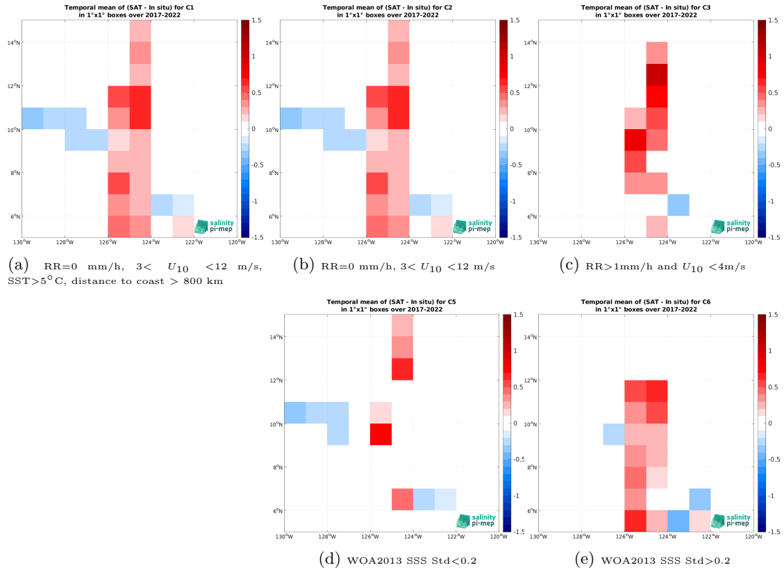
Figure 12: Temporal mean gridded over spatial boxes of size 1^\circ \times 1^\circ of \Delta\text{SSS} (SMOS SSS L3 v332 - 9 Days (CATDS-CPDC) - Sairdrone) for 5 different subdatasets corresponding to:RR=0 mm/h, 3 < U_{10} < 12 m/s, SST >5^\circ\text{C} , distance to coast > 800 km (a), RR=0 mm/h, 3 < U_{10} < 12 m/s (b), RR >1 mm/h and U_{10} < 4 m/s (c), WOA2013 SSS Std <0.2 (d), WOA2013 SSS Std >0.2 (e).
