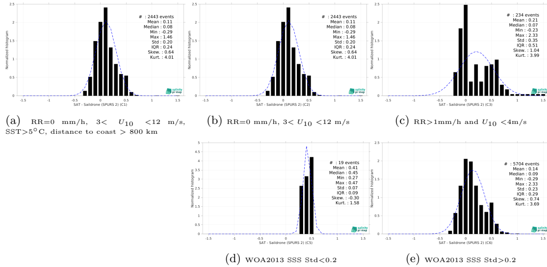
Figure 15: Normalized histogram of \Delta SSS (SMOS SSS L3 v332 - 9 Days (CATDS-CPDC) - Saildrone (SPURS 2)) for 5 different subdatasets corresponding to: RR=0 mm/h, 3 < U_{10} < 12 m/s, SST > 5°C, distance to coast > 800 km (a), RR=0 mm/h, 3 < U_{10} < 12 m/s (b), RR > 1mm/h and U_{10} < 4 m/s (c), WOA2013 SSS Std < 0.2 (d), WOA2013 SSS Std > 0.2 (e).
