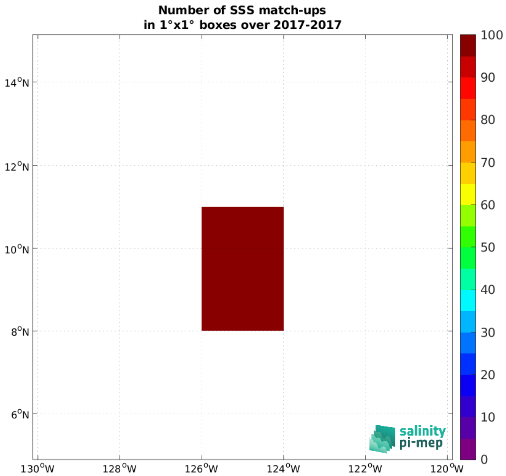
Figure 5: Number of SSS match-ups between Saildrone (SPURS 2) SSS and the SMOS SSS L3 v332 - 9 Days (CATDS-CPDC) SSS product for the SPURS 2 Pi-MEP region over 1^\circ \times 1^\circ boxes and for the full satellite product period.
