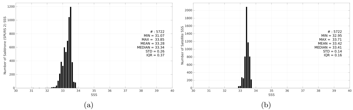
Figure 3: Histograms of SSS from Saildrone (SPURS 2) (a) and SMOS SSS L3 v332 - 9 Days (CATDS-CPDC) (b) considering all match-up pairs per bins of 0.1 over the SPURS 2 Pi-MEP region and for the full satellite product period.
