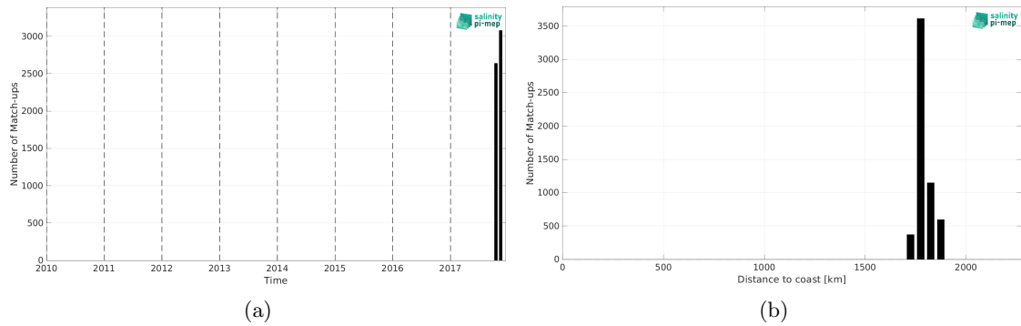
Figure 2: Number of match-ups between Saildrone (SPURS 2) and SMOS SSS L3 v332 - 9 Days (CATDS-CPDC) SSS as a function of time (a) and as function of the distance to coast (b) over the SPURS 2 Pi-MEP region and for the full satellite product period.
