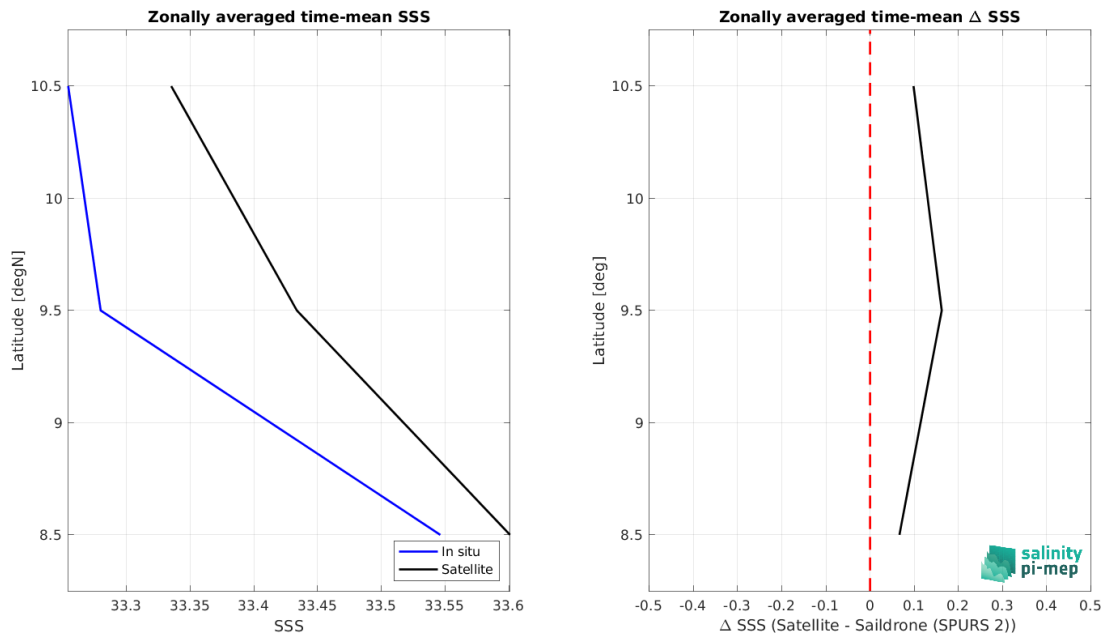
Figure 9: Left panel: Zonal mean SSS from SMOS SSS L3 v332 - 9 Days (CATDS-CPDC) satellite product (black) and from Sairdron (SPURS 2) (blue). Right panel: Zonal mean of \Delta SSS (Satellite - Sairdron (SPURS 2)) for all the collected Pi-MEP match-up pairs estimated over the full satellite product period.
