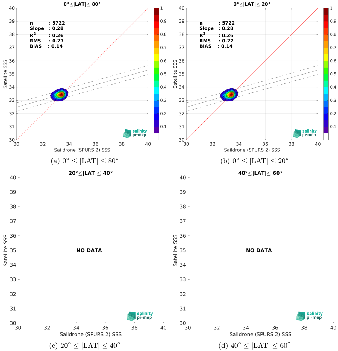
Figure 10: Contour maps of the concentration of SMOS SSS L3 v332 - 9 Days (CATDS-CPDC) SSS (y-axis) versus Saildrone (SPURS 2) SSS (x-axis) at match-up pairs for different latitude bands. For each plot, the red line shows x=y . The black thin and dashed lines indicate a linear fit through the data cloud and the \pm 95\% confidence levels, respectively. The number match-up pairs n , the slope and R^2 coefficient of the linear fit, the root mean square (RMS) and the mean bias between satellite and in situ data are indicated for each latitude band in each plots.
