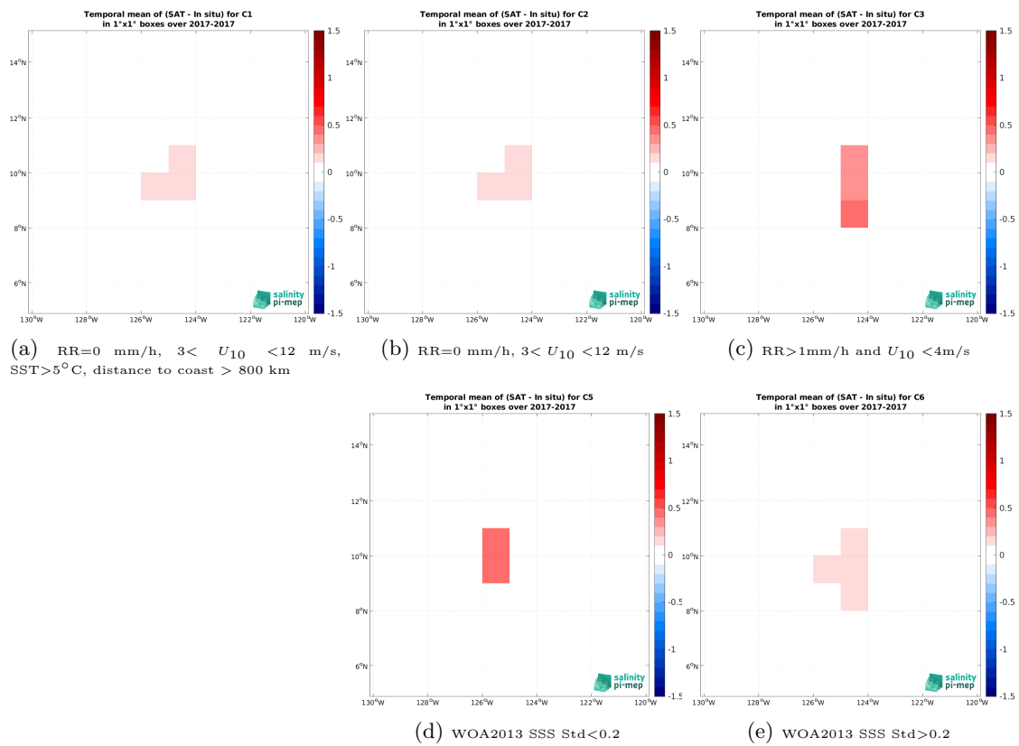
Figure 14: Temporal mean gridded over spatial boxes of size 1^\circ \times 1^\circ of \Delta SSS (SMOS SSS L3 v332 - 9 Days (CATDS-CPDC) - Saildrone (SPURS 2)) for 5 different subdatasets corresponding to:RR=0 mm/h, 3 < U_{10} < 12 m/s, SST >5^\circ C, distance to coast > 800 km (a), RR=0 mm/h, 3 < U_{10} < 12 m/s (b), RR >1 mm/h and U_{10} < 4 m/s (c), WOA2013 SSS Std <0.2 (d), WOA2013 SSS Std >0.2 (e).
