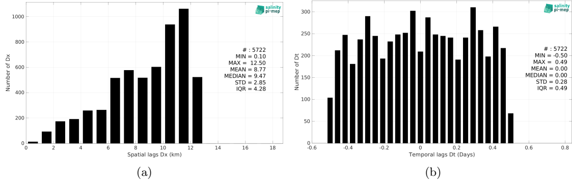
Figure 6: Histograms of the spatial (a) and temporal (b) lags between the location/time of the Saildrone (SPURS 2) measurement and the date of the corresponding SMOS SSS L3 v332 - 9 Days (CATDS-CPDC) SSS pixel.
