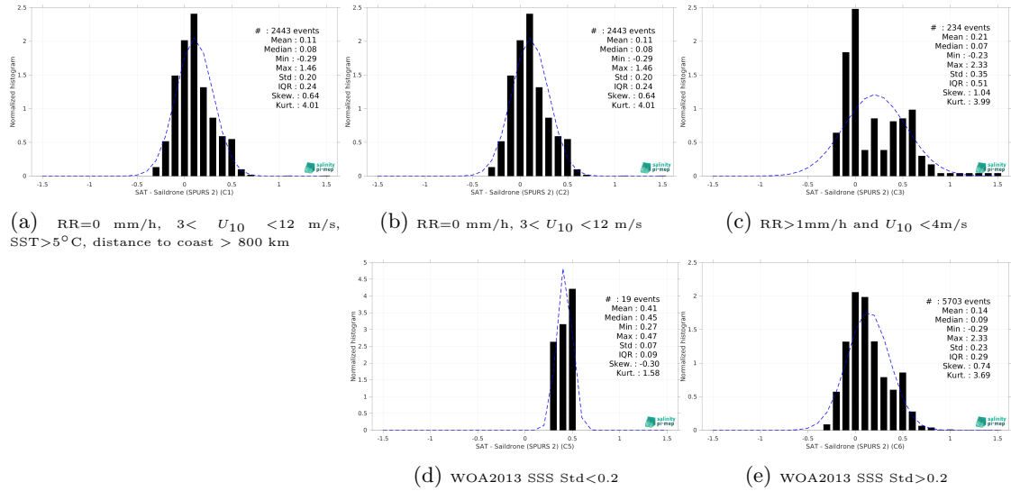
Figure 15: Normalized histogram of \Delta SSS (SMOS SSS L3 v332 - 9 Days (CATDS-CPDC) - Saildrone (SPURS 2)) for 5 different subdatasets corresponding to: RR=0 mm/h, 3 < U_{10} < 12 m/s, SST>5°C, distance to coast > 800 km (a), RR=0 mm/h, 3 < U_{10} < 12 m/s (b), RR>1mm/h and U_{10} < 4 m/s (c), WOA2013 SSS Std<0.2 (d), WOA2013 SSS Std>0.2 (e).
