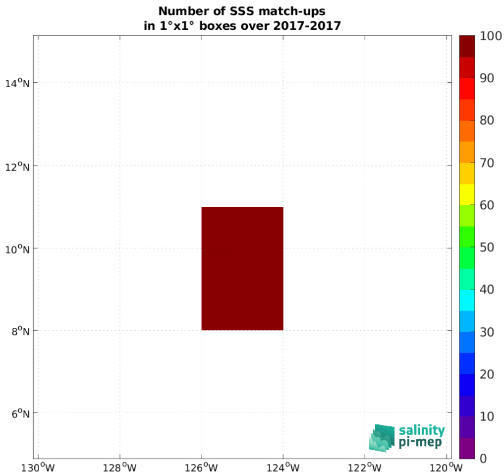
Figure 4: Number of SSS match-ups between Saildrone (SPURS 2) SSS and the SMOS SSS L3 v332 - 9 Days (CATDS-CPDC) SSS product for the SPURS 2 Pi-MEP region over 1°x1° boxes and for the full satellite product period.
