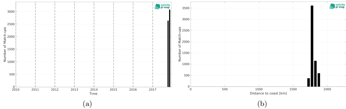
Figure 1: Number of match-ups between Saildrone (SPURS 2) and SMOS SSS L3 v332 - 9 Days (CATDS-CPDC) SSS as a function of time (a) and as function of the distance to coast (b) over the SPURS 2 Pi-MEP region and for the full satellite product period.
