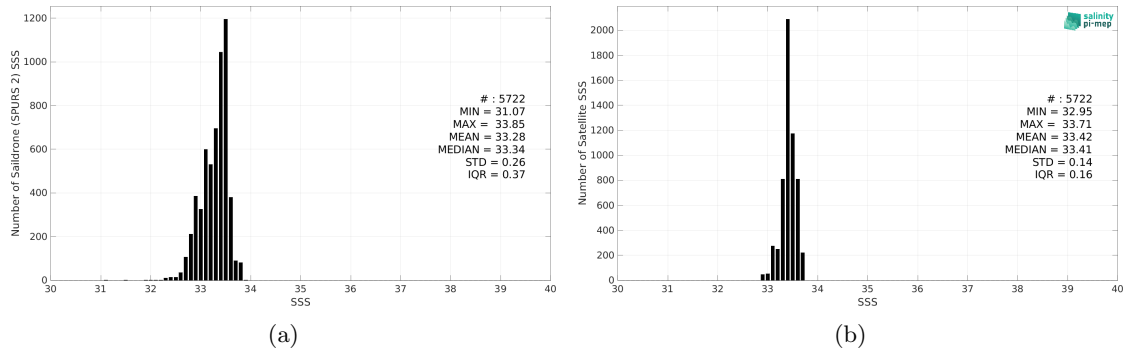
Figure 2: Histograms of SSS from Saildrone (SPURS 2) (a) and SMOS SSS L3 v332 - 9 Days (CATDS-CPDC) (b) considering all match-up pairs per bins of 0.1 over the SPURS 2 Pi-MEP region and for the full satellite product period.
