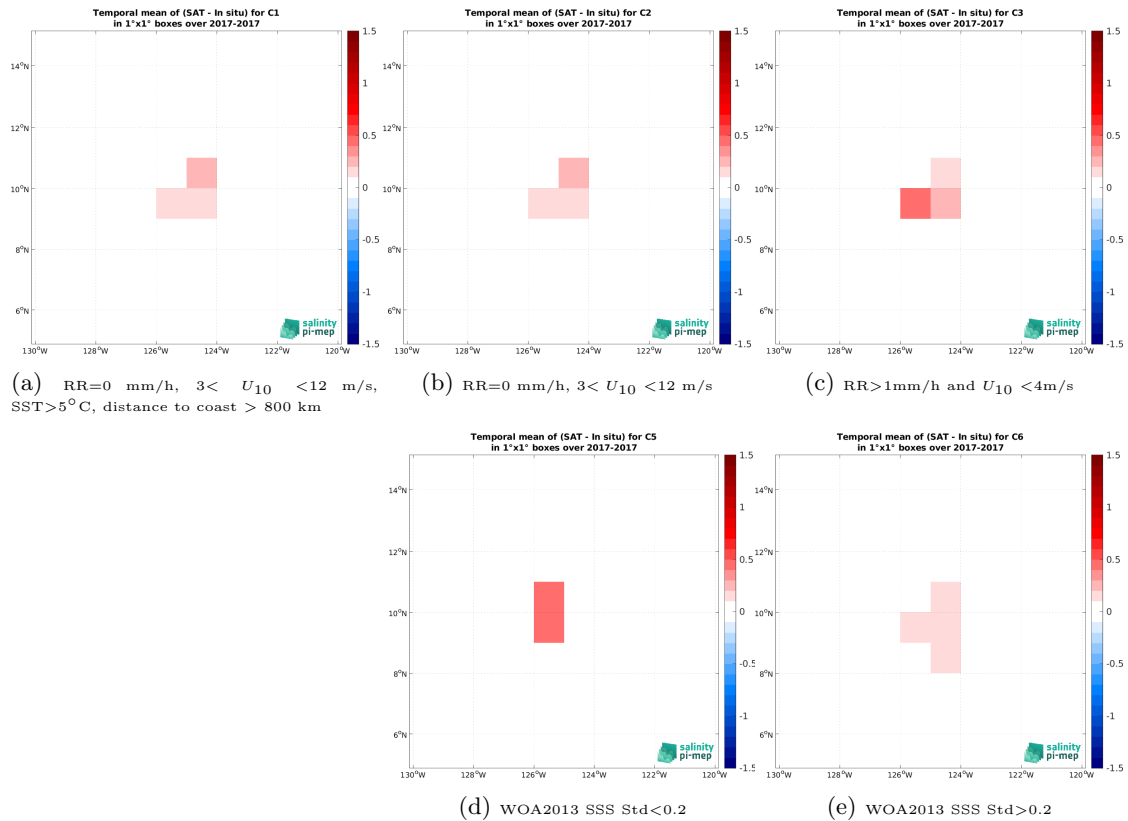
Figure 12: Temporal mean gridded over spatial boxes of size 1^\circ \times 1^\circ of \Delta SSS (SMOS SSS L3 v332 - 9 Days (CATDS-CPDC) - Saildrone (SPURS 2)) for 5 different subdatasets corresponding to:RR=0 mm/h, 3 < U_{10} < 12 m/s, SST >5^\circ C, distance to coast > 800 km (a), RR=0 mm/h, 3 < U_{10} < 12 m/s (b), RR >1 mm/h and U_{10} < 4 m/s (c), WOA2013 SSS Std <0.2 (d), WOA2013 SSS Std >0.2 (e).
