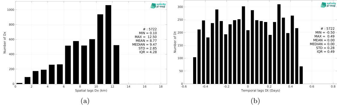
Figure 5: Histograms of the spatial (a) and temporal (b) lags between the location/time of the Saildrone (SPURS 2) measurement and the date of the corresponding SMOS SSS L3 v332 - 9 Days (CATDS-CPDC) SSS pixel.
