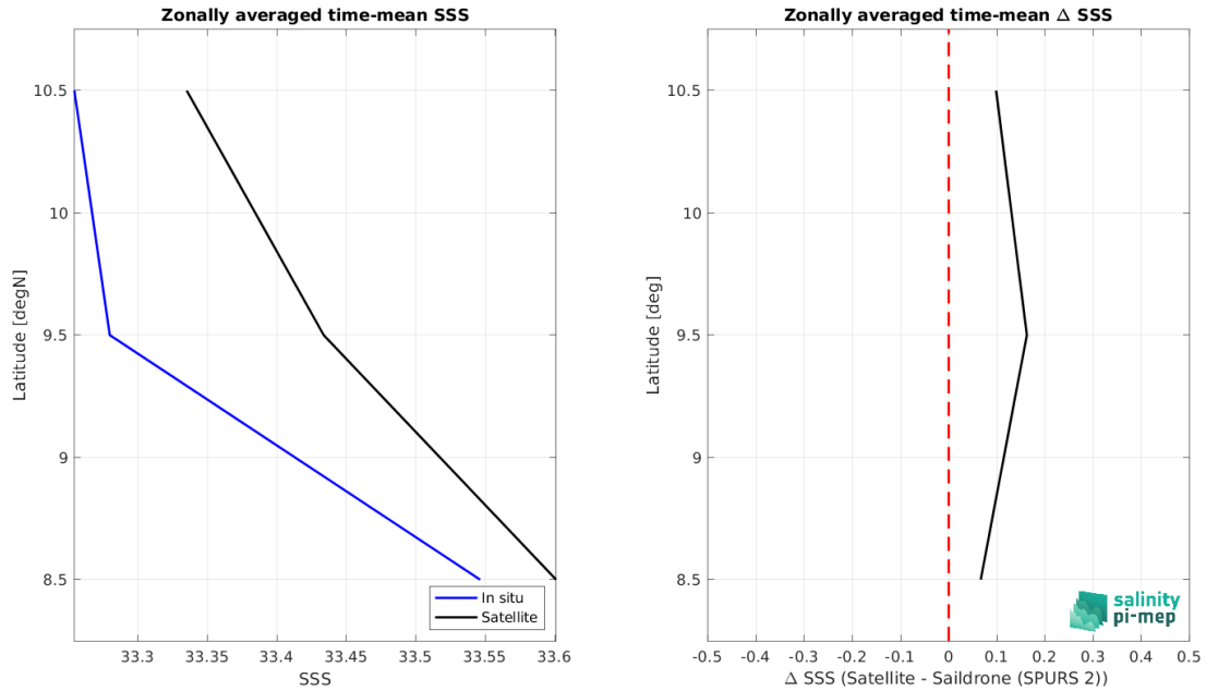
Figure 8: Left panel: Zonal mean SSS from SMOS SSS L3 v332 - 9 Days (CATDS-CPDC) satellite product (black) and from Sairdron (SPURS 2) (blue). Right panel: Zonal mean of \Delta SSS (Satellite - Sairdron (SPURS 2)) for all the collected Pi-MEP match-up pairs estimated over the full satellite product period.
