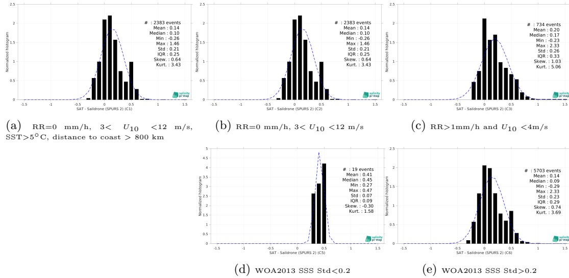
Figure 13: Normalized histogram of \Delta SSS (SMOS SSS L3 v332 - 9 Days (CATDS-CPDC) - Saildrone (SPURS 2)) for 5 different subdatasets corresponding to: RR=0 mm/h, 3 < U_{10} < 12 m/s, SST > 5°C, distance to coast > 800 km (a), RR=0 mm/h, 3 < U_{10} < 12 m/s (b), RR > 1mm/h and U_{10} < 4 m/s (c), WOA2013 SSS Std < 0.2 (d), WOA2013 SSS Std > 0.2 (e).
