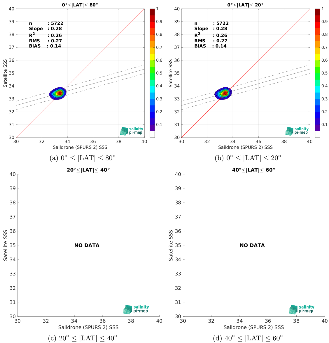
Figure 9: Contour maps of the concentration of SMOS SSS L3 v332 - 9 Days (CATDS-CPDC) SSS (y-axis) versus Saildrone (SPURS 2) SSS (x-axis) at match-up pairs for different latitude bands. For each plot, the red line shows x=y . The black thin and dashed lines indicate a linear fit through the data cloud and the \pm 95\% confidence levels, respectively. The number match-up pairs n , the slope and R^2 coefficient of the linear fit, the root mean square (RMS) and the mean bias between satellite and in situ data are indicated for each latitude band in each plots.
