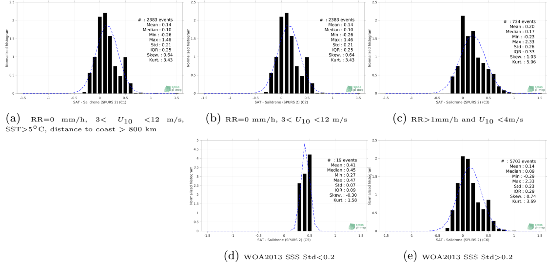
Figure 13: Normalized histogram of \Delta SSS (SMOS SSS L3 v332 - 9 Days (CATDS-CPDC) - Saildrone (SPURS 2)) for 5 different subdatasets corresponding to: RR=0 mm/h, 3 < U_{10} < 12 m/s, SST > 5°C, distance to coast > 800 km (a), RR=0 mm/h, 3 < U_{10} < 12 m/s (b), RR > 1mm/h and U_{10} < 4 m/s (c), WOA2013 SSS Std < 0.2 (d), WOA2013 SSS Std > 0.2 (e).
