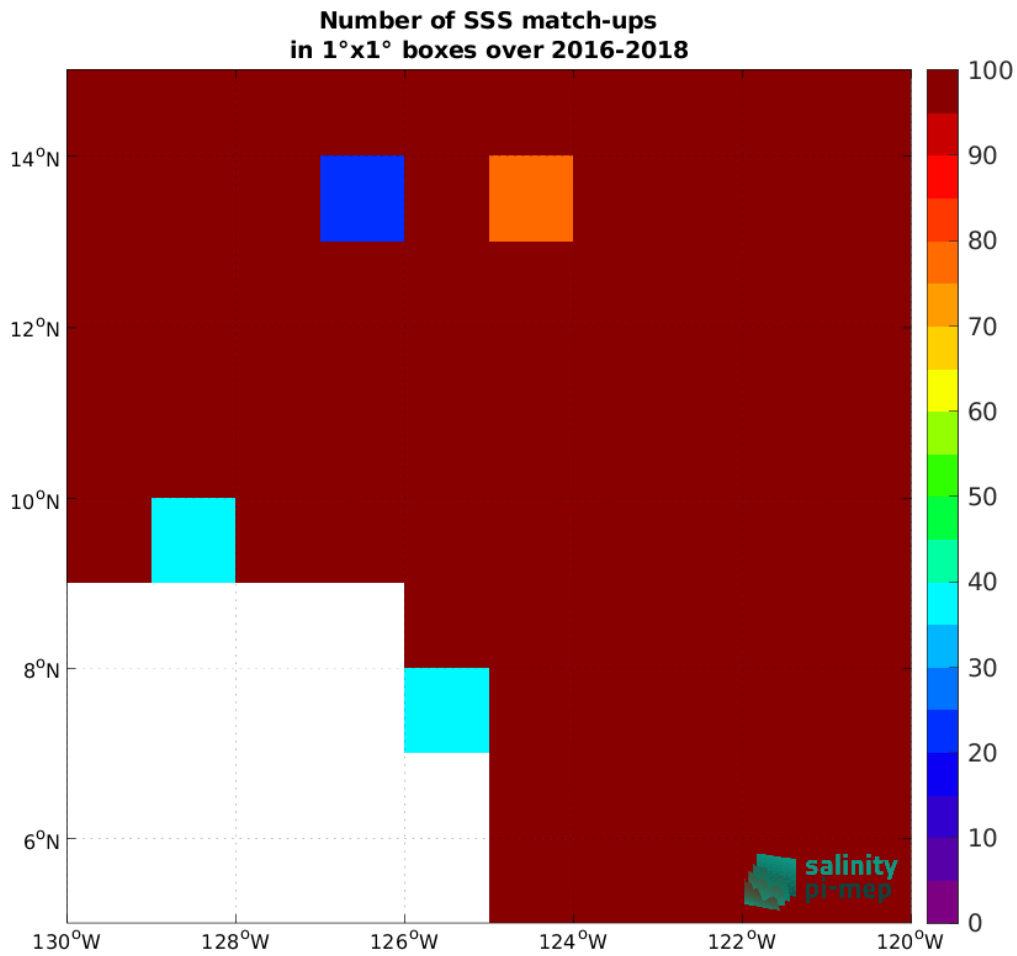
Figure 3: Number of SSS match-ups between Surface drifters SSS and the SMOS SSS L3 v332 - 9 Days (CATDS-CPDC) SSS product for the SPURS 2 Pi-MEP region over 1°x1° boxes and for the full satellite product period.
