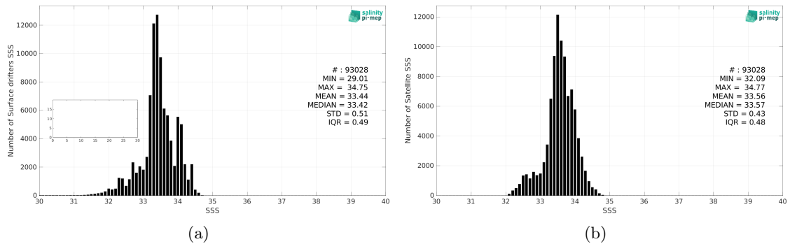
Figure 2: Histograms of SSS from Surface drifters (a) and SMOS SSS L3 v332 - 9 Days (CATDS-CPDC) (b) considering all match-up pairs per bins of 0.1 over the SPURS 2 Pi-MEP region and for the full satellite product period.
