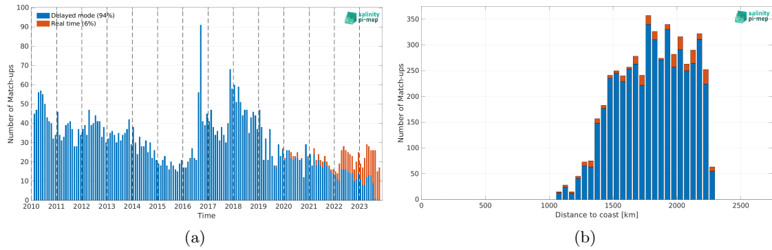
Figure 1: Number of match-ups between Argo and SMOS SSS L3 v332 - 9 Days (CATDS-CPDC) SSS as a function of time (a) and as function of the distance to coast (b) over the SPURS 2 Pi-MEP region and for the full satellite product period.
