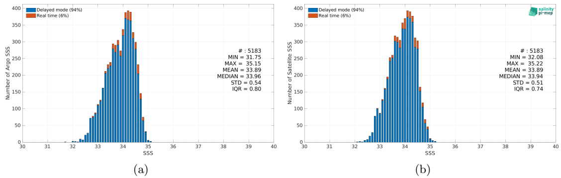
Figure 2: Histograms of SSS from Argo (a) and SMOS SSS L3 v332 - 9 Days (CATDS-CPDC) (b) considering all match-up pairs per bins of 0.1 over the SPURS 2 Pi-MEP region and for the full satellite product period.
