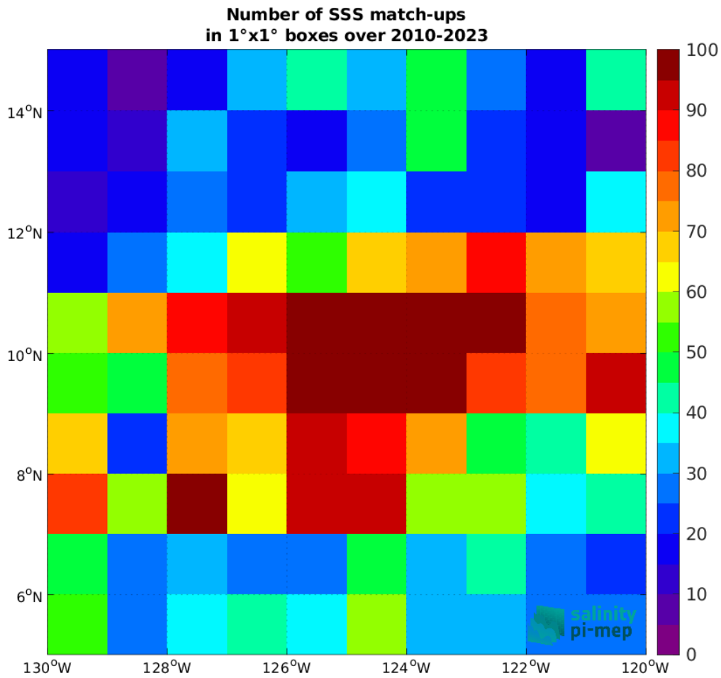
Figure 4: Number of SSS match-ups between Argo SSS and the SMOS SSS L3 v332 - 9 Days (CATDS-CPDC) SSS product for the SPURS 2 Pi-MEP region over 1°x1° boxes and for the full satellite product period.
