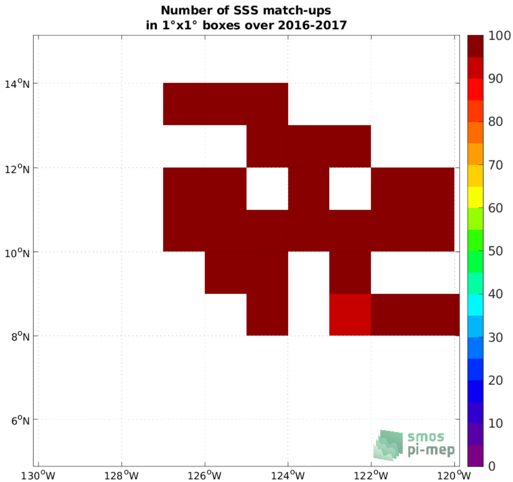
Figure 4: Number of SSS match-ups between Waveglider (SPURS 2) SSS and the SMOS SSS L2Q v331 - 0.25 Deg (CATDS-CPDC) SSS product for the SPURS 2 Pi-MEP region over 1°x1° boxes and for the full satellite product period.
