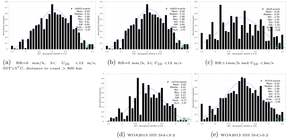
Figure 13: Normalized histogram of \Delta SSS (SMOS SSS L2Q v331 - 0.25 Deg (CATDS-CPDC) - Waveglider (SPURS 2)) for 5 different subdatasets corresponding to: RR=0 mm/h, 3 < U_{10} < 12 m/s, SST>5°C, distance to coast > 800 km (a), RR=0 mm/h, 3 < U_{10} < 12 m/s (b), RR>1mm/h and U_{10} < 4 m/s (c), WOA2013 SSS Std<0.2 (d), WOA2013 SSS Std>0.2 (e).
