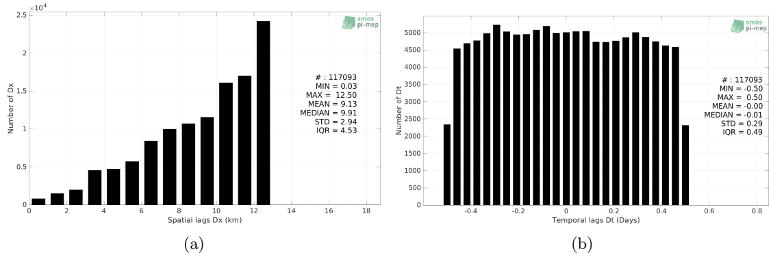
Figure 5: Histograms of the spatial (a) and temporal (b) lags between the location/time of the Waveglider (SPURS 2) measurement and the date of the corresponding SMOS SSS L2Q v331 - 0.25 Deg (CATDS-CPDC) SSS pixel.
