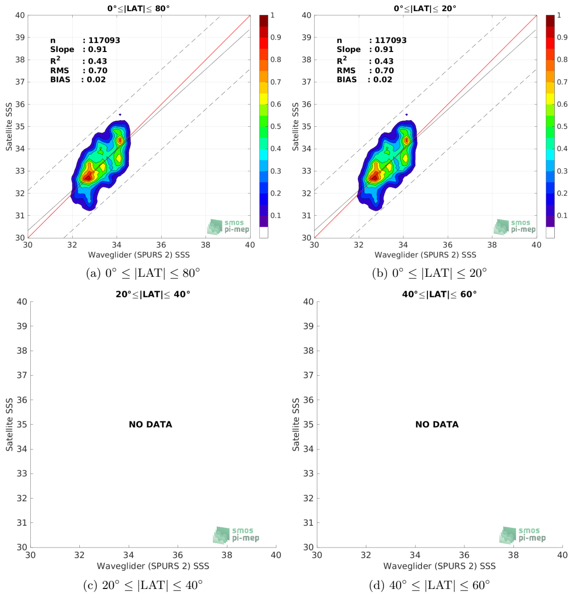
Figure 9: Contour maps of the concentration of SMOS SSS L2Q v331 - 0.25 Deg (CATDS-CPDC) SSS (y-axis) versus Waveglider (SPURS 2) SSS (x-axis) at match-up pairs for different latitude bands. For each plot, the red line shows x=y . The black thin and dashed lines indicate a linear fit through the data cloud and the \pm 95\% confidence levels, respectively. The number match-up pairs n , the slope and R^2 coefficient of the linear fit, the root mean square (RMS) and the mean bias between satellite and in situ data are indicated for each latitude band in each plots.
