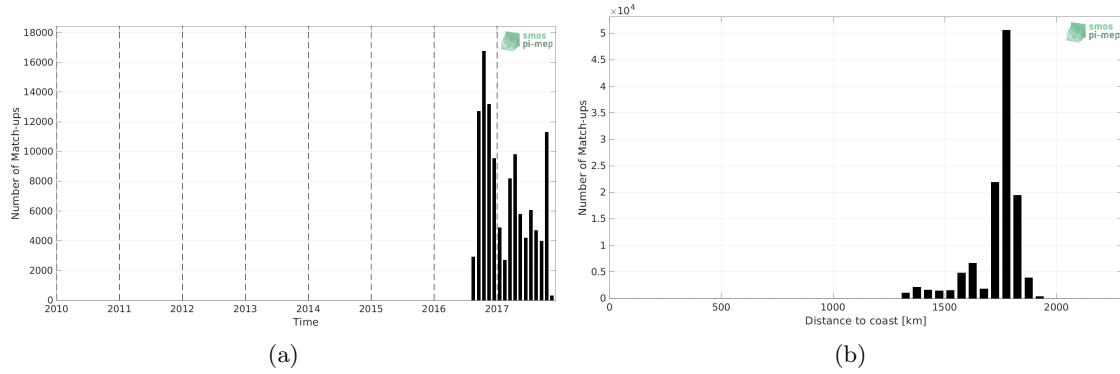
Figure 1: Number of match-ups between Waveglider (SPURS 2) and SMOS SSS L2Q v331 - 0.25 Deg (CATDS-CPDC) SSS as a function of time (a) and as function of the distance to coast (b) over the SPURS 2 Pi-MEP region and for the full satellite product period.
