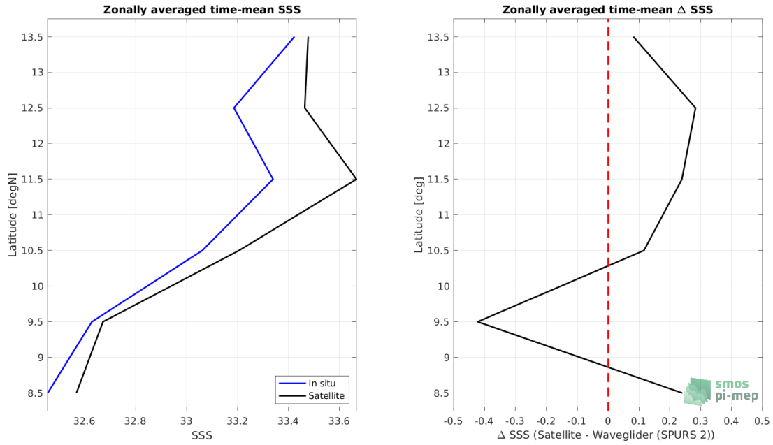
Figure 8: Left panel: Zonal mean SSS from SMOS SSS L2Q v331 - 0.25 Deg (CATDS-CPDC) satellite product (black) and from Waveglider (SPURS 2) (blue). Right panel: Zonal mean of \Delta SSS (Satellite - Waveglider (SPURS 2)) for all the collected Pi-MEP match-up pairs estimated over the full satellite product period.
