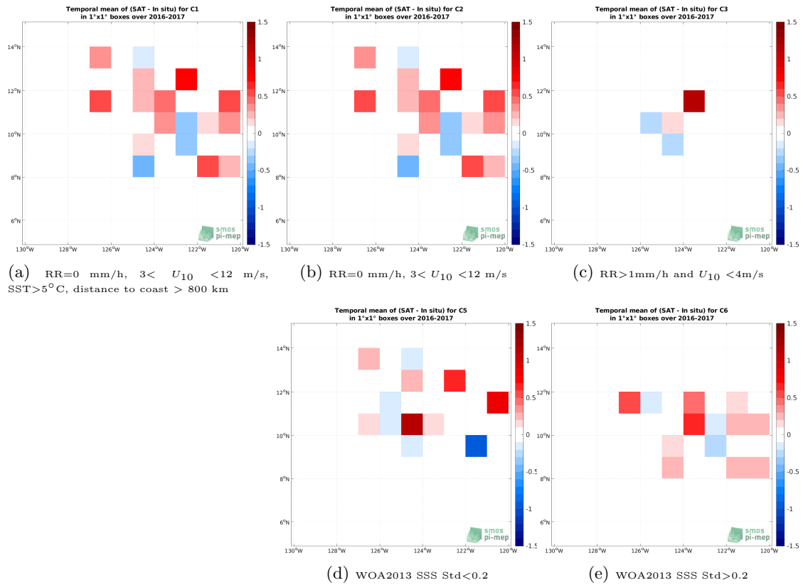
Figure 12: Temporal mean gridded over spatial boxes of size 1^\circ \times 1^\circ of \Delta SSS (SMOS SSS L2Q v331 - 0.25 Deg (CATDS-CPDC) - Waveglider (SPURS 2)) for 5 different subdatasets corresponding to:RR=0 mm/h, 3 < U_{10} < 12 m/s, SST >5^\circ C, distance to coast > 800 km (a), RR=0 mm/h, 3 < U_{10} < 12 m/s (b), RR >1 mm/h and U_{10} < 4 m/s (c), WOA2013 SSS Std <0.2 (d), WOA2013 SSS Std >0.2 (e).
