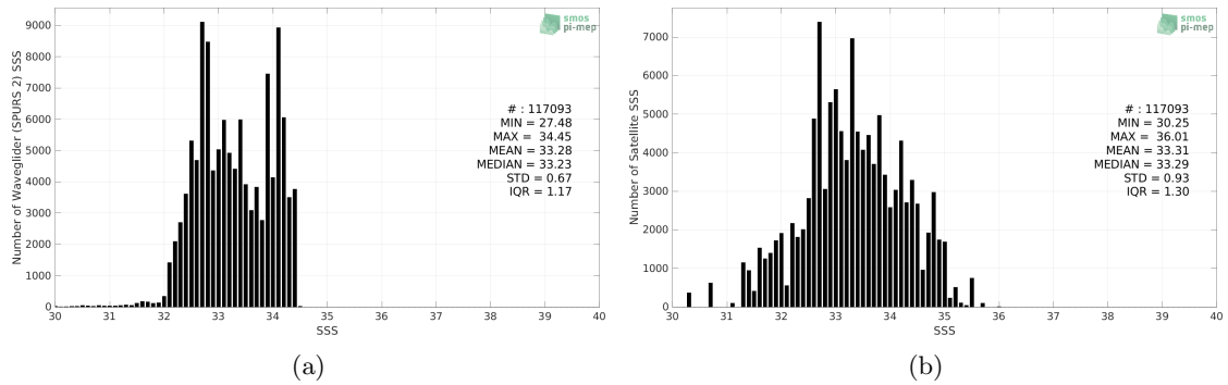
Figure 2: Histograms of SSS from Waveglider (SPURS 2) (a) and SMOS SSS L2Q v331 - 0.25 Deg (CATDS-CPDC) (b) considering all match-up pairs per bins of 0.1 over the SPURS 2 Pi-MEP region and for the full satellite product period.
