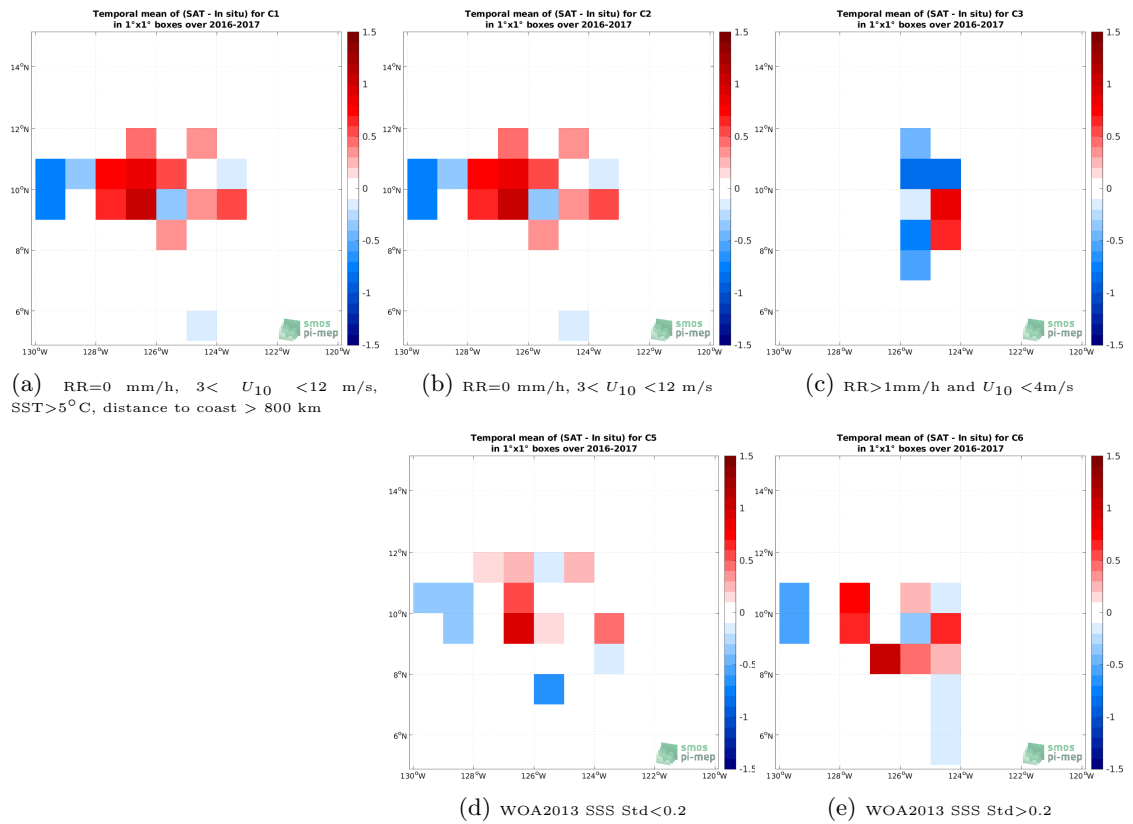
Figure 12: Temporal mean gridded over spatial boxes of size 1^\circ \times 1^\circ of \Delta SSS (SMOS SSS L2Q v331 - 0.25 Deg (CATDS-CPDC) - Salinity Snake (SPURS 2)) for 5 different subdatasets corresponding to:RR=0 mm/h, 3 < U_{10} < 12 m/s, SST >5^\circ C, distance to coast > 800 km (a), RR=0 mm/h, 3 < U_{10} < 12 m/s (b), RR >1 mm/h and U_{10} < 4 m/s (c), WOA2013 SSS Std <0.2 (d), WOA2013 SSS Std >0.2 (e).
