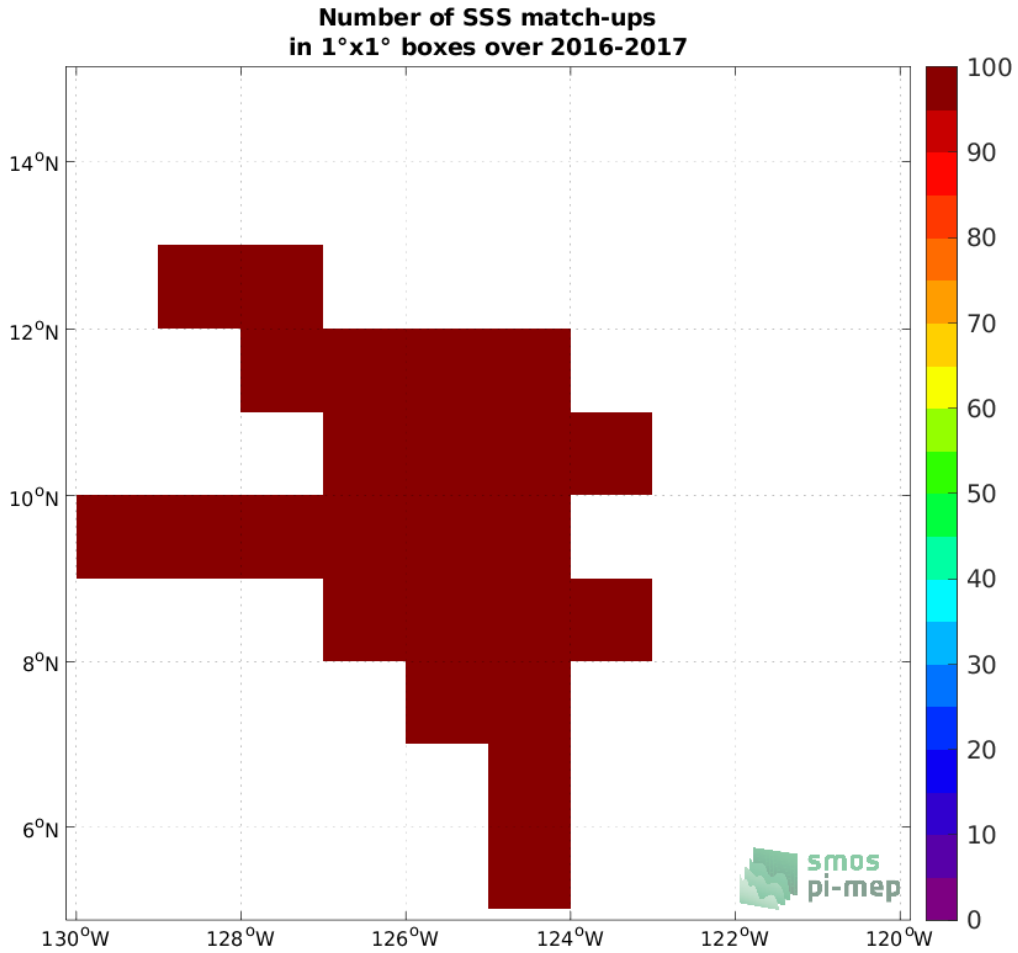
Figure 4: Number of SSS match-ups between Salinity Snake (SPURS 2) SSS and the SMOS SSS L2Q v331 - 0.25 Deg (CATDS-CPDC) SSS product for the SPURS 2 Pi-MEP region over 1°x1° boxes and for the full satellite product period.
