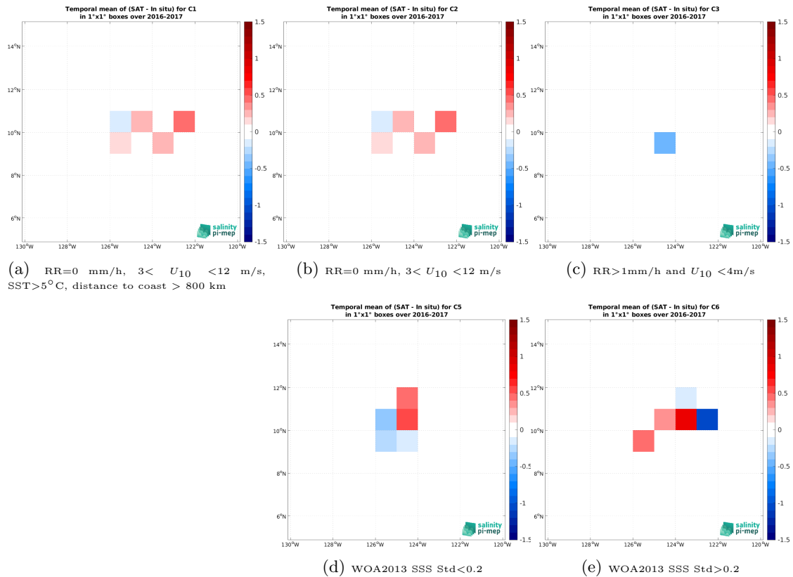
Figure 12: Temporal mean gridded over spatial boxes of size 1^\circ \times 1^\circ of \Delta SSS (SMOS SSS L2Q v331 - 0.25 Deg (CATDS-CPDC) - Seaglider (SPURS 2)) for 5 different subdatasets corresponding to:RR=0 mm/h, 3 < U_{10} < 12 m/s, SST >5^\circ C, distance to coast > 800 km (a), RR=0 mm/h, 3 < U_{10} < 12 m/s (b), RR >1 mm/h and U_{10} < 4 m/s (c), WOA2013 SSS Std <0.2 (d), WOA2013 SSS Std >0.2 (e).
