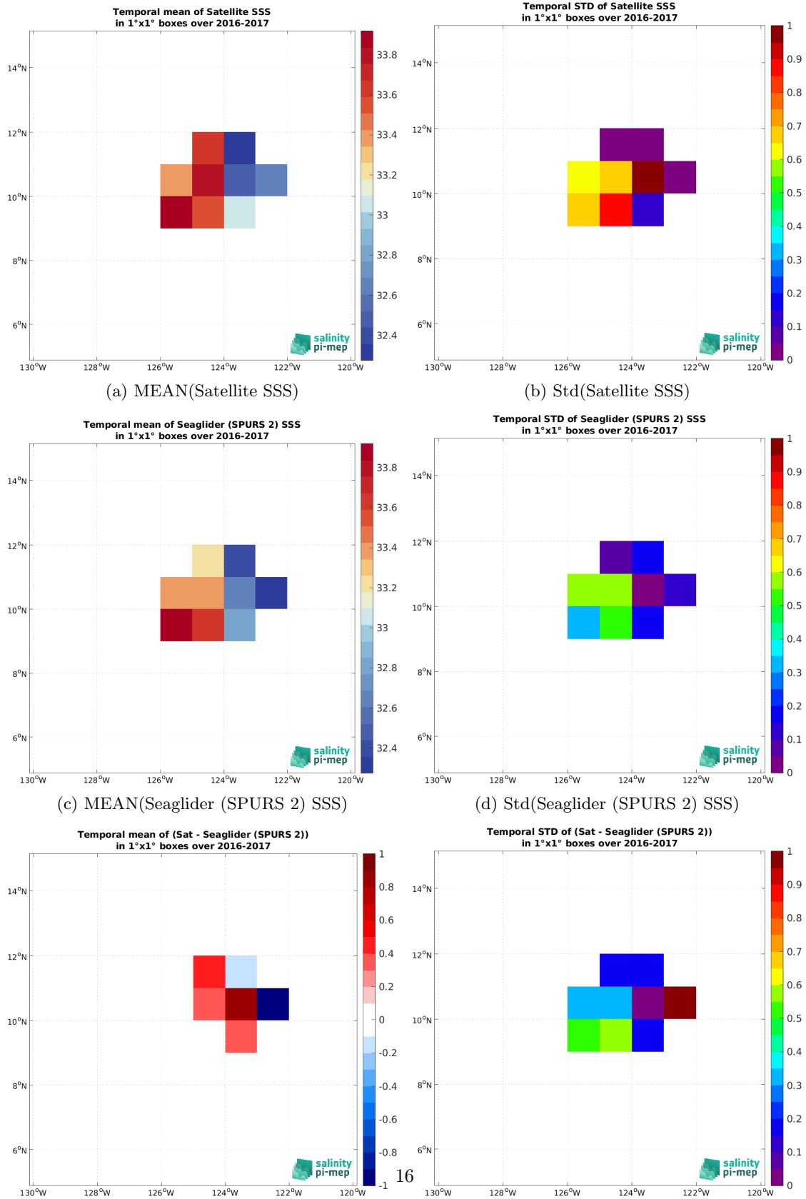
Figure 6: Temporal mean (left) and Std (right) of SSS from SMOS SSS L2Q v331 - 0.25 Deg (CATDS-CPDC) (top), Seaglider (SPURS 2) (middle), and of \Delta SSS (Satellite - Seaglider (SPURS 2)). Only match-up pairs are used to generate these maps.
