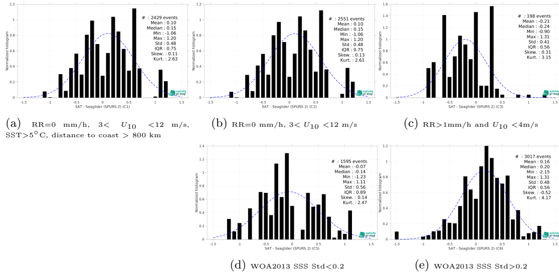
Figure 13: Normalized histogram of \Delta SSS (SMOS SSS L2Q v331 - 0.25 Deg (CATDS-CPDC) - Seaglider (SPURS 2)) for 5 different subdatasets corresponding to: RR=0 mm/h, 3 < U_{10} < 12 m/s, SST >5^{\circ} C, distance to coast > 800 km (a), RR=0 mm/h, 3 < U_{10} < 12 m/s (b), RR >1 mm/h and U_{10} < 4 m/s (c), WOA2013 SSS Std <0.2 (d), WOA2013 SSS Std >0.2 (e).
