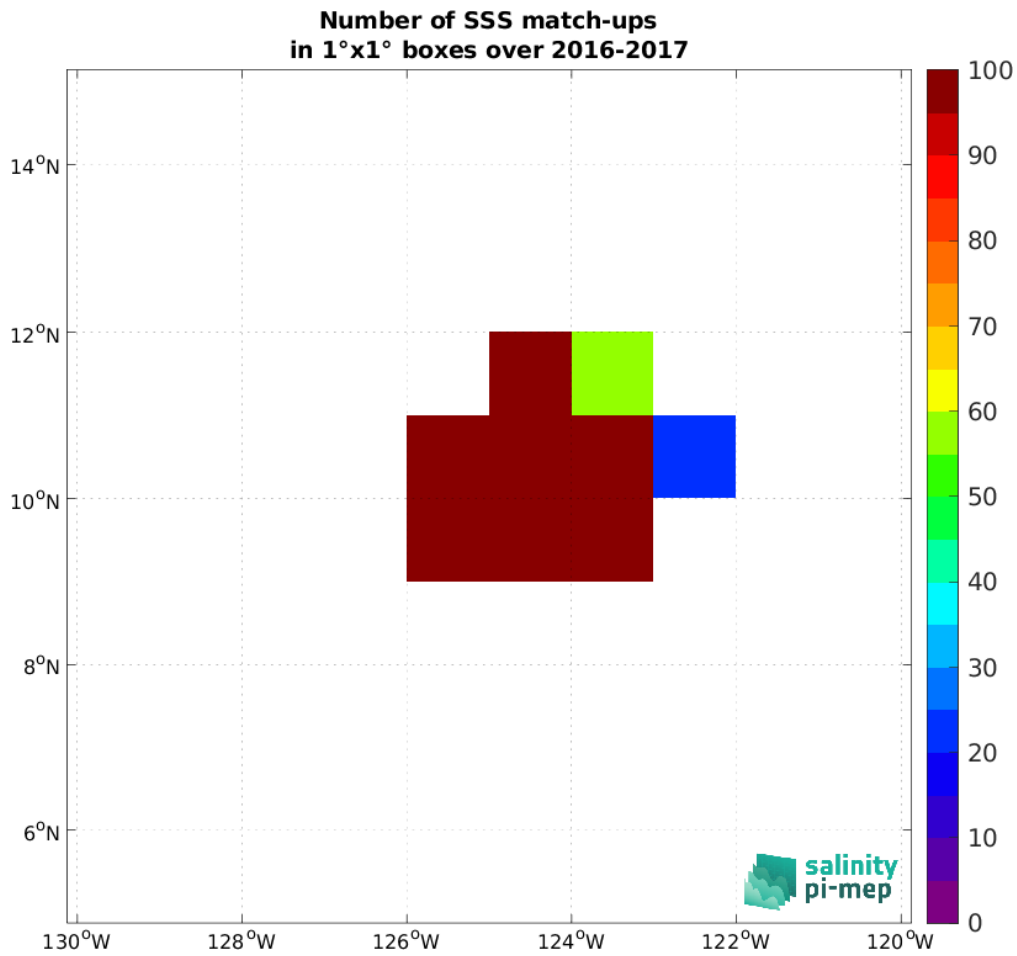
Figure 4: Number of SSS match-ups between Seaglider (SPURS 2) SSS and the SMOS SSS L2Q v331 - 0.25 Deg (CATDS-CPDC) SSS product for the SPURS 2 Pi-MEP region over 1°x1° boxes and for the full satellite product period.
