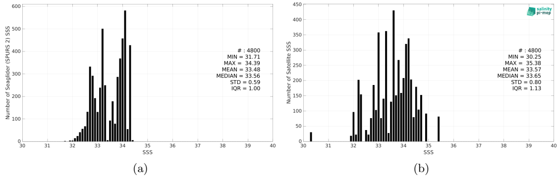
Figure 2: Histograms of SSS from Seaglider (SPURS 2) (a) and SMOS SSS L2Q v331 - 0.25 Deg (CATDS-CPDC) (b) considering all match-up pairs per bins of 0.1 over the SPURS 2 Pi-MEP region and for the full satellite product period.
