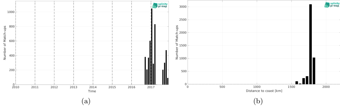
Figure 1: Number of match-ups between Seaglider (SPURS 2) and SMOS SSS L2Q v331 - 0.25 Deg (CATDS-CPDC) SSS as a function of time (a) and as function of the distance to coast (b) over the SPURS 2 Pi-MEP region and for the full satellite product period.
