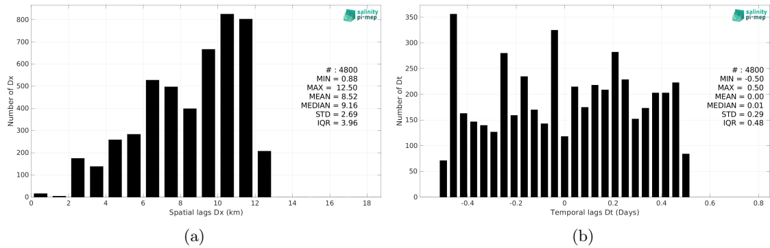
Figure 5: Histograms of the spatial (a) and temporal (b) lags between the location/time of the Seaglider (SPURS 2) measurement and the date of the corresponding SMOS SSS L2Q v331 - 0.25 Deg (CATDS-CPDC) SSS pixel.
