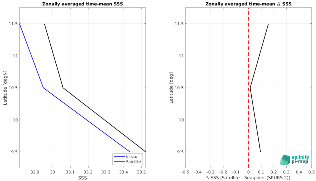
Figure 8: Left panel: Zonal mean SSS from SMOS SSS L2Q v331 - 0.25 Deg (CATDS-CPDC) satellite product (black) and from Seaglider (SPURS 2) (blue). Right panel: Zonal mean of \Delta SSS (Satellite - Seaglider (SPURS 2)) for all the collected Pi-MEP match-up pairs estimated over the full satellite product period.
