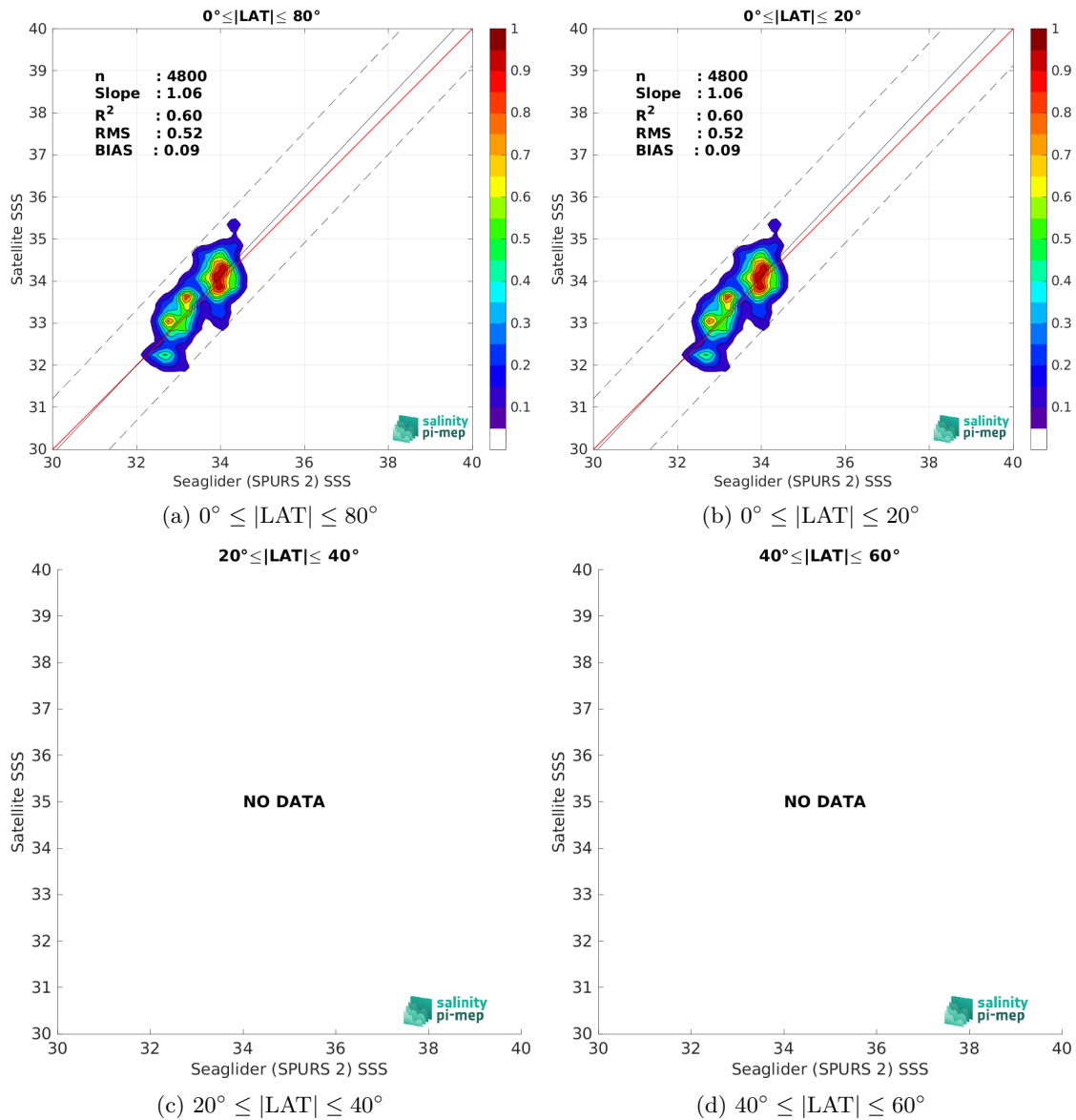
Figure 9: Contour maps of the concentration of SMOS SSS L2Q v331 - 0.25 Deg (CATDS-CPDC) SSS (y-axis) versus Seaglider (SPURS 2) SSS (x-axis) at match-up pairs for different latitude bands. For each plot, the red line shows x=y . The black thin and dashed lines indicate a linear fit through the data cloud and the \pm 95\% confidence levels, respectively. The number match-up pairs n , the slope and R^2 coefficient of the linear fit, the root mean square (RMS) and the mean bias between satellite and in situ data are indicated for each latitude band in each plots.
