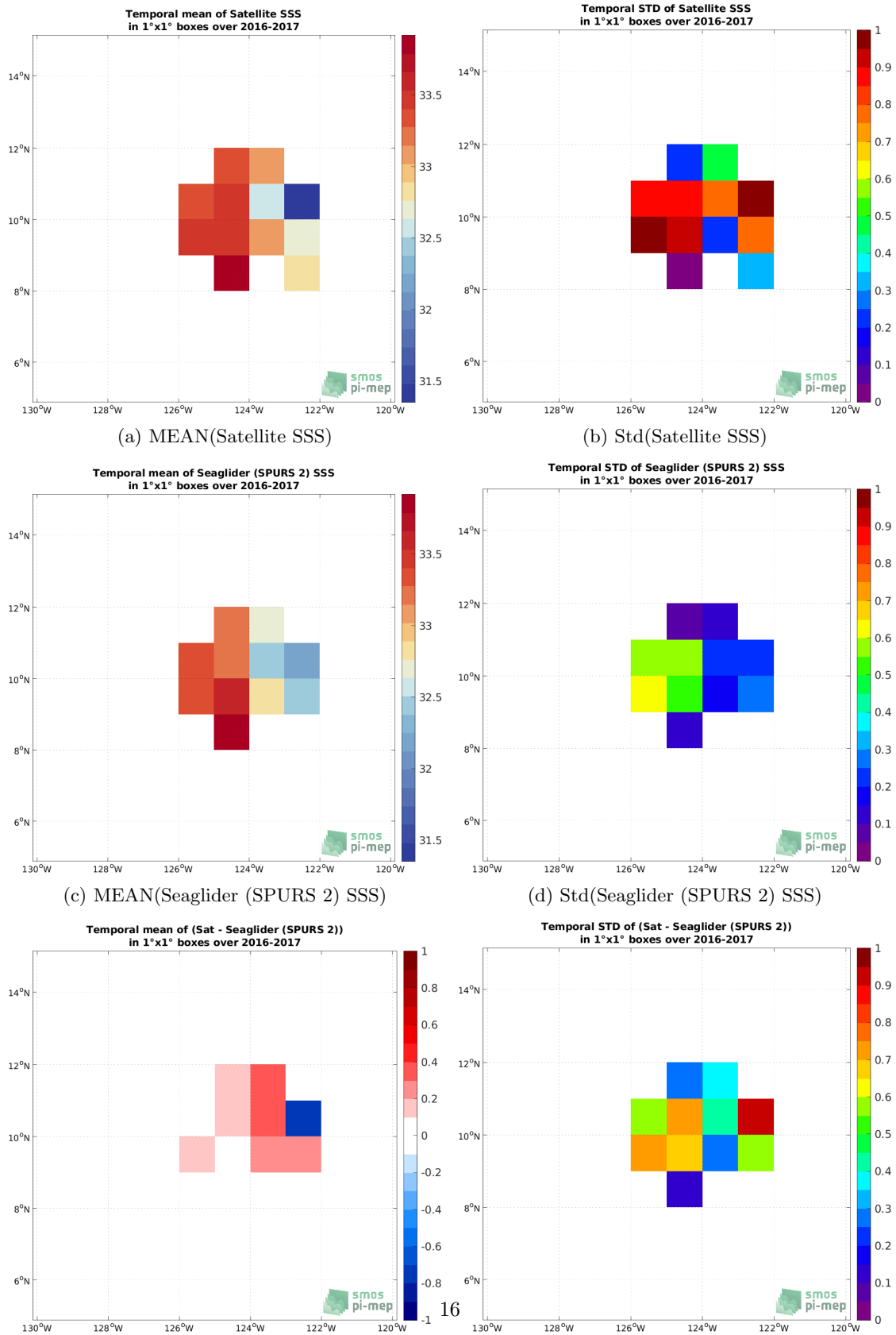
(e) MEAN( \Delta SSS) (Satellite - Seaglider (SPURS 2)) (f) Std( \Delta SSS) (Satellite - Seaglider (SPURS 2)) Figure 6: Temporal mean (left) and Std (right) of SSS from SMOS SSS L2Q v331 - 0.25 Deg (CATDS-CPDC) (top), Seaglider (SPURS 2) (middle), and of \Delta SSS (Satellite - Seaglider (SPURS 2)). Only match-up pairs are used to generate these maps.
