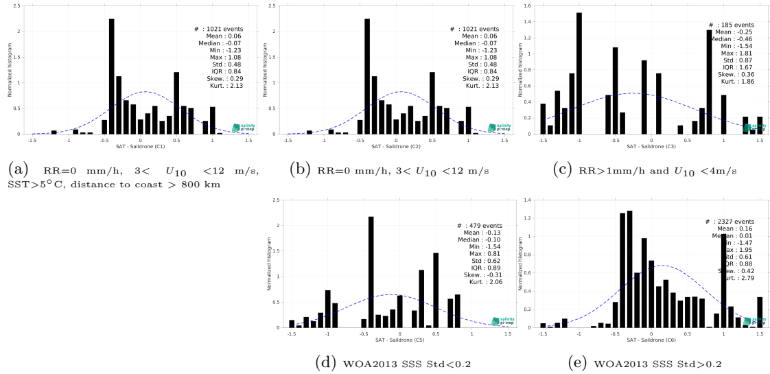
Figure 13: Normalized histogram of \Delta SSS (SMOS SSS L2Q v331 - 0.25 Deg (CATDS-CPDC) - Sailability) for 5 different subdatasets corresponding to: RR=0 mm/h, 3 < U_{10} < 12 m/s, SST > 5°C, distance to coast > 800 km (a), RR=0 mm/h, 3 < U_{10} < 12 m/s (b), RR > 1mm/h and U_{10} < 4 m/s (c), WOA2013 SSS Std < 0.2 (d), WOA2013 SSS Std > 0.2 (e).
