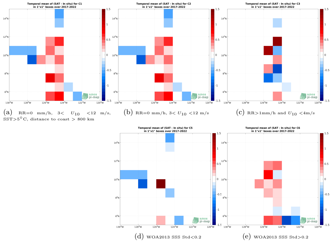
Figure 12: Temporal mean gridded over spatial boxes of size 1^\circ \times 1^\circ of \Delta SSS (SMOS SSS L2Q v331 - 0.25 Deg (CATDS-CPDC) - Saildrone) for 5 different subdatasets corresponding to:RR=0 mm/h, 3 < U_{10} < 12 m/s, SST >5^\circ C, distance to coast > 800 km (a), RR=0 mm/h, 3 < U_{10} < 12 m/s (b), RR >1 mm/h and U_{10} < 4 m/s (c), WOA2013 SSS Std <0.2 (d), WOA2013 SSS Std >0.2 (e).
