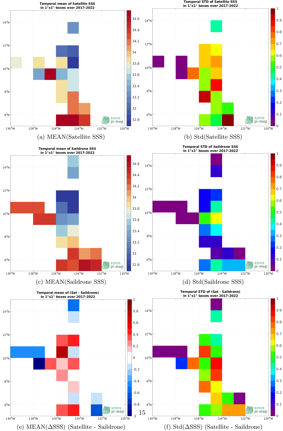
Figure 6: Temporal mean (left) and Std (right) of SSS from SMOS SSS L2Q v331 - 0.25 Deg (CATDS-CPDC) (top), Saildrone (middle), and of \Delta SSS (Satellite - Saildrone). Only match-up pairs are used to generate these maps.
