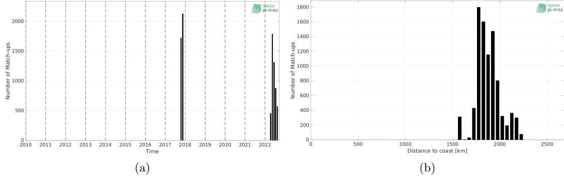
Figure 1: Number of match-ups between Saildrone and SMOS SSS L2Q v331 - 0.25 Deg (CATDS-CPDC) SSS as a function of time (a) and as function of the distance to coast (b) over the SPURS 2 Pi-MEP region and for the full satellite product period.
