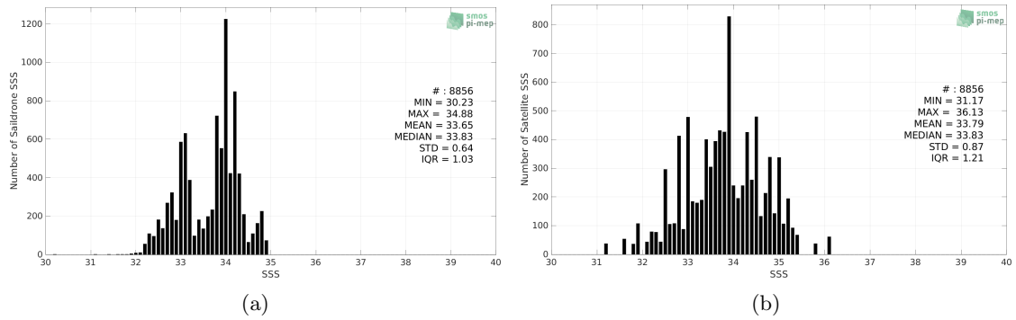
Figure 2: Histograms of SSS from Saildrone (a) and SMOS SSS L2Q v331 - 0.25 Deg (CATDS-CPDC) (b) considering all match-up pairs per bins of 0.1 over the SPURS 2 Pi-MEP region and for the full satellite product period.
