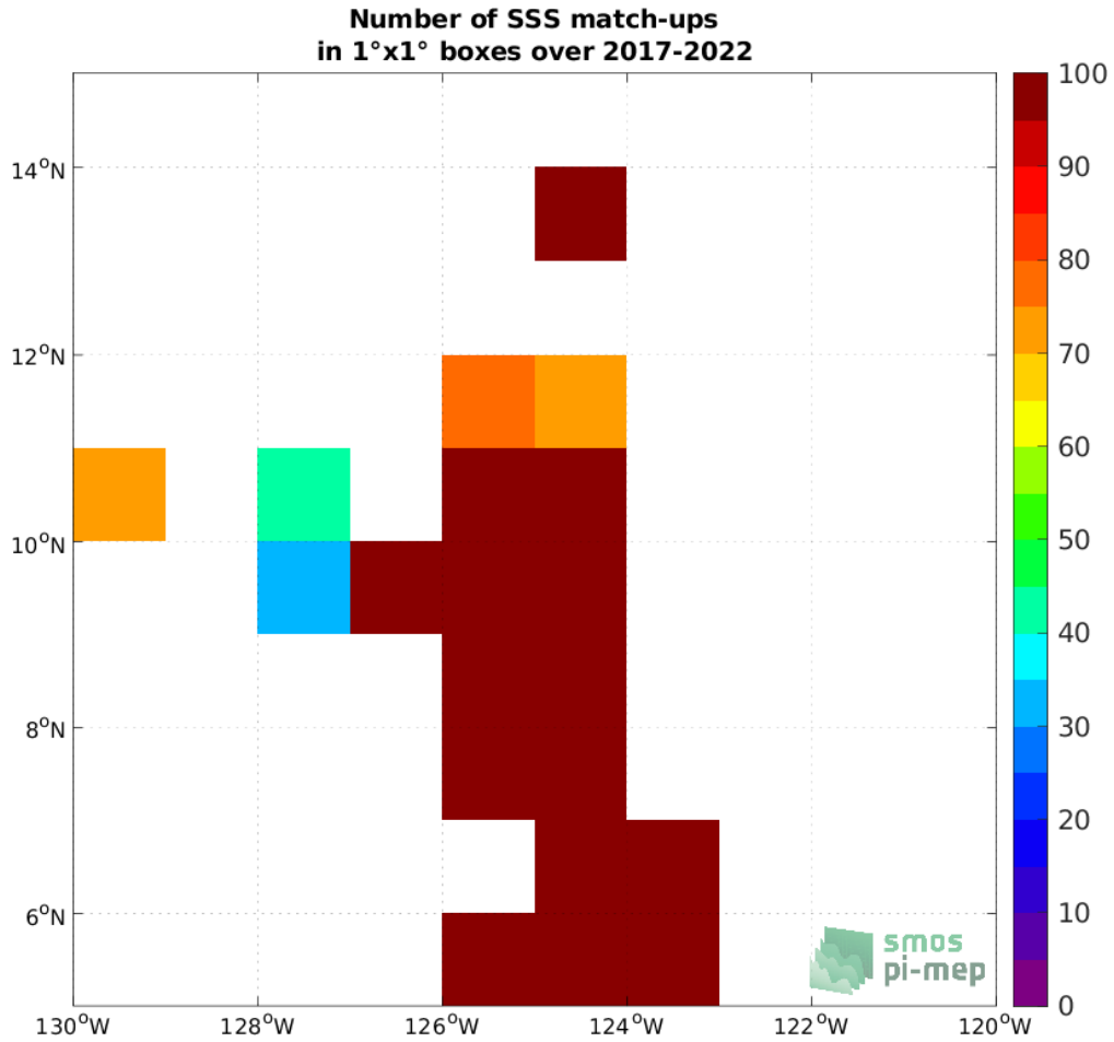
Figure 4: Number of SSS match-ups between Saildrone SSS and the SMOS SSS L2Q v331 - 0.25 Deg (CATDS-CPDC) SSS product for the SPURS 2 Pi-MEP region over 1°x1° boxes and for the full satellite product period.
