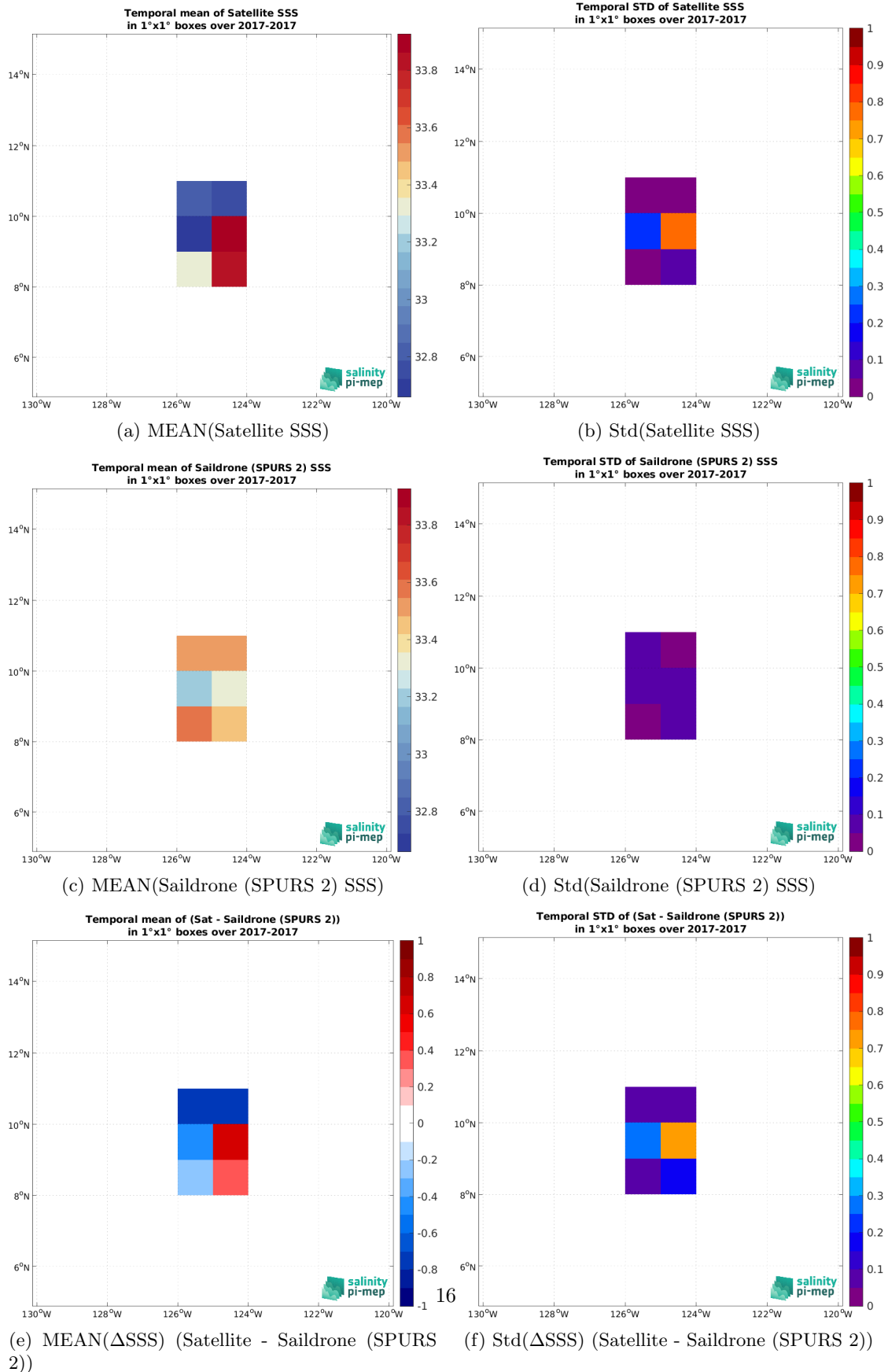
Figure 6: Temporal mean (left) and Std (right) of SSS from SMOS SSS L2Q v331 - 0.25 Deg (CATDS-CPDC) (top), Saildrone (SPURS 2) (middle), and of \Delta SSS (Satellite - Saildrone (SPURS 2)). Only match-up pairs are used to generate these maps.
