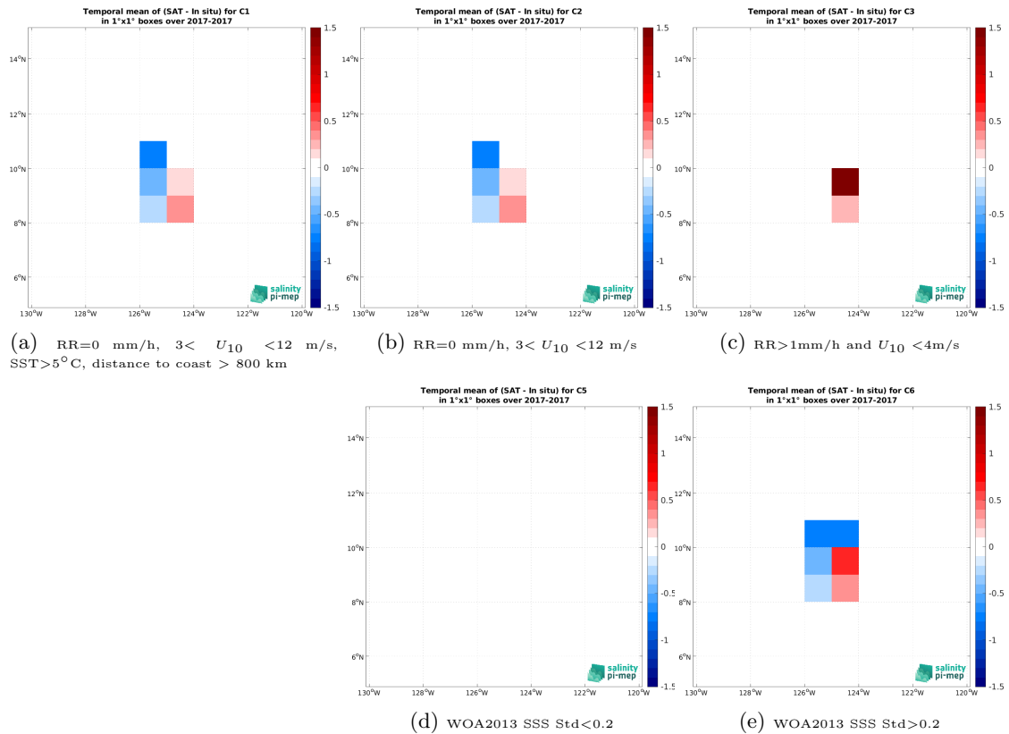
Figure 12: Temporal mean gridded over spatial boxes of size 1^\circ \times 1^\circ of \Delta SSS (SMOS SSS L2Q v331 - 0.25 Deg (CATDS-CPDC) - Saildrone (SPURS 2)) for 5 different subdatasets corresponding to: RR=0 mm/h, 3 < U_{10} < 12 m/s, SST > 5^\circ\text{C} , distance to coast > 800 km (a), RR=0 mm/h, 3 < U_{10} < 12 m/s (b), RR > 1 mm/h and U_{10} < 4 m/s (c), WOA2013 SSS Std < 0.2 (d), WOA2013 SSS Std > 0.2 (e).
