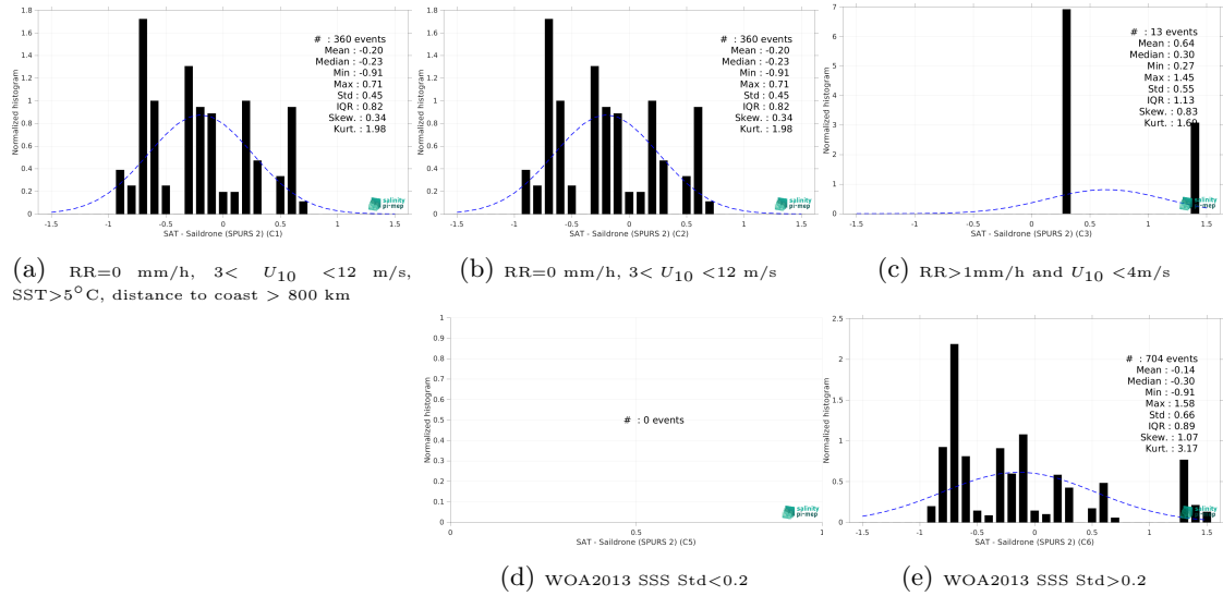
Figure 13: Normalized histogram of \Delta SSS (SMOS SSS L2Q v331 - 0.25 Deg (CATDS-CPDC) - Saildrone (SPURS 2)) for 5 different subdatasets corresponding to: RR=0 mm/h, 3 < U_{10} < 12 m/s, SST>5°C, distance to coast > 800 km (a), RR=0 mm/h, 3 < U_{10} < 12 m/s (b), RR>1mm/h and U_{10} < 4 m/s (c), WOA2013 SSS Std<0.2 (d), WOA2013 SSS Std>0.2 (e).
