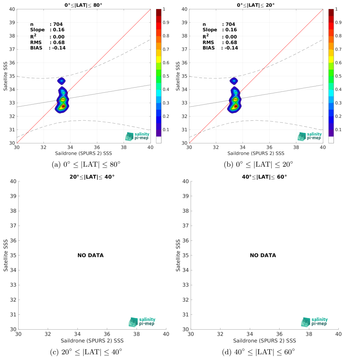
Figure 9: Contour maps of the concentration of SMOS SSS L2Q v331 - 0.25 Deg (CATDS-CPDC) SSS (y-axis) versus Saildrone (SPURS 2) SSS (x-axis) at match-up pairs for different latitude bands. For each plot, the red line shows x=y . The black thin and dashed lines indicate a linear fit through the data cloud and the \pm 95\% confidence levels, respectively. The number match-up pairs n , the slope and R^2 coefficient of the linear fit, the root mean square (RMS) and the mean bias between satellite and in situ data are indicated for each latitude band in each plots.
