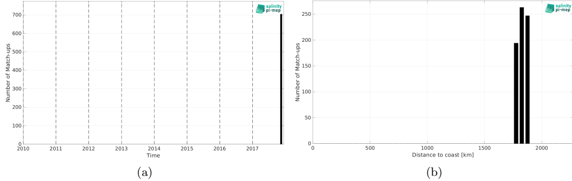
Figure 1: Number of match-ups between Saildrone (SPURS 2) and SMOS SSS L2Q v331 - 0.25 Deg (CATDS-CPDC) SSS as a function of time (a) and as function of the distance to coast (b) over the SPURS 2 Pi-MEP region and for the full satellite product period.
