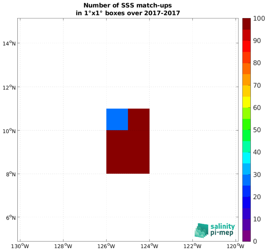
Figure 4: Number of SSS match-ups between Sairdrones (SPURS 2) SSS and the SMOS SSS L2Q v331 - 0.25 Deg (CATDS-CPDC) SSS product for the SPURS 2 Pi-MEP region over 1°x1° boxes and for the full satellite product period.
