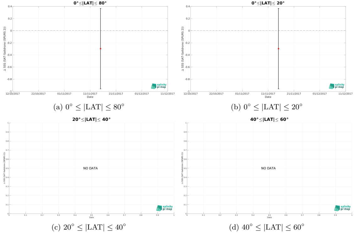
Figure 10: Monthly median (red curves) of \Delta\text{SSS} (Satellite - Sailability (SPURS 2)) and \pm 1 Std (black vertical thick bars) as function of time for all the collected Pi-MEP match-up pairs estimated over the SPURS 2 Pi-MEP region and for the full satellite product period are shown for different latitude bands: (a) 80°S-80°N, (b) 20°S-20°N, (c) 40°S-20°S and 20°N-40°N and (d) 60°S-40°S and 40°N-60°N.
