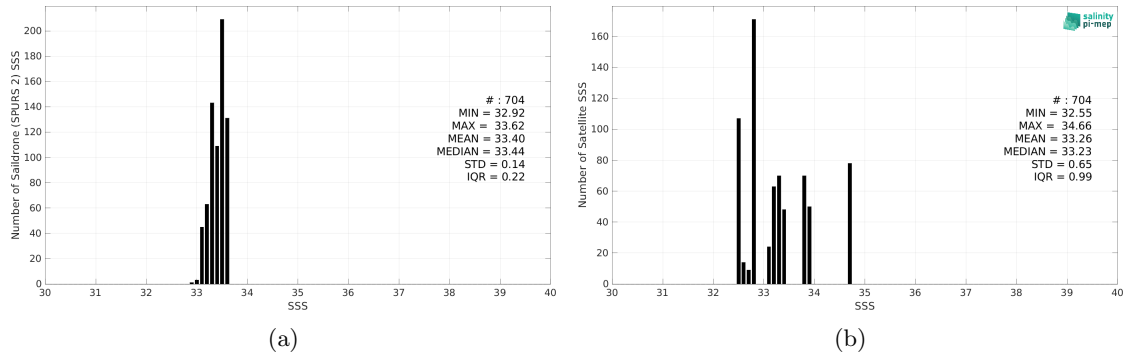
Figure 2: Histograms of SSS from Saildrone (SPURS 2) (a) and SMOS SSS L2Q v331 - 0.25 Deg (CATDS-CPDC) (b) considering all match-up pairs per bins of 0.1 over the SPURS 2 Pi-MEP region and for the full satellite product period.
