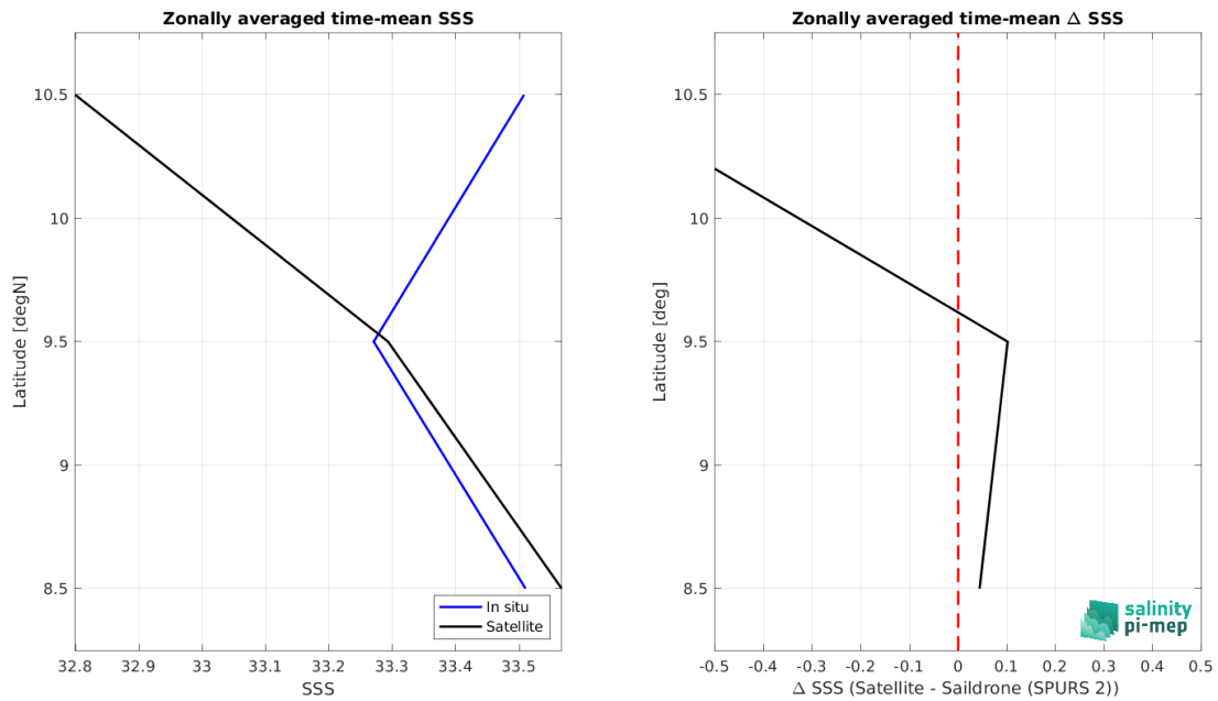
Figure 8: Left panel: Zonal mean SSS from SMOS SSS L2Q v331 - 0.25 Deg (CATDS-CPDC) satellite product (black) and from Saildrone (SPURS 2) (blue). Right panel: Zonal mean of \Delta SSS (Satellite - Saildrone (SPURS 2)) for all the collected Pi-MEP match-up pairs estimated over the full satellite product period.
