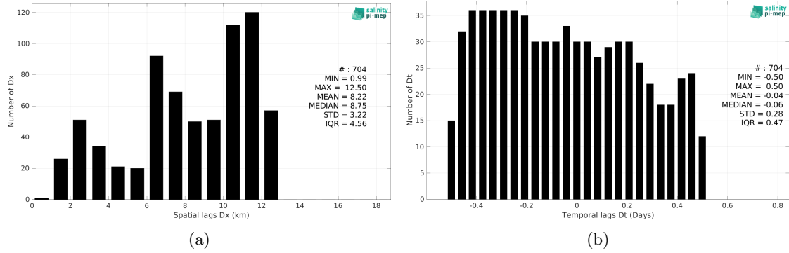
Figure 5: Histograms of the spatial (a) and temporal (b) lags between the location/time of the Saildrone (SPURS 2) measurement and the date of the corresponding SMOS SSS L2Q v331 - 0.25 Deg (CATDS-CPDC) SSS pixel.
