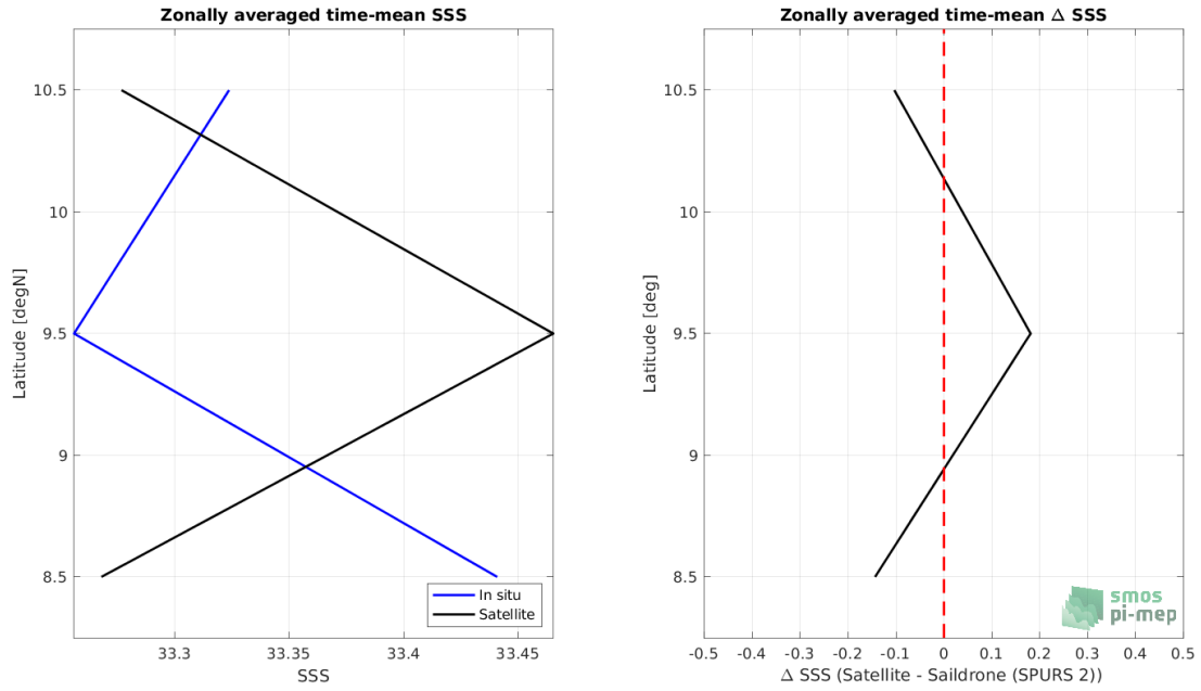
Figure 8: Left panel: Zonal mean SSS from SMOS SSS L2Q v331 - 0.25 Deg (CATDS-CPDC) satellite product (black) and from Sairdrone (SPURS 2) (blue). Right panel: Zonal mean of \Delta SSS (Satellite - Sairdrone (SPURS 2)) for all the collected Pi-MEP match-up pairs estimated over the full satellite product period.
