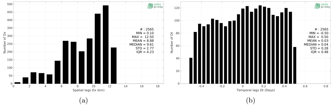
Figure 5: Histograms of the spatial (a) and temporal (b) lags between the location/time of the Sairdrone (SPURS 2) measurement and the date of the corresponding SMOS SSS L2Q v331 - 0.25 Deg (CATDS-CPDC) SSS pixel.
