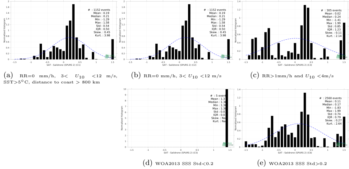
Figure 13: Normalized histogram of \Delta SSS (SMOS SSS L2Q v331 - 0.25 Deg (CATDS-CPDC) - Saildrone (SPURS 2)) for 5 different subdatasets corresponding to: RR=0 mm/h, 3 < U_{10} < 12 m/s, SST > 5°C, distance to coast > 800 km (a), RR=0 mm/h, 3 < U_{10} < 12 m/s (b), RR > 1mm/h and U_{10} < 4 m/s (c), WOA2013 SSS Std < 0.2 (d), WOA2013 SSS Std > 0.2 (e).
