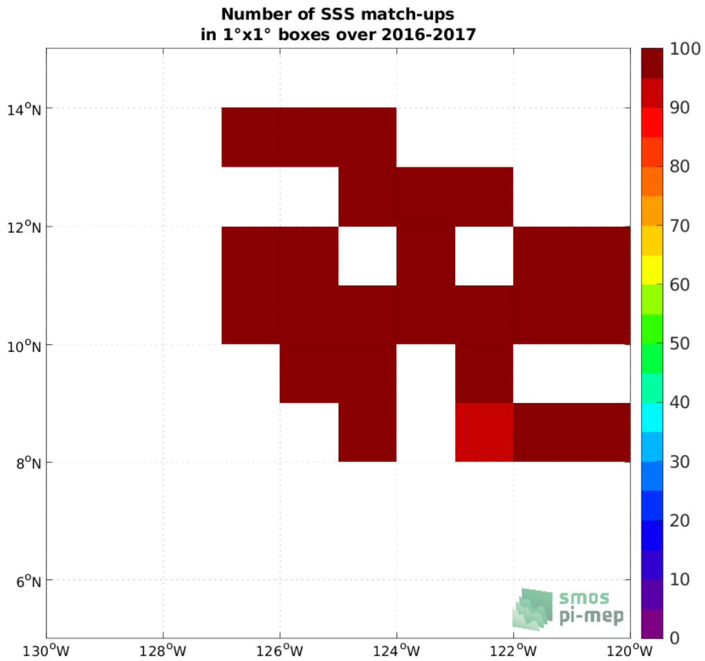
Figure 3: Number of SSS match-ups between Waveglider SSS and the SMOS SSS L2Q v330 - 0.25 Deg (CATDS-CPDC) SSS product for the SPURS 2 Pi-MEP region over 1°x1° boxes and for the full satellite product period.
