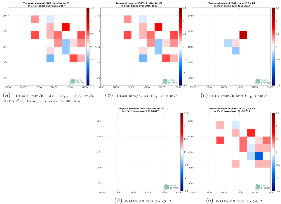
Figure 11: Temporal mean gridded over spatial boxes of size 1^\circ \times 1^\circ of \Delta SSS (SMOS SSS L2Q v330 - 0.25 Deg (CATDS-CPDC) - Waveglider) for 5 different subdatasets corresponding to: RR=0 mm/h, 3 < U_{10} < 12 m/s, SST > 5^\circ\text{C} , distance to coast > 800 km (a), RR=0 mm/h, 3 < U_{10} < 12 m/s (b), RR > 1 mm/h and U_{10} < 4 m/s (c), WOA2013 SSS Std < 0.2 (d), WOA2013 SSS Std > 0.2 (e).
