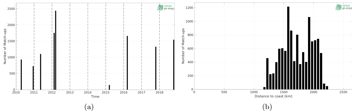
Figure 1: Number of match-ups between TSG (SAMOS) and SMOS SSS L2Q v330 - 0.25 Deg (CATDS-CPDC) SSS as a function of time (a) and as function of the distance to coast (b) over the SPURS 2 Pi-MEP region and for the full satellite product period.
