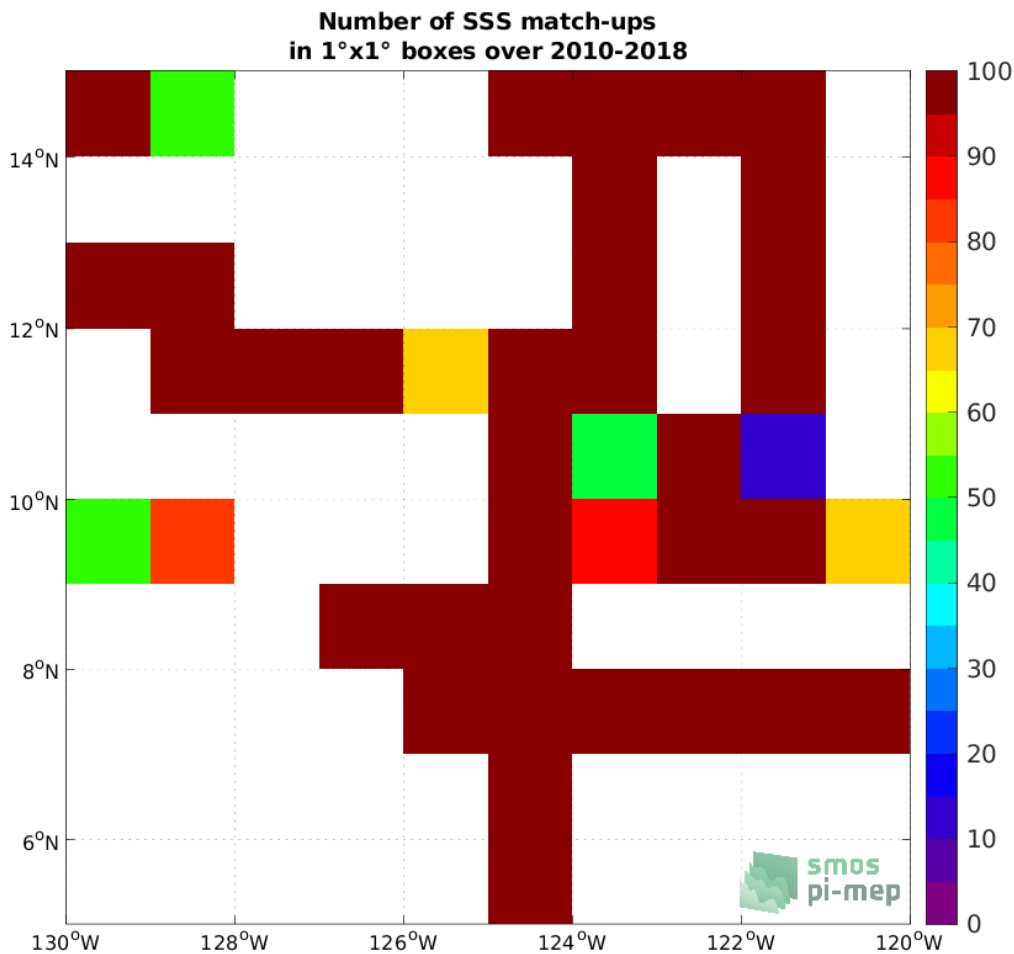
Figure 4: Number of SSS match-ups between TSG (SAMOS) SSS and the SMOS SSS L2Q v330 - 0.25 Deg (CATDS-CPDC) SSS product for the SPURS 2 Pi-MEP region over 1°x1° boxes and for the full satellite product period.
