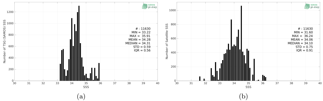
Figure 2: Histograms of SSS from TSG (SAMOS) (a) and SMOS SSS L2Q v330 - 0.25 Deg (CATDS-CPDC) (b) considering all match-up pairs per bins of 0.1 over the SPURS 2 Pi-MEP region and for the full satellite product period.
