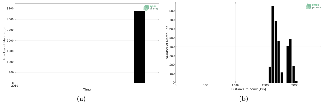
Figure 1: Number of match-ups between TSG (GOSUD-Sailing-ship) and SMOS SSS L2Q v330 - 0.25 Deg (CATDS-CPDC) SSS as a function of time (a) and as function of the distance to coast (b) over the SPURS 2 Pi-MEP region and for the full satellite product period.
