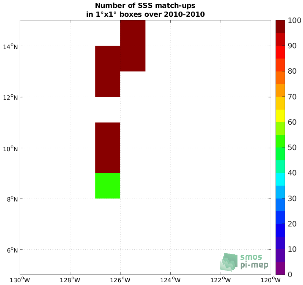
Figure 4: Number of SSS match-ups between TSG (GOSUD-Sailing-ship) SSS and the SMOS SSS L2Q v330 - 0.25 Deg (CATDS-CPDC) SSS product for the SPURS 2 Pi-MEP region over 1^\circ \times 1^\circ boxes and for the full satellite product period.
