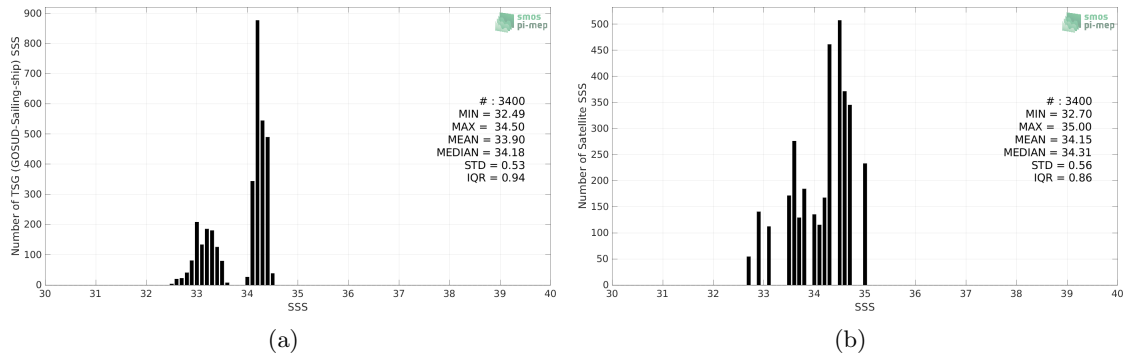
Figure 2: Histograms of SSS from TSG (GOSUD-Sailing-ship) (a) and SMOS SSS L2Q v330 - 0.25 Deg (CATDS-CPDC) (b) considering all match-up pairs per bins of 0.1 over the SPURS 2 Pi-MEP region and for the full satellite product period.
