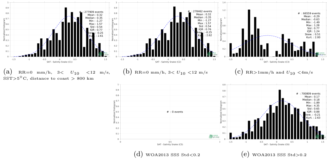
Figure 13: Normalized histogram of \Delta SSS (SMOS SSS L2Q v330 - 0.25 Deg (CATDS-CPDC) - Salinity Snake) for 5 different subdatasets corresponding to: RR=0 mm/h, 3 < U_{10} < 12 m/s, SST > 5°C, distance to coast > 800 km (a), RR=0 mm/h, 3 < U_{10} < 12 m/s (b), RR > 1mm/h and U_{10} < 4 m/s (c), WOA2013 SSS Std < 0.2 (d), WOA2013 SSS Std > 0.2 (e).
