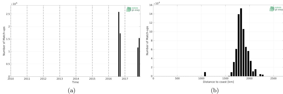
Figure 1: Number of match-ups between Salinity Snake and SMOS SSS L2Q v330 - 0.25 Deg (CATDS-CPDC) SSS as a function of time (a) and as function of the distance to coast (b) over the SPURS 2 Pi-MEP region and for the full satellite product period.
