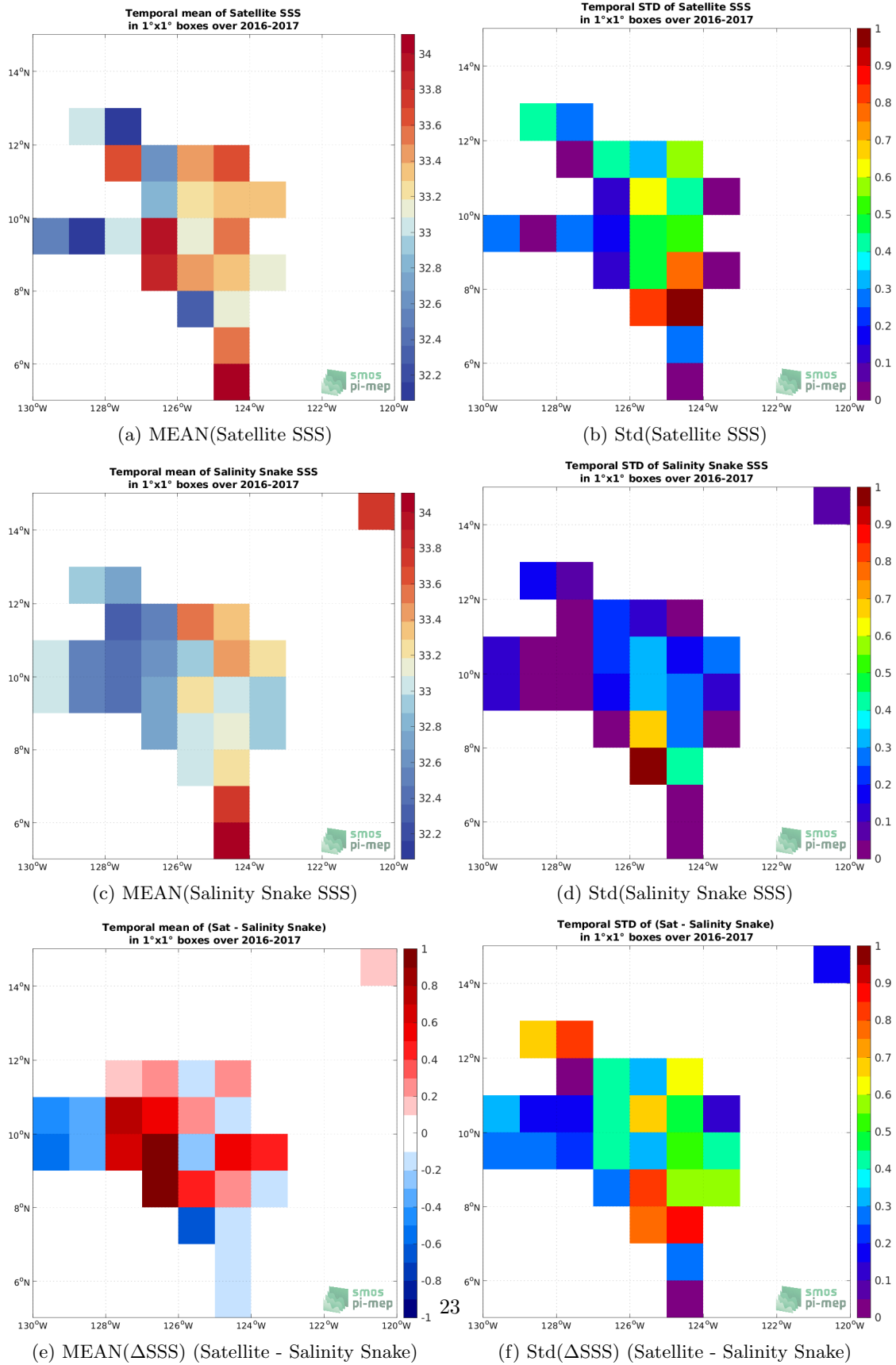
Figure 6: Temporal mean (left) and Std (right) of SSS from SMOS SSS L2Q v330 - 0.25 Deg (CATDS-CPDC) (top), Salinity Snake (middle), and of \Delta SSS (Satellite - Salinity Snake). Only match-up pairs are used to generate these maps.
