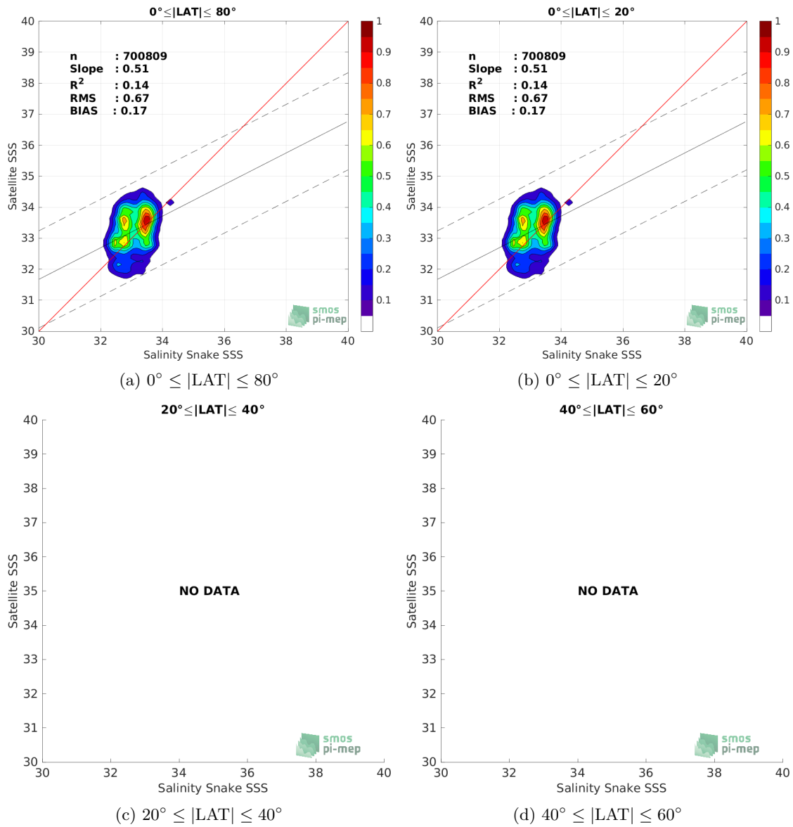
Figure 9: Contour maps of the concentration of SMOS SSS L2Q v330 - 0.25 Deg (CATDS-CPDC) SSS (y-axis) versus Salinity Snake SSS (x-axis) at match-up pairs for different latitude bands. For each plot, the red line shows x=y . The black thin and dashed lines indicate a linear fit through the data cloud and the \pm 95\% confidence levels, respectively. The number match-up pairs n , the slope and R^2 coefficient of the linear fit, the root mean square (RMS) and the mean bias between satellite and in situ data are indicated for each latitude band in each plots.
