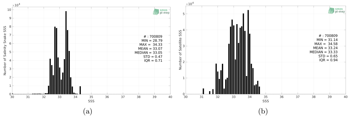
Figure 2: Histograms of SSS from Salinity Snake (a) and SMOS SSS L2Q v330 - 0.25 Deg (CATDS-CPDC) (b) considering all match-up pairs per bins of 0.1 over the SPURS 2 Pi-MEP region and for the full satellite product period.
