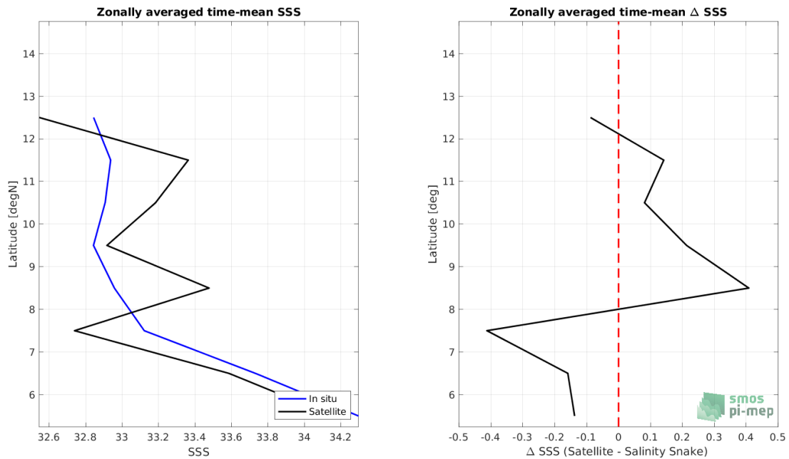
Figure 8: Left panel: Zonal mean SSS from SMOS SSS L2Q v330 - 0.25 Deg (CATDS-CPDC) satellite product (black) and from Salinity Snake (blue). Right panel: Zonal mean of \Delta SSS (Satellite - Salinity Snake) for all the collected Pi-MEP match-up pairs estimated over the full satellite product period.
