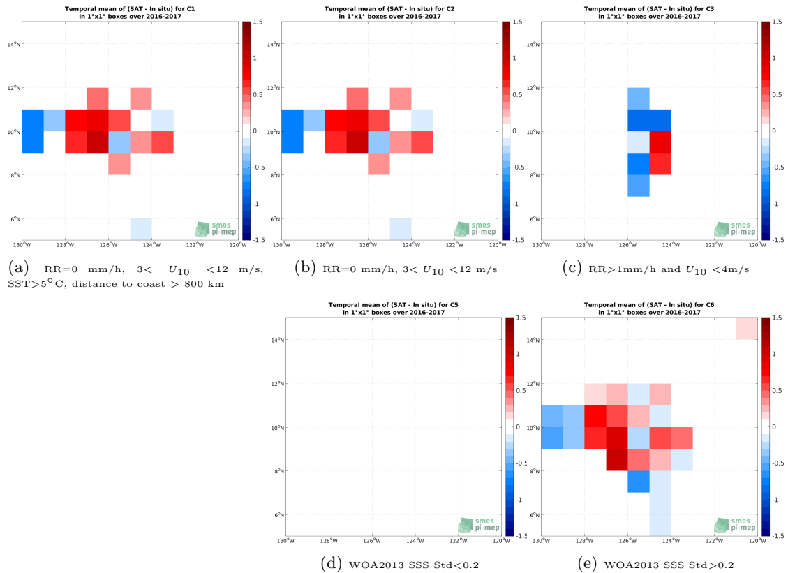
Figure 12: Temporal mean gridded over spatial boxes of size 1^\circ \times 1^\circ of \Delta SSS (SMOS SSS L2Q v330 - 0.25 Deg (CATDS-CPDC) - Salinity Snake) for 5 different subdatasets corresponding to:RR=0 mm/h, 3 < U_{10} < 12 m/s, SST >5^\circ C, distance to coast > 800 km (a), RR=0 mm/h, 3 < U_{10} < 12 m/s (b), RR >1 mm/h and U_{10} < 4 m/s (c), WOA2013 SSS Std <0.2 (d), WOA2013 SSS Std >0.2 (e).
