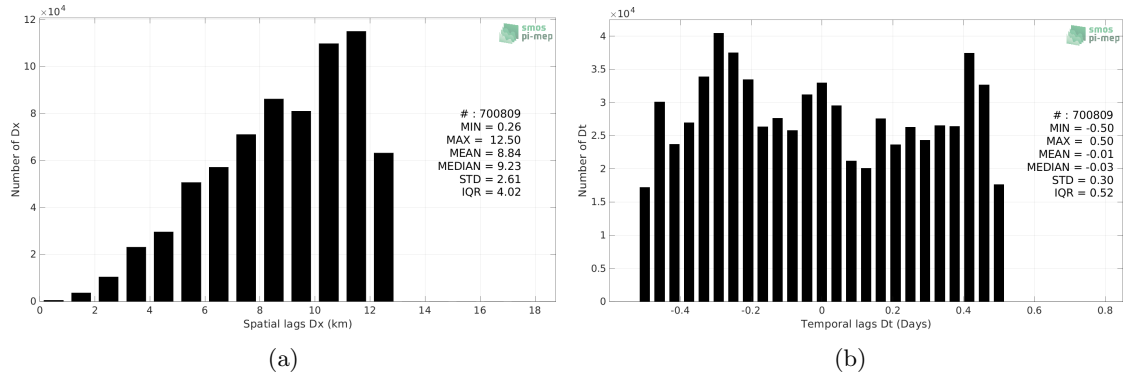
Figure 5: Histograms of the spatial (a) and temporal (b) lags between the location/time of the Salinity Snake measurement and the date of the corresponding SMOS SSS L2Q v330 - 0.25 Deg (CATDS-CPDC) SSS pixel.
