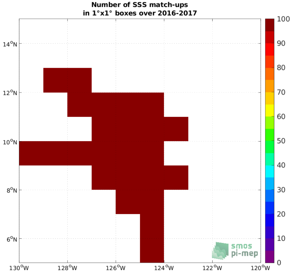
Figure 4: Number of SSS match-ups between Salinity Snake SSS and the SMOS SSS L2Q v330 - 0.25 Deg (CATDS-CPDC) SSS product for the SPURS 2 Pi-MEP region over 1^\circ \times 1^\circ boxes and for the full satellite product period.
