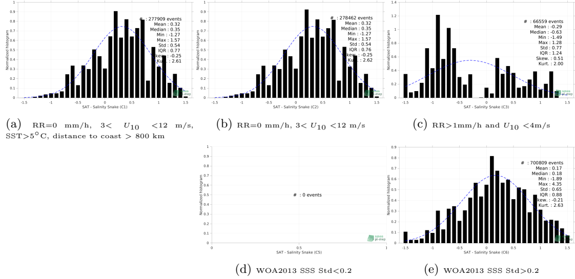
Figure 12: Normalized histogram of \Delta SSS (SMOS SSS L2Q v330 - 0.25 Deg (CATDS-CPDC) - Salinity Snake) for 5 different subdatasets corresponding to: RR=0 mm/h, 3 < U_{10} < 12 m/s, SST > 5°C, distance to coast > 800 km (a), RR=0 mm/h, 3 < U_{10} < 12 m/s (b), RR > 1mm/h and U_{10} < 4 m/s (c), WOA2013 SSS Std < 0.2 (d), WOA2013 SSS Std > 0.2 (e).
