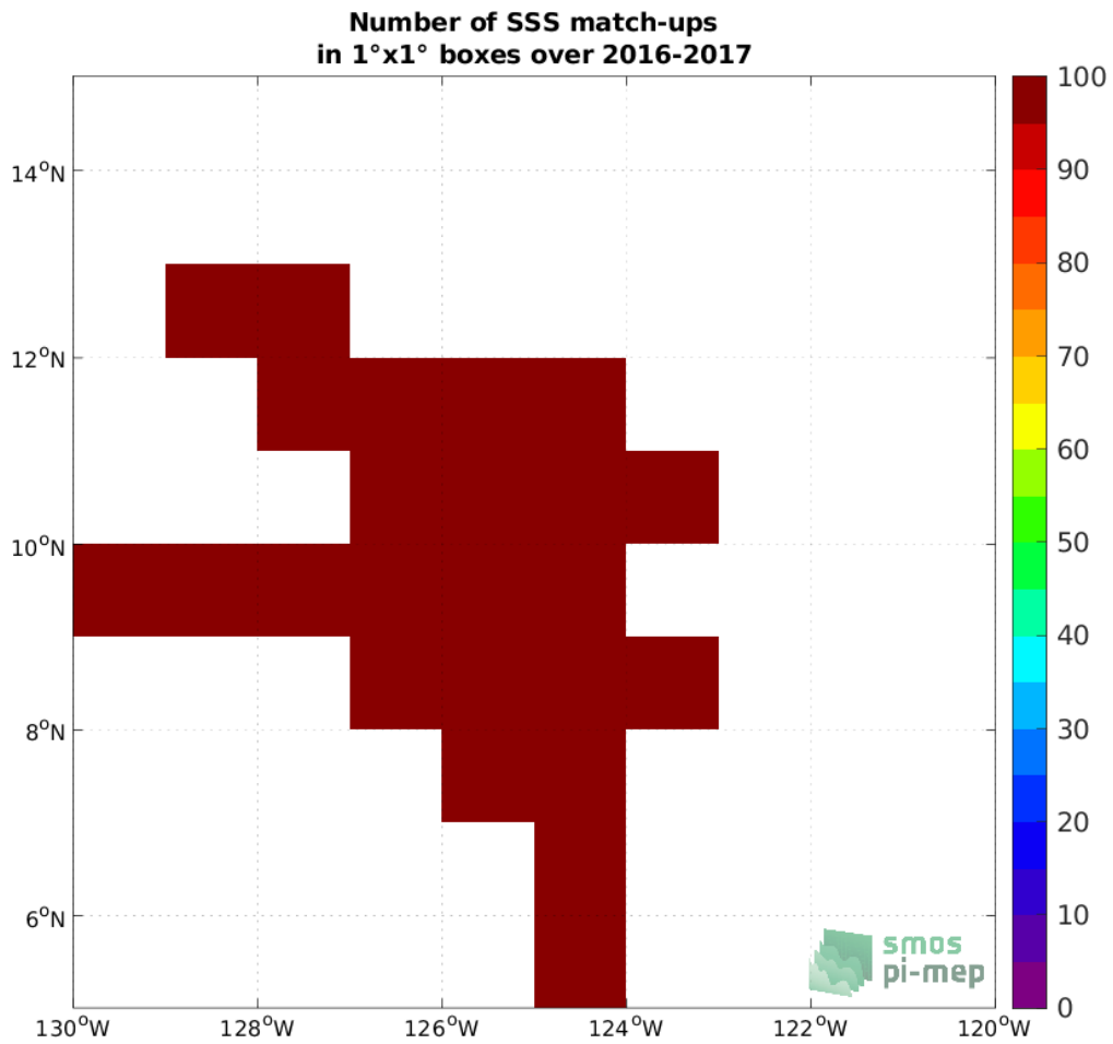
Figure 3: Number of SSS match-ups between Salinity Snake SSS and the SMOS SSS L2Q v330 - 0.25 Deg (CATDS-CPDC) SSS product for the SPURS 2 Pi-MEP region over 1°x1° boxes and for the full satellite product period.
