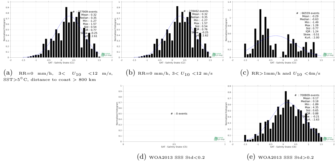
Figure 12: Normalized histogram of \Delta SSS (SMOS SSS L2Q v330 - 0.25 Deg (CATDS-CPDC) - Salinity Snake) for 5 different subdatasets corresponding to: RR=0 mm/h, 3 < U_{10} < 12 m/s, SST>5°C, distance to coast > 800 km (a), RR=0 mm/h, 3 < U_{10} < 12 m/s (b), RR>1mm/h and U_{10} < 4 m/s (c), WOA2013 SSS Std<0.2 (d), WOA2013 SSS Std>0.2 (e).
