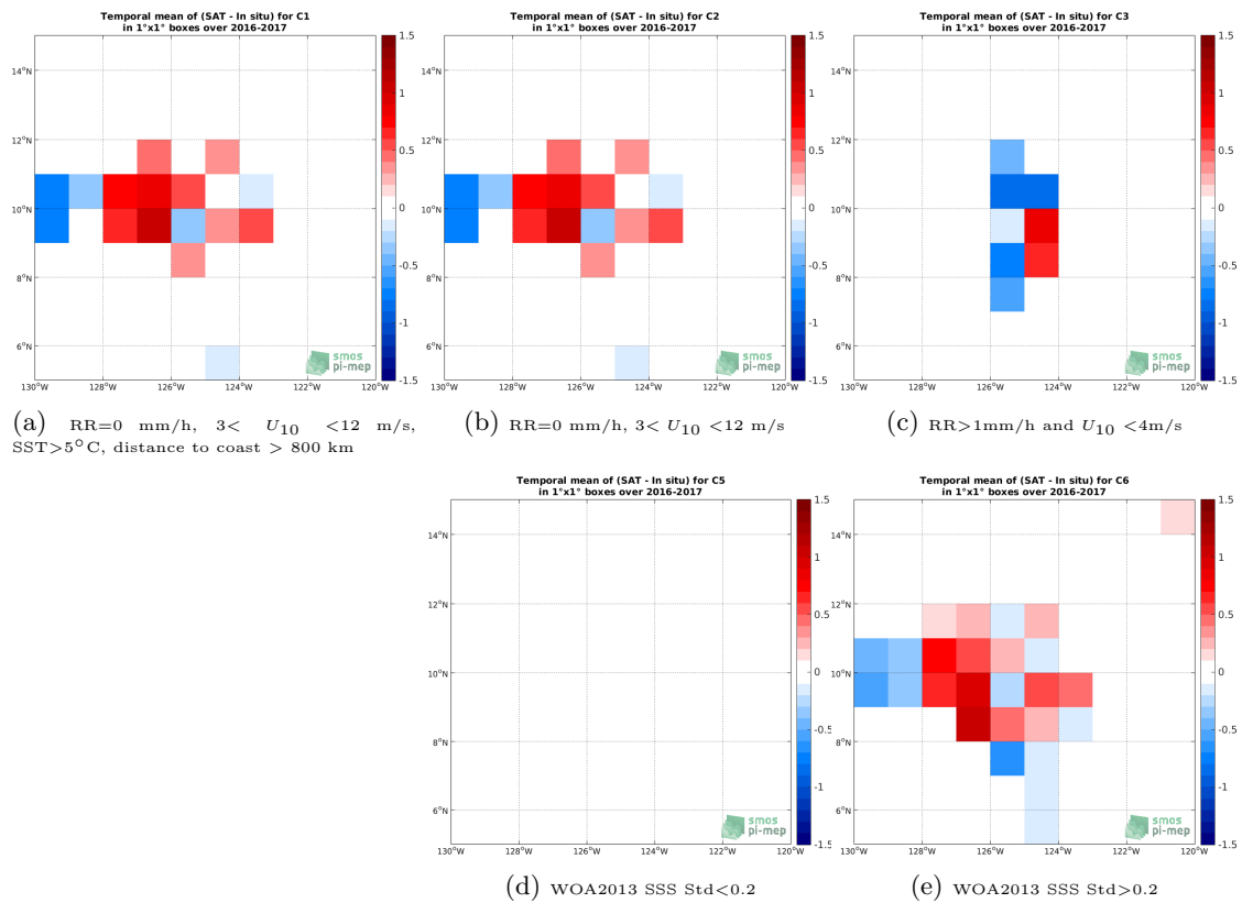
Figure 11: Temporal mean gridded over spatial boxes of size 1^\circ \times 1^\circ of \Delta SSS (SMOS SSS L2Q v330 - 0.25 Deg (CATDS-CPDC) - Salinity Snake) for 5 different subdatasets corresponding to:RR=0 mm/h, 3 < U_{10} < 12 m/s, SST >5^\circ C, distance to coast > 800 km (a), RR=0 mm/h, 3 < U_{10} < 12 m/s (b), RR >1 mm/h and U_{10} < 4 m/s (c), WOA2013 SSS Std <0.2 (d), WOA2013 SSS Std >0.2 (e).
