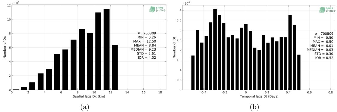
Figure 4: Histograms of the spatial (a) and temporal (b) lags between the location/time of the Salinity Snake measurement and the date of the corresponding SMOS SSS L2Q v330 - 0.25 Deg (CATDS-CPDC) SSS pixel.
