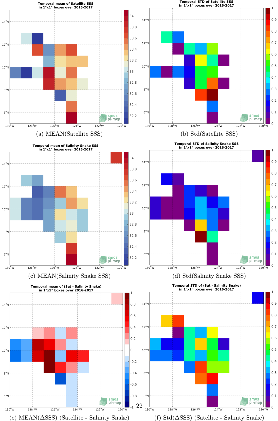
Figure 5: Temporal mean (left) and Std (right) of SSS from SMOS SSS L2Q v330 - 0.25 Deg (CATDS-CPDC) (top), Salinity Snake (middle), and of \Delta SSS (Satellite - Salinity Snake). Only match-up pairs are used to generate these maps.
