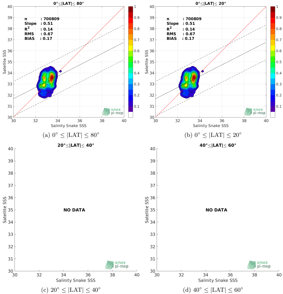
Figure 8: Contour maps of the concentration of SMOS SSS L2Q v330 - 0.25 Deg (CATDS-CPDC) SSS (y-axis) versus Salinity Snake SSS (x-axis) at match-up pairs for different latitude bands. For each plot, the red line shows x=y . The black thin and dashed lines indicate a linear fit through the data cloud and the \pm 95\% confidence levels, respectively. The number match-up pairs n , the slope and R^2 coefficient of the linear fit, the root mean square (RMS) and the mean bias between satellite and in situ data are indicated for each latitude band in each plots.
