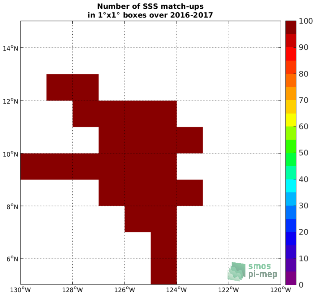
Figure 3: Number of SSS match-ups between Salinity Snake SSS and the SMOS SSS L2Q v330 - 0.25 Deg (CATDS-CPDC) SSS product for the SPURS 2 Pi-MEP region over 1°×1° boxes and for the full satellite product period.
