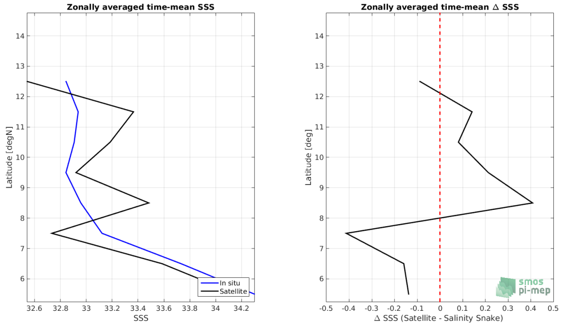
Figure 7: Left panel: Zonal mean SSS from SMOS SSS L2Q v330 - 0.25 Deg (CATDS-CPDC) satellite product (black) and from Salinity Snake (blue). Right panel: Zonal mean of \Delta SSS (Satellite - Salinity Snake) for all the collected Pi-MEP match-up pairs estimated over the full satellite product period.
