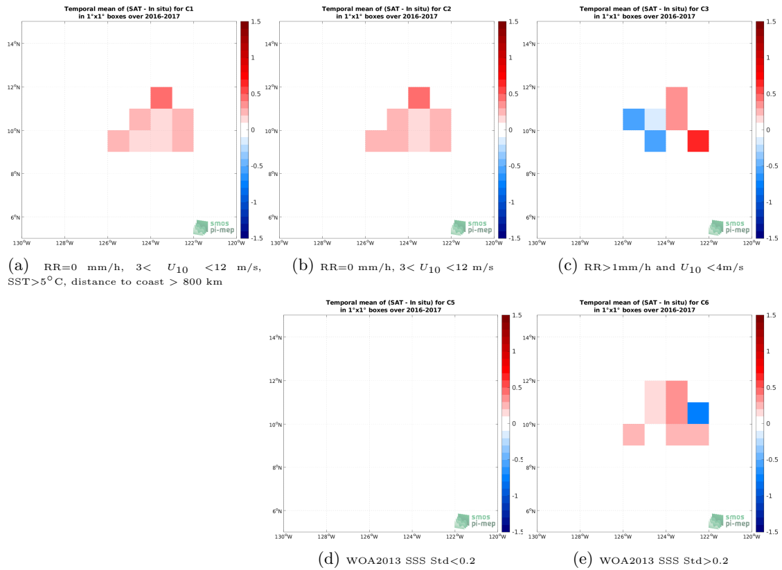
Figure 12: Temporal mean gridded over spatial boxes of size 1^\circ \times 1^\circ of \Delta SSS (SMOS SSS L2Q v330 - 0.25 Deg (CATDS-CPDC) - Seaglider) for 5 different subdatasets corresponding to:RR=0 mm/h, 3 < U_{10} < 12 m/s, SST >5^\circ C, distance to coast > 800 km (a), RR=0 mm/h, 3 < U_{10} < 12 m/s (b), RR >1 mm/h and U_{10} < 4 m/s (c), WOA2013 SSS Std <0.2 (d), WOA2013 SSS Std >0.2 (e).
