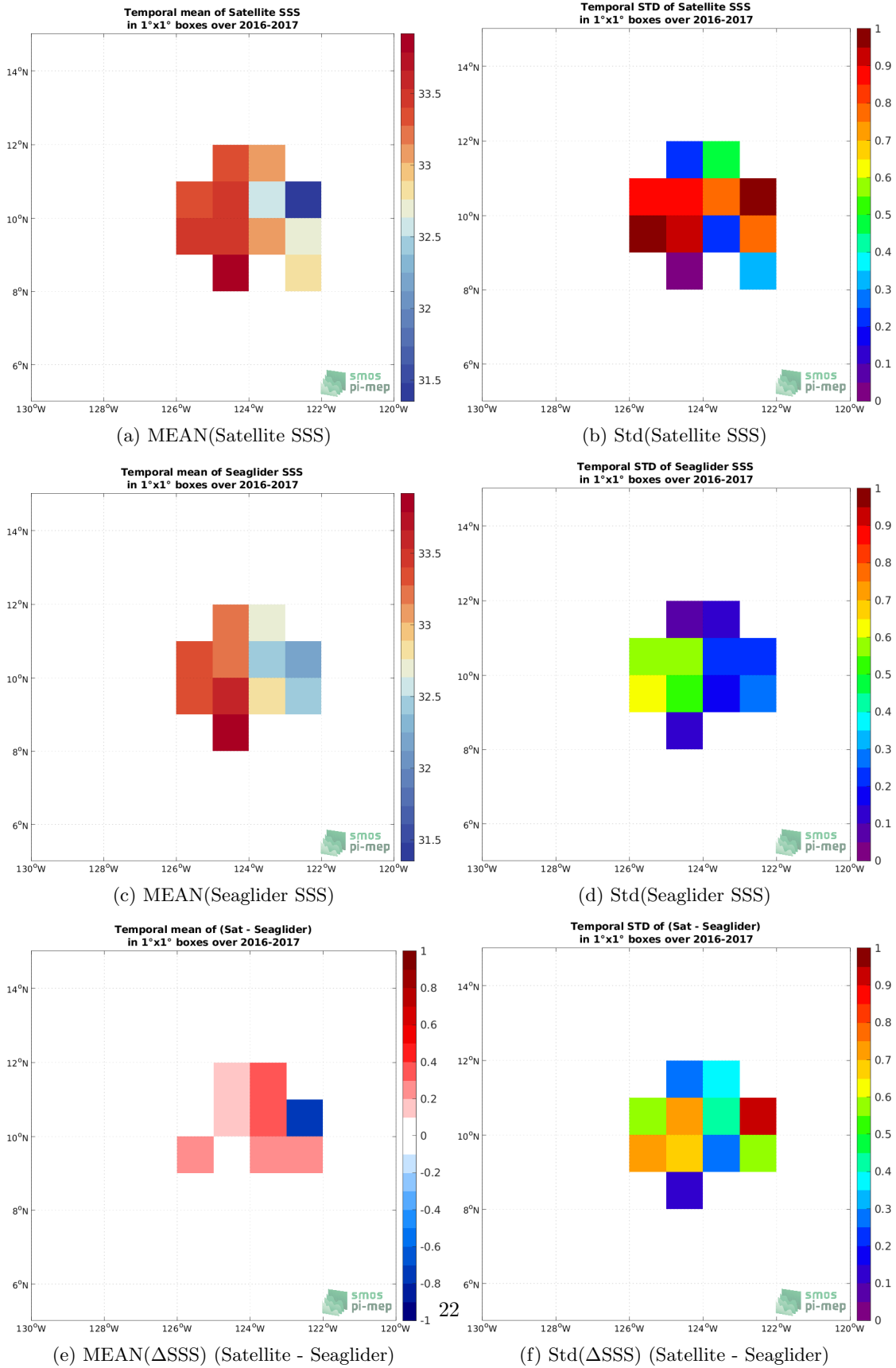
Figure 6: Temporal mean (left) and Std (right) of SSS from SMOS SSS L2Q v330 - 0.25 Deg (CATDS-CPDC) (top), Seaglider (middle), and of \Delta SSS (Satellite - Seaglider). Only match-up pairs are used to generate these maps.
