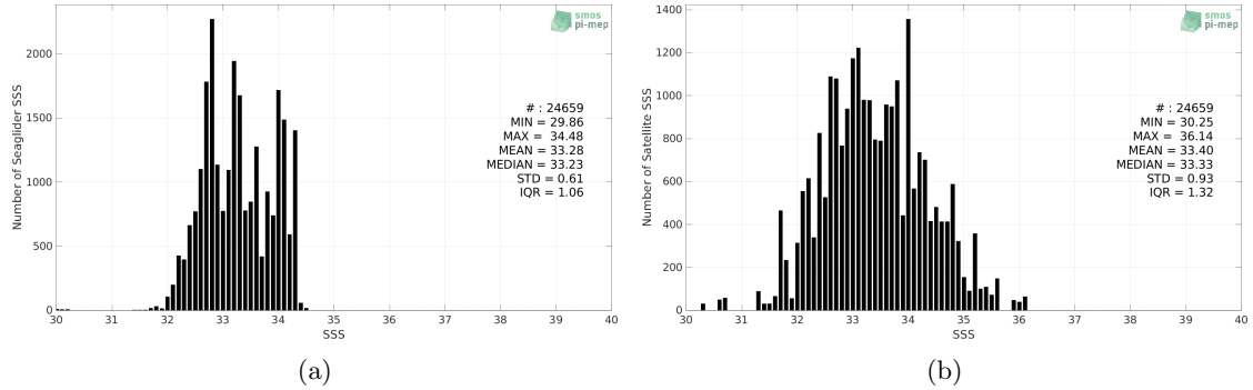
Figure 2: Histograms of SSS from Seagliders (a) and SMOS SSS L2Q v330 - 0.25 Deg (CATDS-CPDC) (b) considering all match-up pairs per bins of 0.1 over the SPURS 2 Pi-MEP region and for the full satellite product period.
