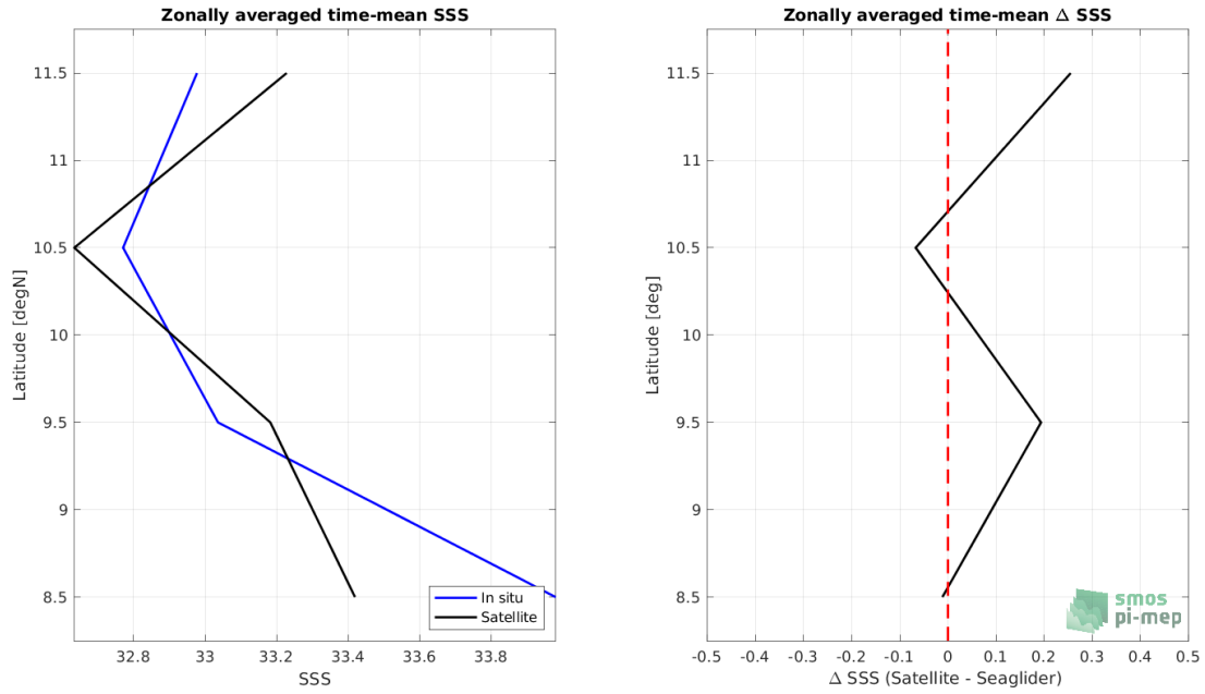
Figure 8: Left panel: Zonal mean SSS from SMOS SSS L2Q v330 - 0.25 Deg (CATDS-CPDC) satellite product (black) and from Seaglider (blue). Right panel: Zonal mean of \Delta SSS (Satellite - Seaglider) for all the collected Pi-MEP match-up pairs estimated over the full satellite product period.
