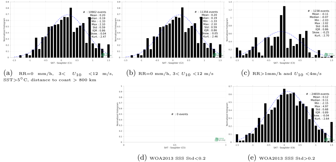
Figure 13: Normalized histogram of \Delta SSS (SMOS SSS L2Q v330 - 0.25 Deg (CATDS-CPDC) - Seaglider) for 5 different subdatasets corresponding to: RR=0 mm/h, 3 < U_{10} < 12 m/s, SST > 5°C, distance to coast > 800 km (a), RR=0 mm/h, 3 < U_{10} < 12 m/s (b), RR > 1mm/h and U_{10} < 4 m/s (c), WOA2013 SSS Std < 0.2 (d), WOA2013 SSS Std > 0.2 (e).
