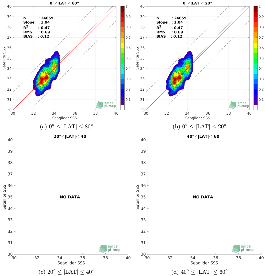
Figure 9: Contour maps of the concentration of SMOS SSS L2Q v330 - 0.25 Deg (CATDS-CPDC) SSS (y-axis) versus Seaglider SSS (x-axis) at match-up pairs for different latitude bands. For each plot, the red line shows x=y . The black thin and dashed lines indicate a linear fit through the data cloud and the \pm 95\% confidence levels, respectively. The number match-up pairs n , the slope and R^2 coefficient of the linear fit, the root mean square (RMS) and the mean bias between satellite and in situ data are indicated for each latitude band in each plots.
