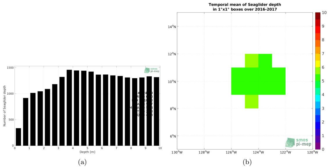
Figure 3: Histograms of the depth of the upper level SSS measurements from Seagliders in the Match-up DataBase for the SPURS 2 Pi-MEP region (a) and temporal mean spatial distribution of pressure of the in situ SSS data over 1^\circ \times 1^\circ boxes and for the full satellite product period (b).
