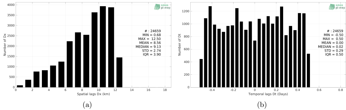
Figure 5: Histograms of the spatial (a) and temporal (b) lags between the location/time of the Seaglider measurement and the date of the corresponding SMOS SSS L2Q v330 - 0.25 Deg (CATDS-CPDC) SSS pixel.
