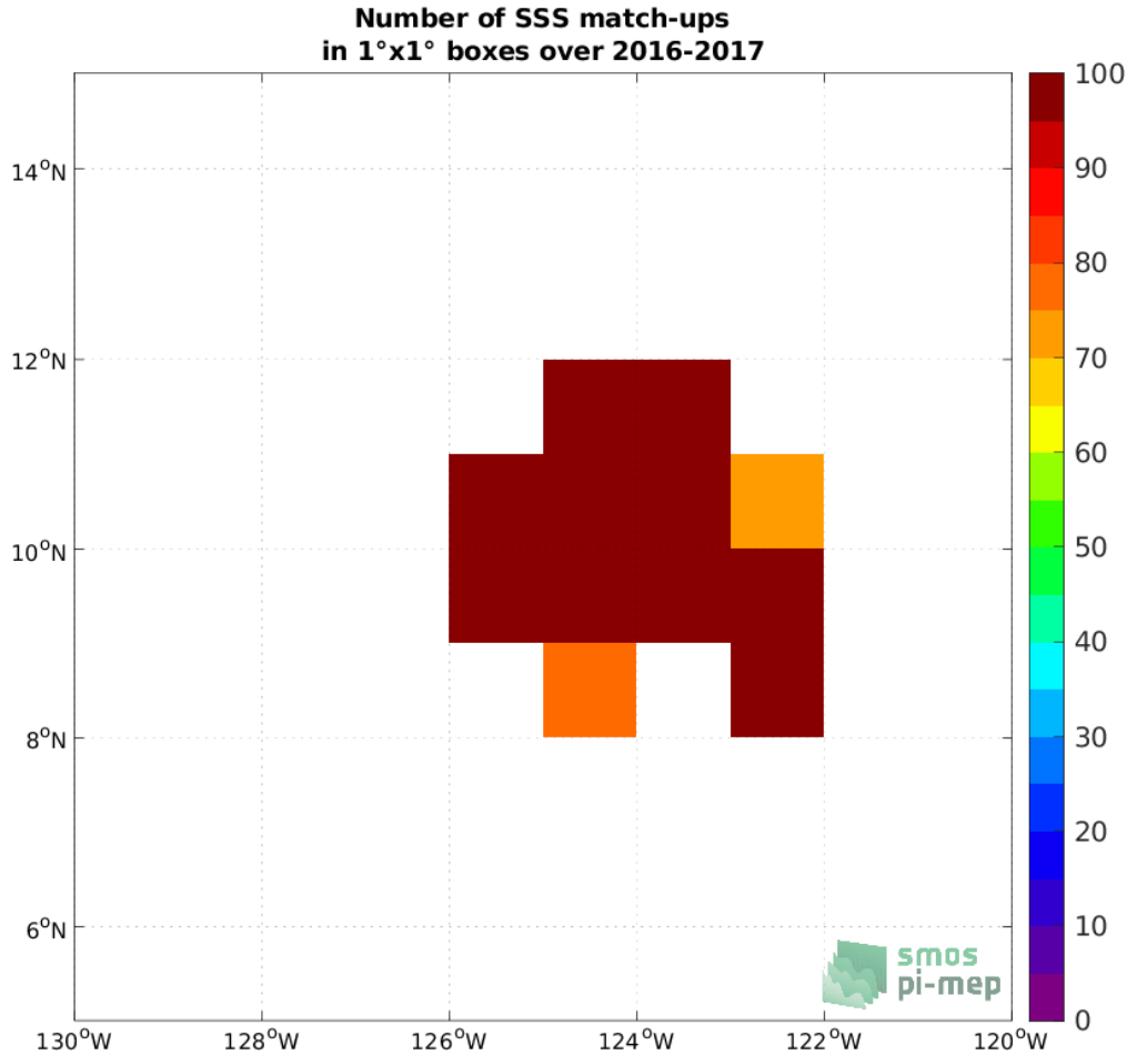
Figure 4: Number of SSS match-ups between Seaglider SSS and the SMOS SSS L2Q v330 - 0.25 Deg (CATDS-CPDC) SSS product for the SPURS 2 Pi-MEP region over 1^\circ \times 1^\circ boxes and for the full satellite product period.
