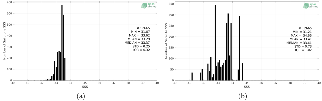
Figure 2: Histograms of SSS from Saildrone (a) and SMOS SSS L2Q v330 - 0.25 Deg (CATDS-CPDC) (b) considering all match-up pairs per bins of 0.1 over the SPURS 2 Pi-MEP region and for the full satellite product period.
