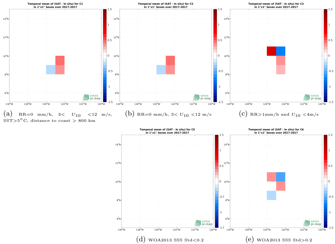
Figure 12: Temporal mean gridded over spatial boxes of size 1^\circ \times 1^\circ of \Delta SSS (SMOS SSS L2Q v330 - 0.25 Deg (CATDS-CPDC) - Saildrone) for 5 different subdatasets corresponding to:RR=0 mm/h, 3 < U_{10} < 12 m/s, SST >5^\circ C, distance to coast > 800 km (a), RR=0 mm/h, 3 < U_{10} < 12 m/s (b), RR >1 mm/h and U_{10} < 4 m/s (c), WOA2013 SSS Std <0.2 (d), WOA2013 SSS Std >0.2 (e).
