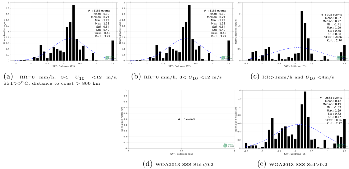
Figure 13: Normalized histogram of \Delta SSS (SMOS SSS L2Q v330 - 0.25 Deg (CATDS-CPDC) - Saildrone) for 5 different subdatasets corresponding to: RR=0 mm/h, 3 < U_{10} < 12 m/s, SST > 5°C, distance to coast > 800 km (a), RR=0 mm/h, 3 < U_{10} < 12 m/s (b), RR > 1mm/h and U_{10} < 4 m/s (c), WOA2013 SSS Std < 0.2 (d), WOA2013 SSS Std > 0.2 (e).
