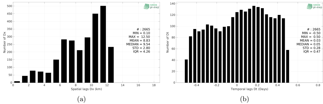
Figure 5: Histograms of the spatial (a) and temporal (b) lags between the location/time of the Saildrone measurement and the date of the corresponding SMOS SSS L2Q v330 - 0.25 Deg (CATDS-CPDC) SSS pixel.
