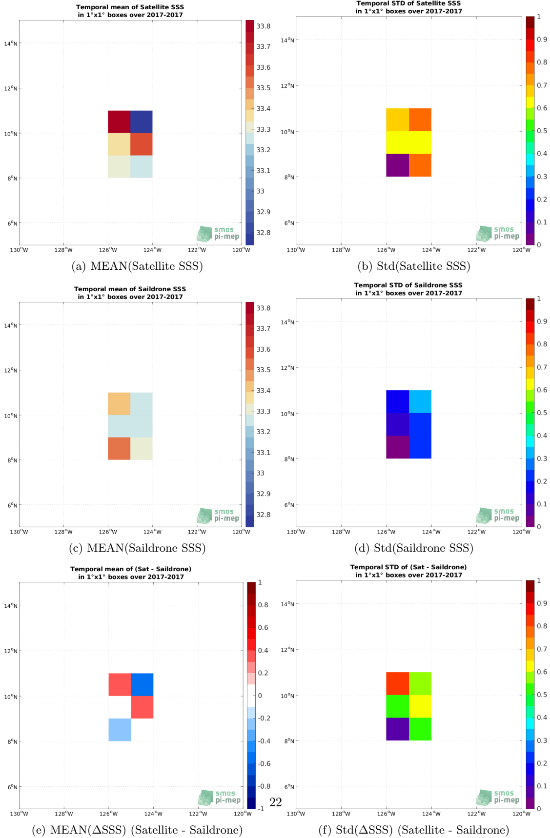
Figure 6: Temporal mean (left) and Std (right) of SSS from SMOS SSS L2Q v330 - 0.25 Deg (CATDS-CPDC) (top), Saildrone (middle), and of \Delta SSS (Satellite - Saildrone). Only match-up pairs are used to generate these maps.
