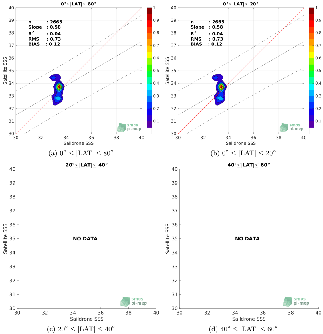
Figure 9: Contour maps of the concentration of SMOS SSS L2Q v330 - 0.25 Deg (CATDS-CPDC) SSS (y-axis) versus Sailldrone SSS (x-axis) at match-up pairs for different latitude bands. For each plot, the red line shows x=y . The black thin and dashed lines indicate a linear fit through the data cloud and the \pm 95\% confidence levels, respectively. The number match-up pairs n , the slope and R^2 coefficient of the linear fit, the root mean square (RMS) and the mean bias between satellite and in situ data are indicated for each latitude band in each plots.
