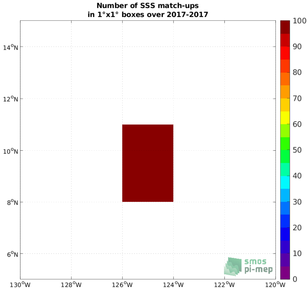
Figure 4: Number of SSS match-ups between Saildrone SSS and the SMOS SSS L2Q v330 - 0.25 Deg (CATDS-CPDC) SSS product for the SPURS 2 Pi-MEP region over 1^\circ \times 1^\circ boxes and for the full satellite product period.
