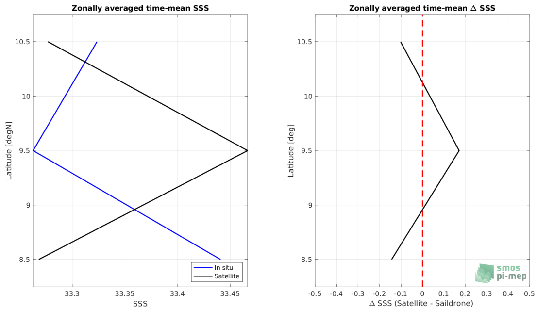
Figure 8: Left panel: Zonal mean SSS from SMOS SSS L2Q v330 - 0.25 Deg (CATDS-CPDC) satellite product (black) and from Sairdrone (blue). Right panel: Zonal mean of \Delta SSS (Satellite - Sairdrone) for all the collected Pi-MEP match-up pairs estimated over the full satellite product period.
