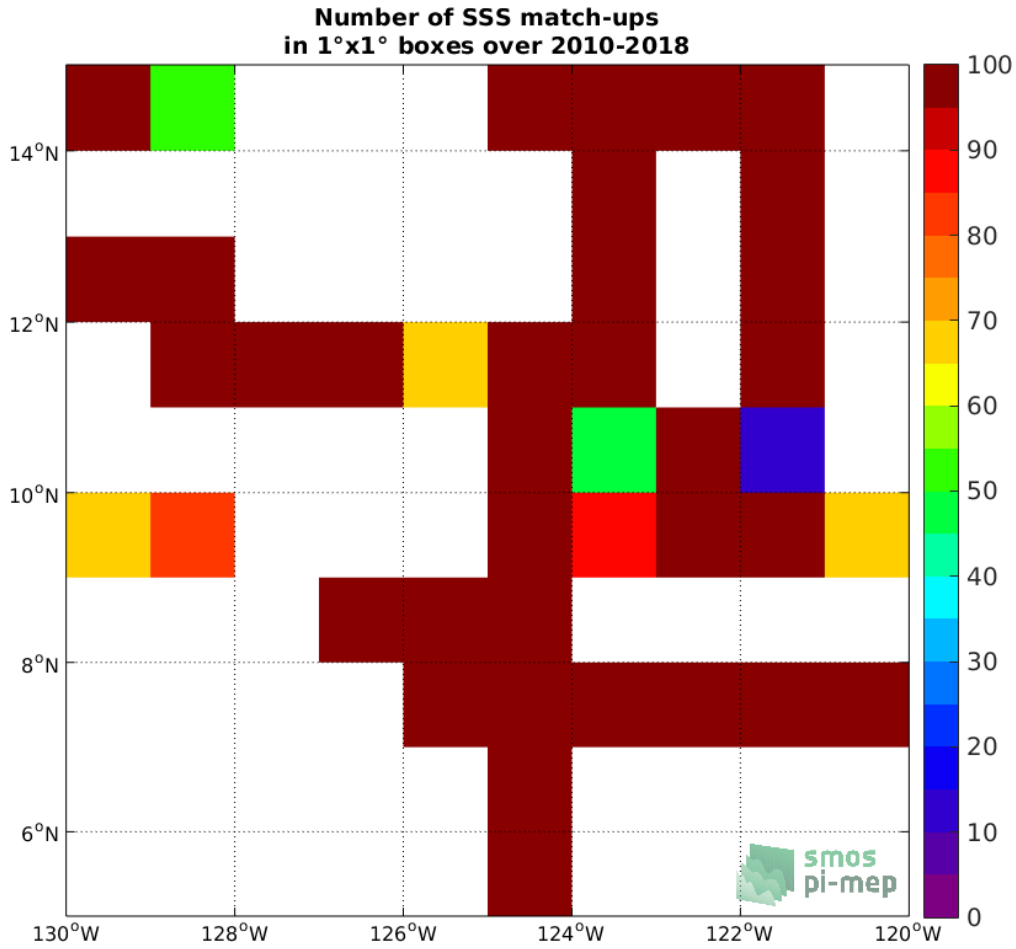
Figure 4: Number of SSS match-ups between TSG (SAMOS) SSS and the SMOS SSS L2Q v321 - 0.25 Deg (CATDS-CPDC) SSS product for the SPURS 2 Pi-MEP region over 1°×1° boxes and for the full satellite product period.
