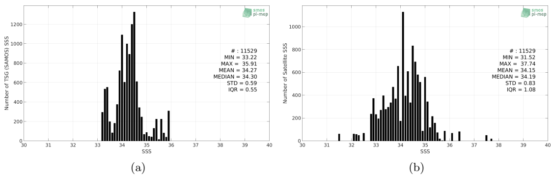
Figure 2: Histograms of SSS from TSG (SAMOS) (a) and SMOS SSS L2Q v321 - 0.25 Deg (CATDS-CPDC) (b) considering all match-up pairs per bins of 0.1 over the SPURS 2 Pi-MEP region and for the full satellite product period.
