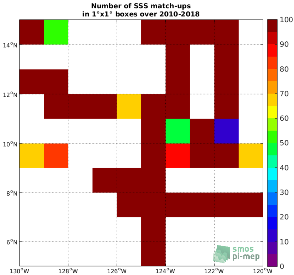
Figure 4: Number of SSS match-ups between TSG (SAMOS) SSS and the SMOS SSS L2Q v321 - 0.25 Deg (CATDS-CPDC) SSS product for the SPURS 2 Pi-MEP region over 1°x1° boxes and for the full satellite product period.
