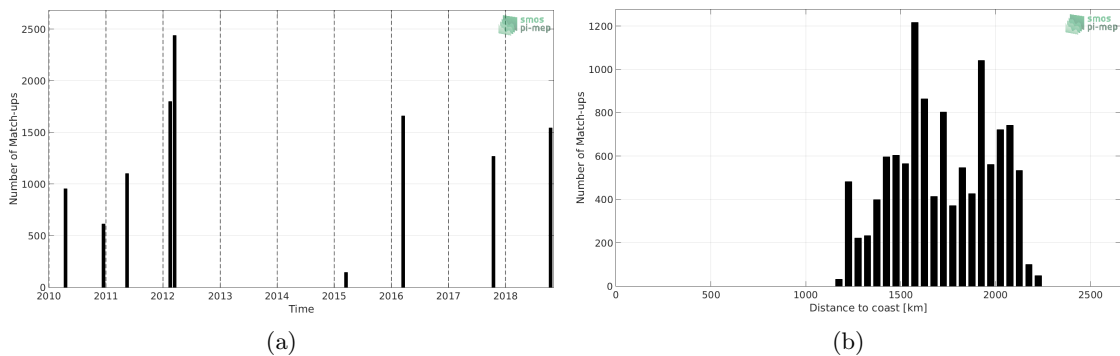
Figure 1: Number of match-ups between TSG (SAMOS) and SMOS SSS L2Q v321 - 0.25 Deg (CATDS-CPDC) SSS as a function of time (a) and as function of the distance to coast (b) over the SPURS 2 Pi-MEP region and for the full satellite product period.
