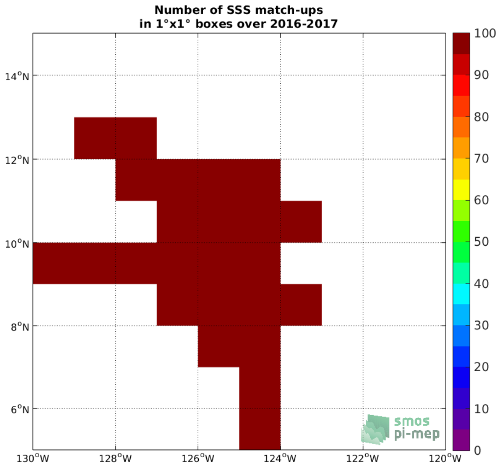
Figure 3: Number of SSS match-ups between Salinity Snake SSS and the SMOS SSS L2Q v321 - 0.25 Deg (CATDS-CPDC) SSS product for the SPURS 2 Pi-MEP region over 1°×1° boxes and for the full satellite product period.
