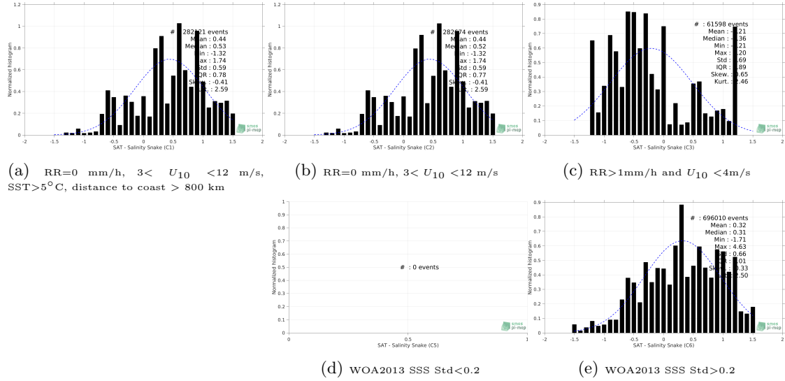
Figure 12: Normalized histogram of \Delta SSS (SMOS SSS L2Q v321 - 0.25 Deg (CATDS-CPDC) - Salinity Snake) for 5 different subdatasets corresponding to: RR=0 mm/h, 3 < U_{10} < 12 m/s, SST > 5°C, distance to coast > 800 km (a), RR=0 mm/h, 3 < U_{10} < 12 m/s (b), RR > 1mm/h and U_{10} < 4 m/s (c), WOA2013 SSS Std < 0.2 (d), WOA2013 SSS Std > 0.2 (e).
