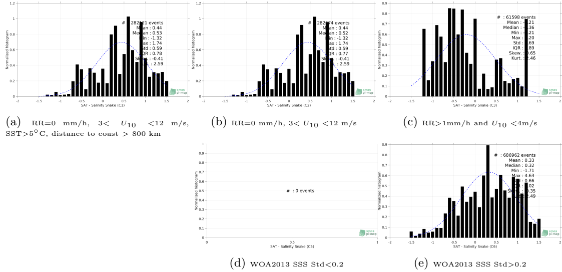
Figure 13: Normalized histogram of \Delta SSS (SMOS SSS L2Q v321 - 0.25 Deg (CATDS-CPDC) - Salinity Snake) for 5 different subdatasets corresponding to: RR=0 mm/h, 3 < U_{10} < 12 m/s, SST > 5°C, distance to coast > 800 km (a), RR=0 mm/h, 3 < U_{10} < 12 m/s (b), RR > 1mm/h and U_{10} < 4 m/s (c), WOA2013 SSS Std < 0.2 (d), WOA2013 SSS Std > 0.2 (e).
