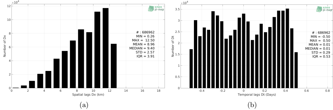
Figure 5: Histograms of the spatial (a) and temporal (b) lags between the time of the Salinity Snake measurements and the date of the corresponding SMOS SSS L2Q v321 - 0.25 Deg (CATDS-CPDC) SSS product.
