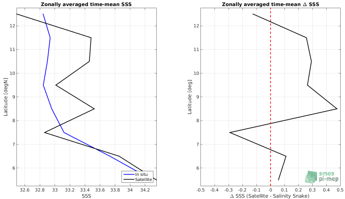
Figure 8: Left panel: Zonal mean SSS from SMOS SSS L2Q v321 - 0.25 Deg (CATDS-CPDC) satellite product (black) and from Salinity Snake (blue). Right panel: Zonal mean of \Delta SSS (Satellite - Salinity Snake) for all the collected Pi-MEP match-up pairs estimated over the full satellite product period.
