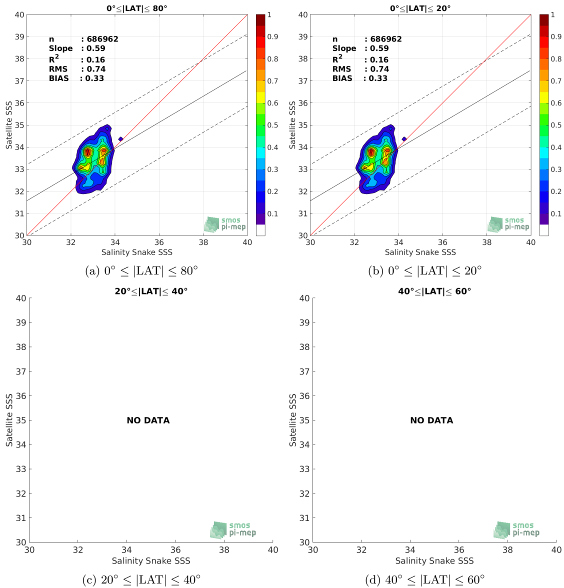
Figure 9: Contour maps of the concentration of SMOS SSS L2Q v321 - 0.25 Deg (CATDS-CPDC) SSS (y-axis) versus Salinity Snake SSS (x-axis) at match-up pairs for different latitude bands. For each plot, the red line shows x=y . The black thin and dashed lines indicate a linear fit through the data cloud and the \pm 95\% confidence levels, respectively. The number match-up pairs n , the slope and R^2 coefficient of the linear fit, the root mean square (RMS) and the mean bias between satellite and in situ data are indicated for each latitude band in each plots.
