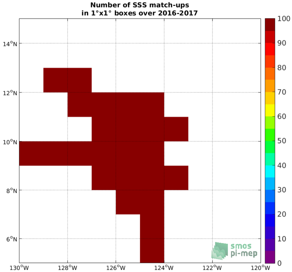
Figure 4: Number of SSS match-ups between Salinity Snake SSS and the SMOS SSS L2Q v321 - 0.25 Deg (CATDS-CPDC) SSS product for the SPURS 2 Pi-MEP region over 1°x1° boxes and for the full satellite product period.
