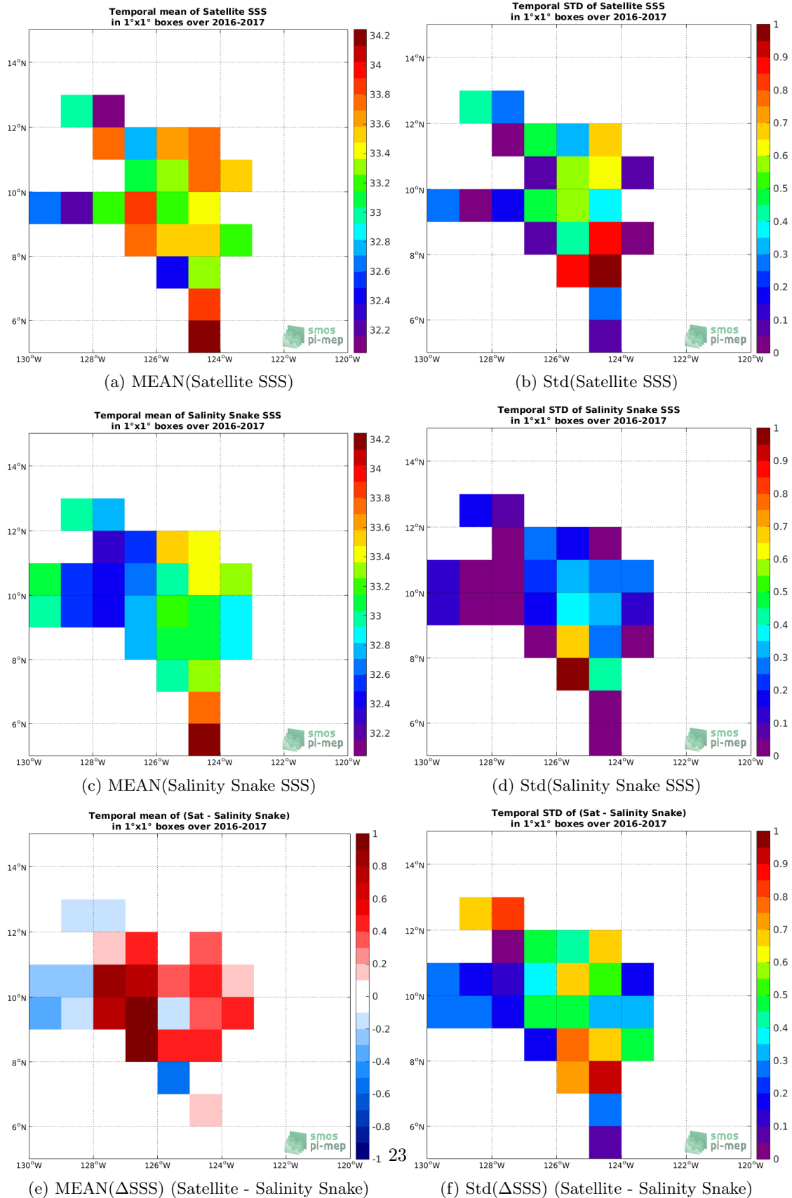
Figure 6: Temporal mean (left) and Std (right) of SSS from SMOS SSS L2Q v321 - 0.25 Deg (CATDS-CPDC) (top), Salinity Snake (middle), and of \Delta SSS (Satellite - Salinity Snake). Only match-up pairs are used to generate these maps.
