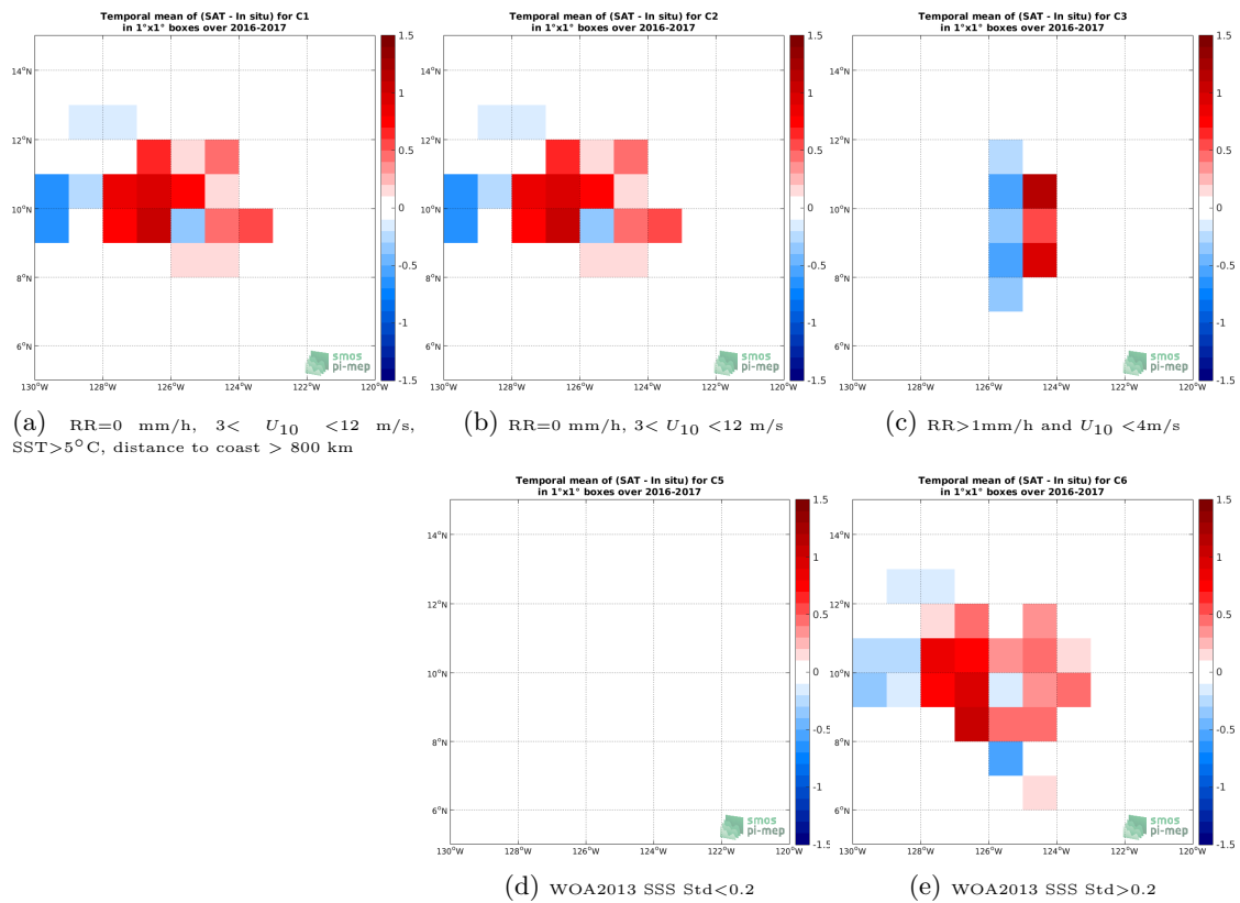
Figure 12: Temporal mean gridded over spatial boxes of size 1^\circ \times 1^\circ of \Delta SSS (SMOS SSS L2Q v321 - 0.25 Deg (CATDS-CPDC) - Salinity Snake) for 5 different subdatasets corresponding to:RR=0 mm/h, 3 < U_{10} < 12 m/s, SST >5^\circ\text{C} , distance to coast > 800 km (a), RR=0 mm/h, 3 < U_{10} < 12 m/s (b), RR >1 mm/h and U_{10} < 4 m/s (c), WOA2013 SSS Std <0.2 (d), WOA2013 SSS Std >0.2 (e).
