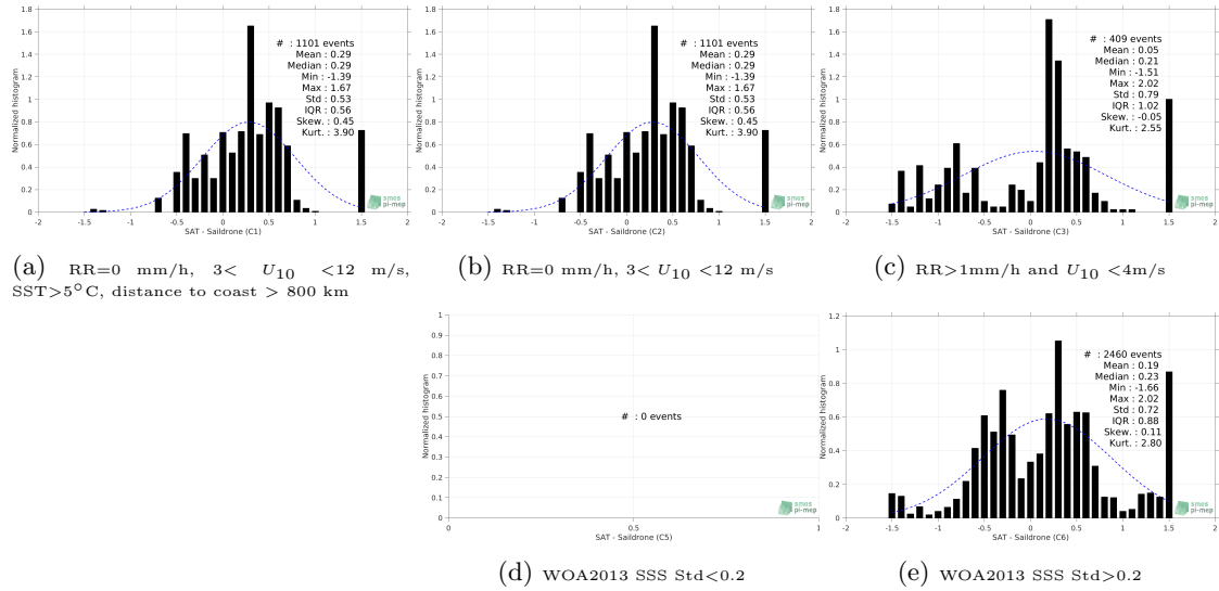
Figure 12: Normalized histogram of \Delta SSS (SMOS SSS L2Q v321 - 0.25 Deg (CATDS-CPDC) - Saildrone) for 5 different subdatasets corresponding to: RR=0 mm/h, 3 < U_{10} < 12 m/s, SST > 5°C, distance to coast > 800 km (a), RR=0 mm/h, 3 < U_{10} < 12 m/s (b), RR > 1mm/h and U_{10} < 4 m/s (c), WOA2013 SSS Std < 0.2 (d), WOA2013 SSS Std > 0.2 (e).
