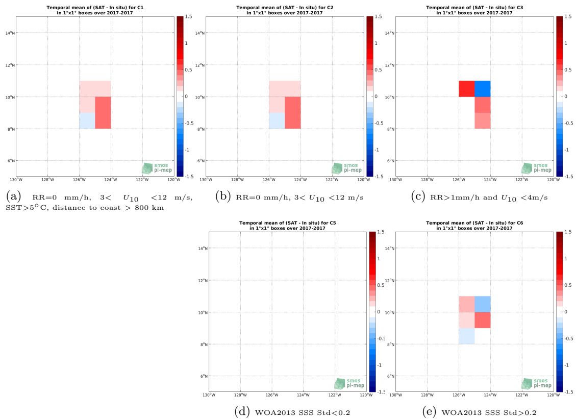
Figure 11: Temporal mean gridded over spatial boxes of size 1^\circ \times 1^\circ of \Delta SSS (SMOS SSS L2Q v321 - 0.25 Deg (CATDS-CPDC) - Saildrone) for 5 different subdatasets corresponding to:RR=0 mm/h, 3 < U_{10} < 12 m/s, SST >5^\circ C, distance to coast > 800 km (a), RR=0 mm/h, 3 < U_{10} < 12 m/s (b), RR >1 mm/h and U_{10} < 4 m/s (c), WOA2013 SSS Std <0.2 (d), WOA2013 SSS Std >0.2 (e).
