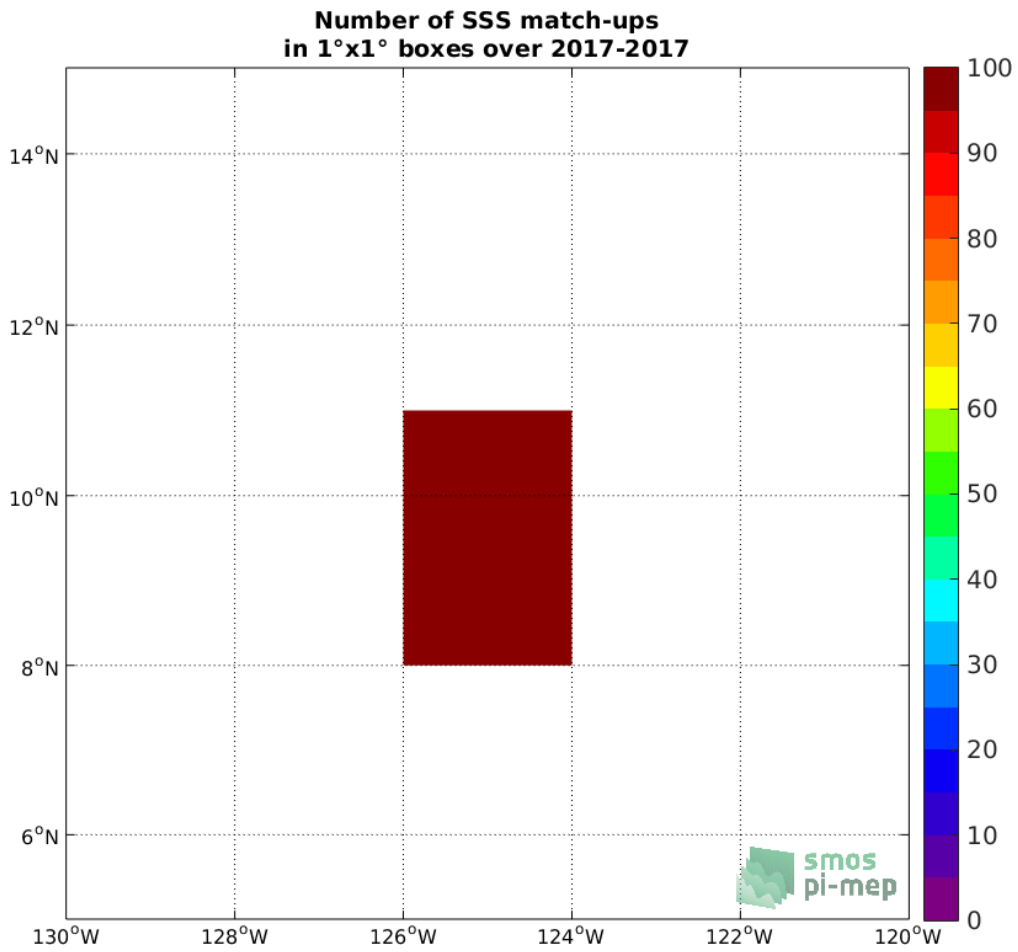
Figure 3: Number of SSS match-ups between Sairdrone SSS and the SMOS SSS L2Q v321 - 0.25 Deg (CATDS-CPDC) SSS product for the SPURS 2 Pi-MEP region over 1°x1° boxes and for the full satellite product period.
