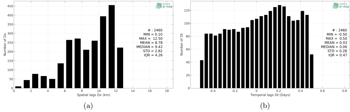
Figure 4: Histograms of the spatial (a) and temporal (b) lags between the location/time of the Saildrone measurement and the date of the corresponding SMOS SSS L2Q v321 - 0.25 Deg (CATDS-CPDC) SSS pixel.
