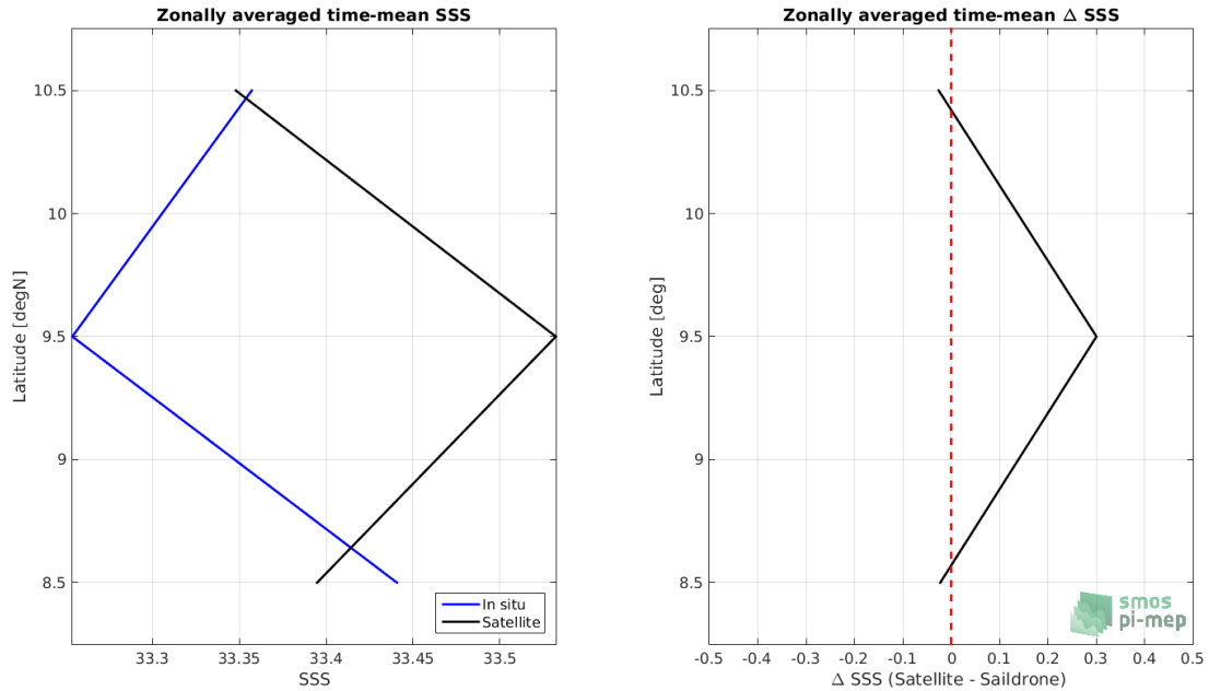
Figure 7: Left panel: Zonal mean SSS from SMOS SSS L2Q v321 - 0.25 Deg (CATDS-CPDC) satellite product (black) and from Sairdrone (blue). Right panel: Zonal mean of \Delta SSS (Satellite - Sairdrone) for all the collected Pi-MEP match-up pairs estimated over the full satellite product period.
