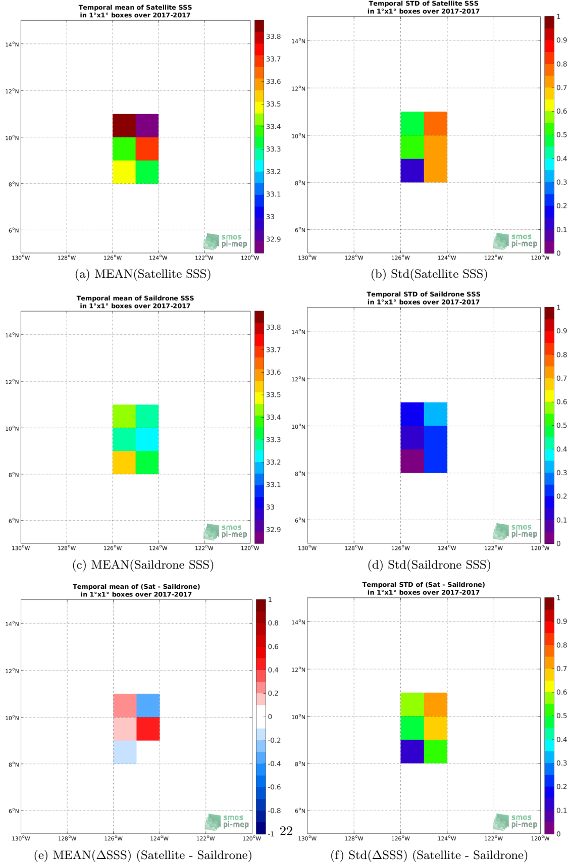
Figure 5: Temporal mean (left) and Std (right) of SSS from SMOS SSS L2Q v321 - 0.25 Deg (CATDS-CPDC) (top), Saildrone (middle), and of \Delta SSS (Satellite - Saildrone). Only match-up pairs are used to generate these maps.
