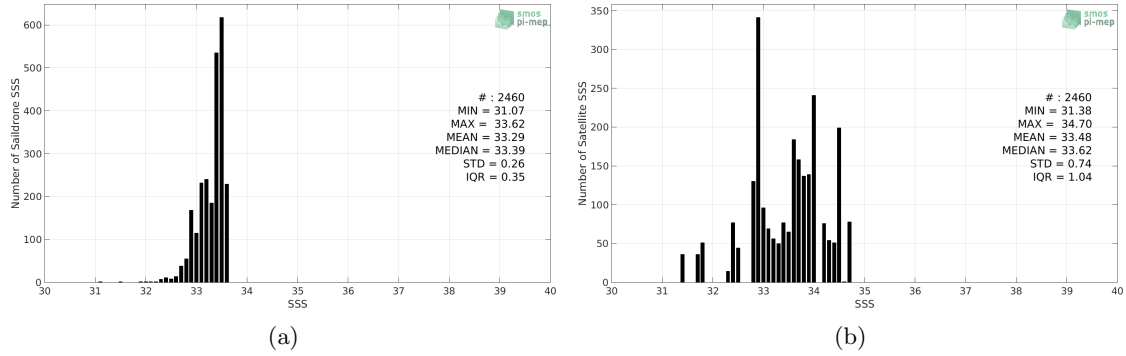
Figure 2: Histograms of SSS from Sairdrone (a) and SMOS SSS L2Q v321 - 0.25 Deg (CATDS-CPDC) (b) considering all match-up pairs per bins of 0.1 over the SPURS 2 Pi-MEP region and for the full satellite product period.
