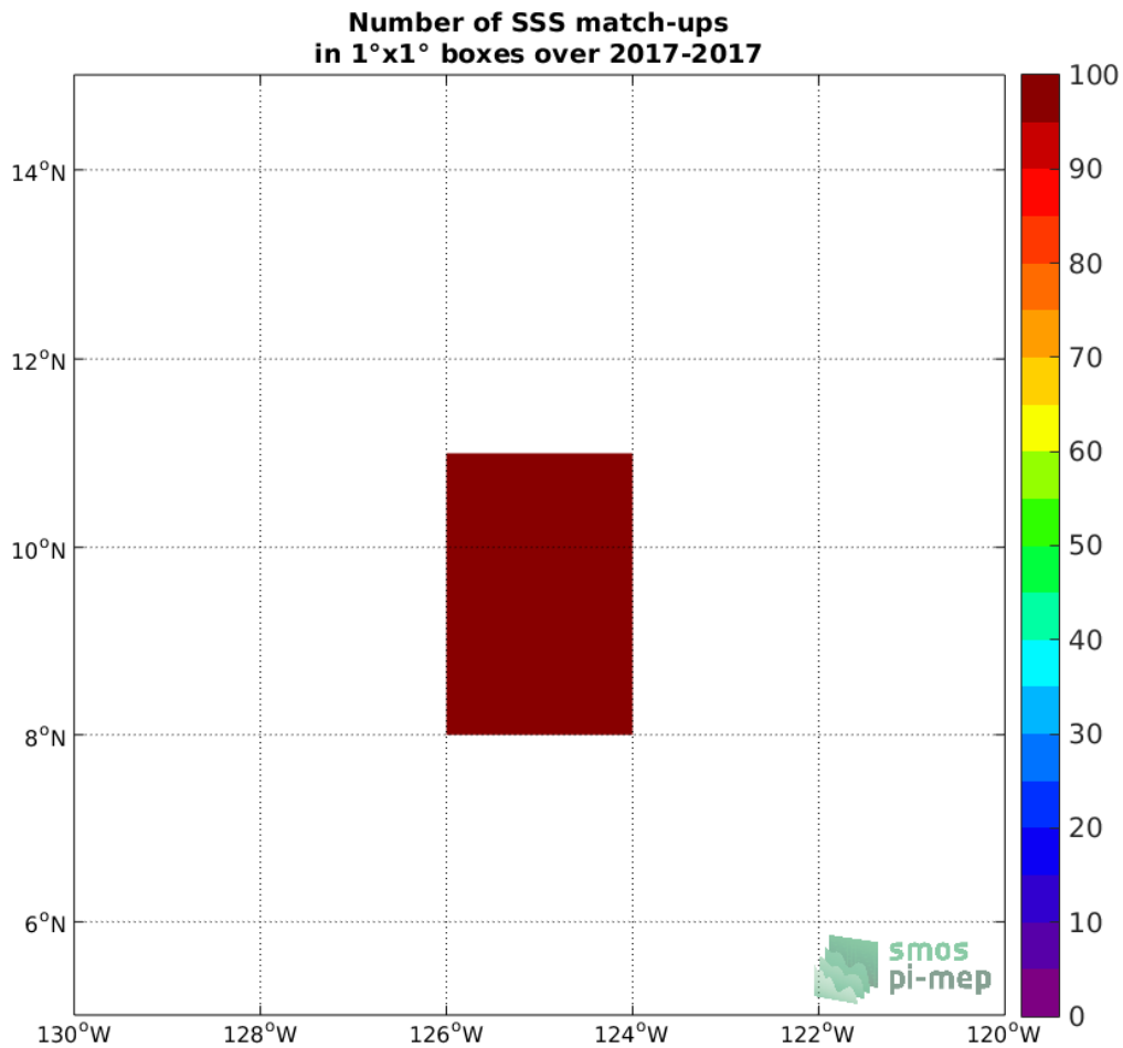
Figure 4: Number of SSS match-ups between Saildrone SSS and the SMOS SSS L2Q v321 - 0.25 Deg (CATDS-CPDC) SSS product for the SPURS 2 Pi-MEP region over 1°x1° boxes and for the full satellite product period.
