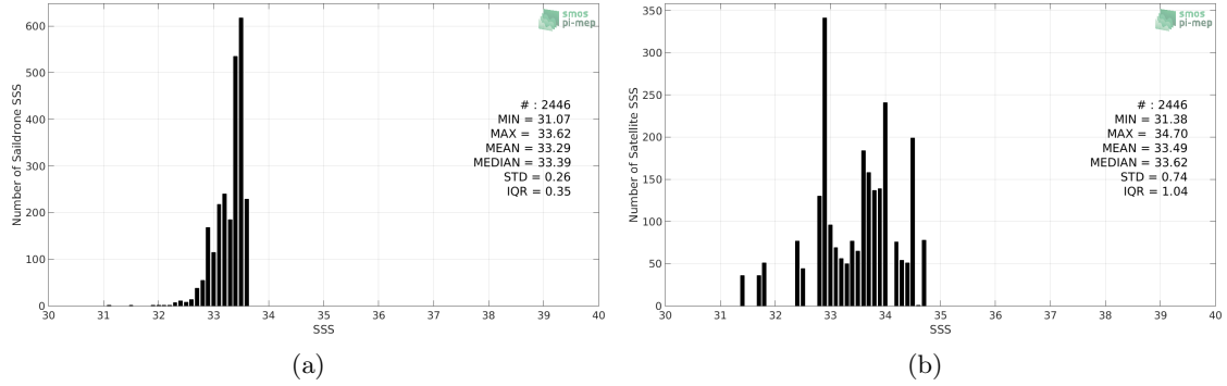
Figure 2: Histograms of SSS from Saildrone (a) and SMOS SSS L2Q v321 - 0.25 Deg (CATDS-CPDC) (b) considering all match-up pairs per bins of 0.1 over the SPURS 2 Pi-MEP region and for the full satellite product period.
