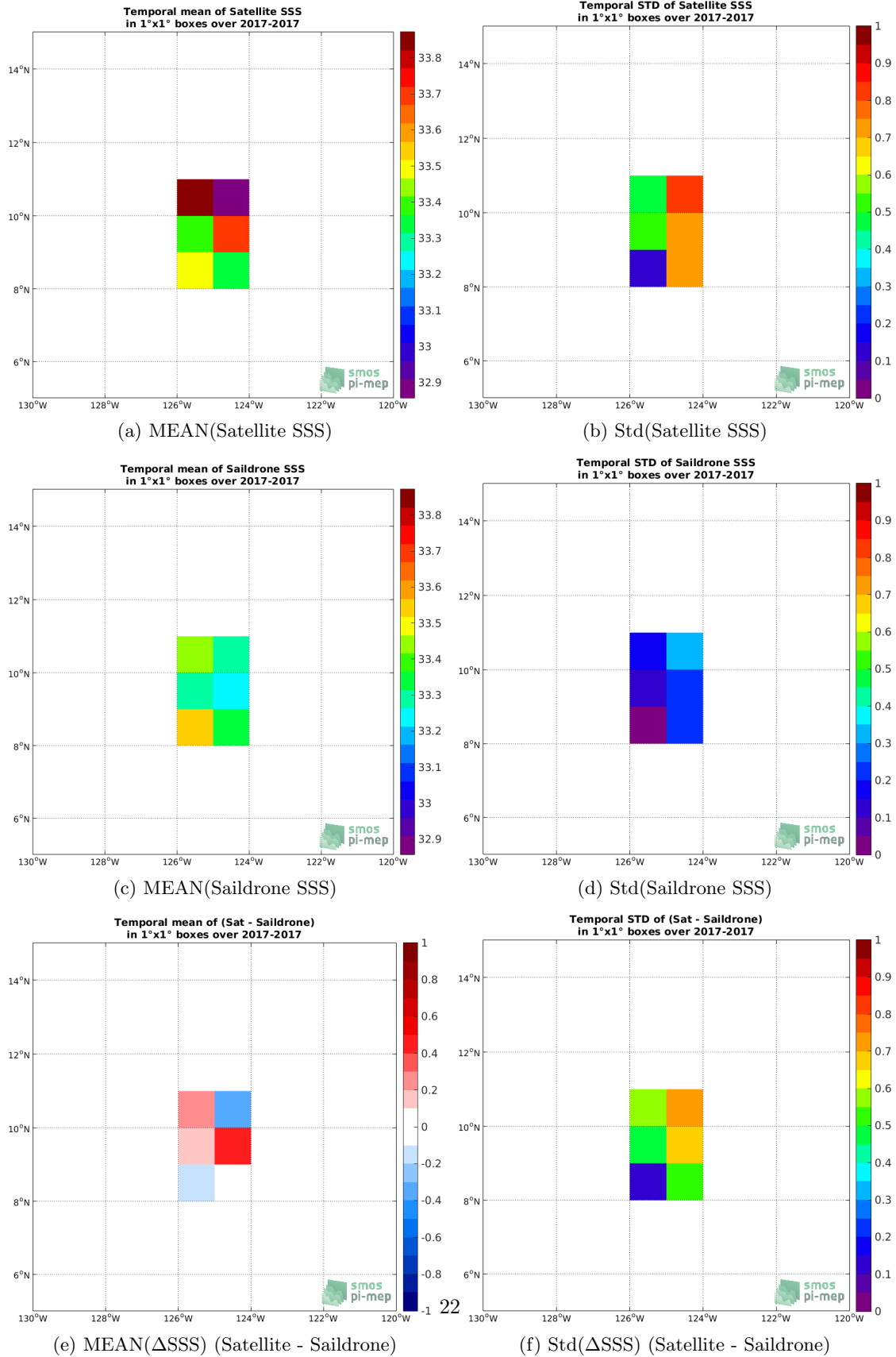
Figure 6: Temporal mean (left) and Std (right) of SSS from SMOS SSS L2Q v321 - 0.25 Deg (CATDS-CPDC) (top), Saildrone (middle), and of \Delta SSS (Satellite - Saildrone). Only match-up pairs are used to generate these maps.
