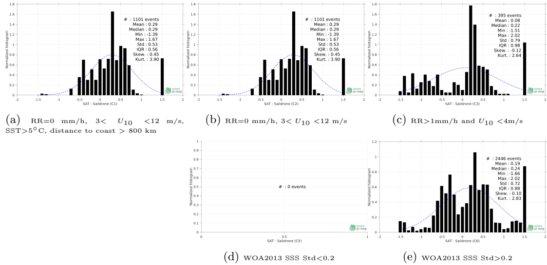
Figure 13: Normalized histogram of \Delta SSS (SMOS SSS L2Q v321 - 0.25 Deg (CATDS-CPDC) - Saildrone) for 5 different subdatasets corresponding to: RR=0 mm/h, 3 < U_{10} < 12 m/s, SST > 5°C, distance to coast > 800 km (a), RR=0 mm/h, 3 < U_{10} < 12 m/s (b), RR > 1mm/h and U_{10} < 4 m/s (c), WOA2013 SSS Std < 0.2 (d), WOA2013 SSS Std > 0.2 (e).
