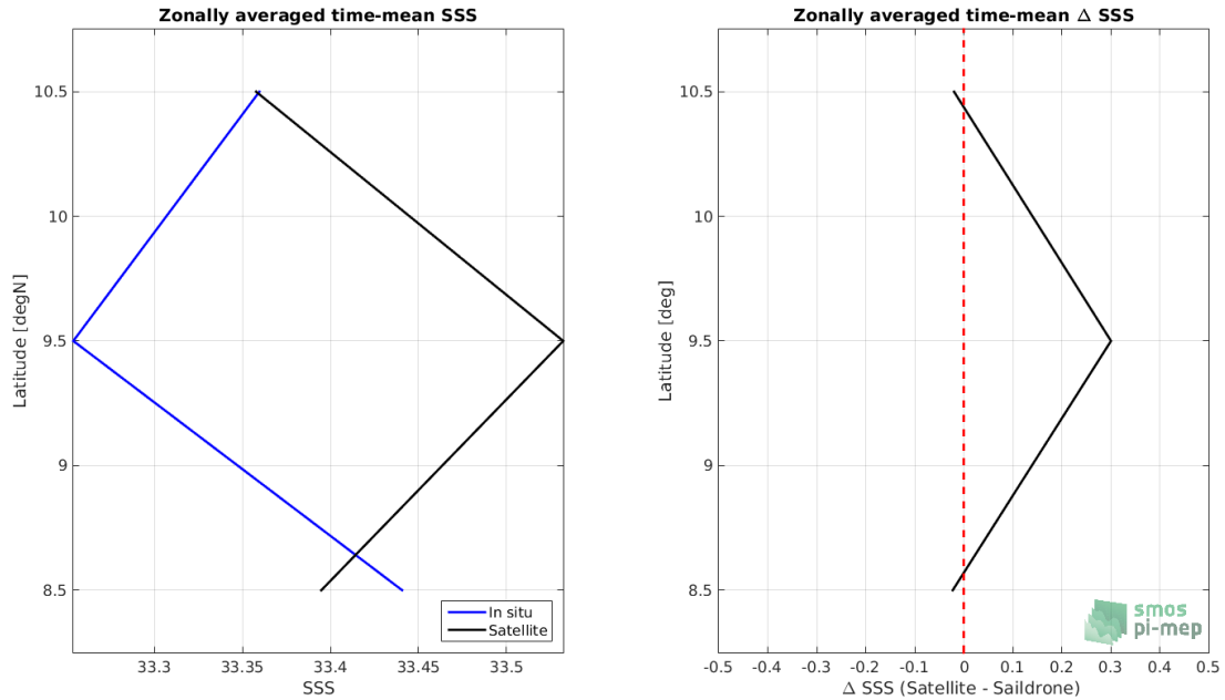
Figure 8: Left panel: Zonal mean SSS from SMOS SSS L2Q v321 - 0.25 Deg (CATDS-CPDC) satellite product (black) and from Sairdrone (blue). Right panel: Zonal mean of \Delta SSS (Satellite - Sairdrone) for all the collected Pi-MEP match-up pairs estimated over the full satellite product period.
