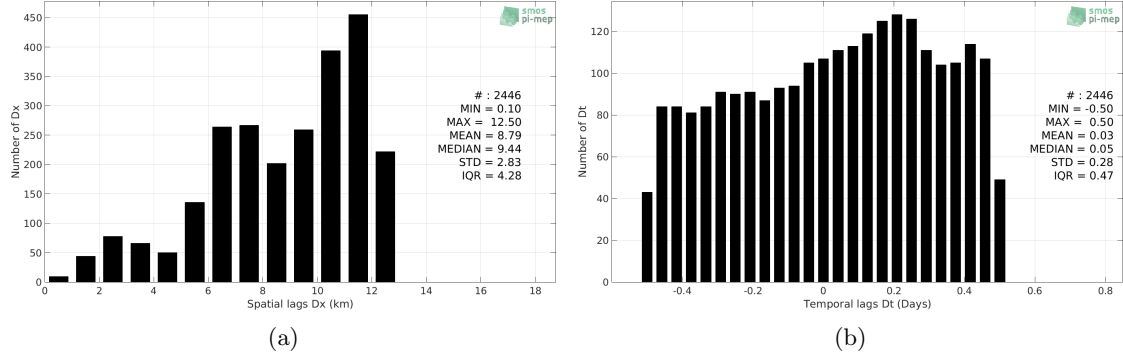
Figure 5: Histograms of the spatial (a) and temporal (b) lags between the time of the Saildrone measurements and the date of the corresponding SMOS SSS L2Q v321 - 0.25 Deg (CATDS-CPDC) SSS product.
