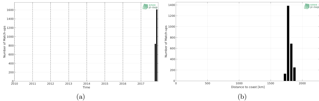
Figure 1: Number of match-ups between Sairdrone and SMOS SSS L2Q v321 - 0.25 Deg (CATDS-CPDC) SSS as a function of time (a) and as function of the distance to coast (b) over the SPURS 2 Pi-MEP region and for the full satellite product period.
