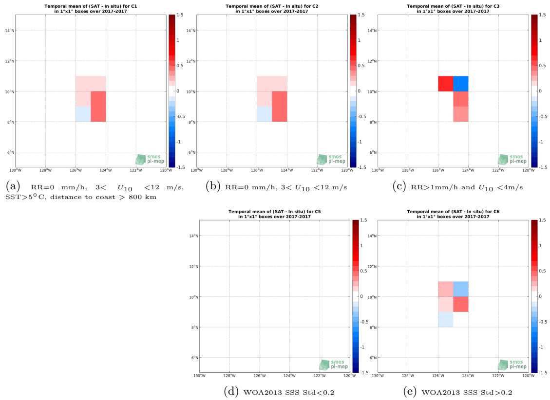
Figure 12: Temporal mean gridded over spatial boxes of size 1^\circ \times 1^\circ of \Delta SSS (SMOS SSS L2Q v321 - 0.25 Deg (CATDS-CPDC) - Saildrone) for 5 different subdatasets corresponding to: RR=0 mm/h, 3 < U_{10} < 12 m/s, SST > 5^\circ C , distance to coast > 800 km (a), RR=0 mm/h, 3 < U_{10} < 12 m/s (b), RR > 1 mm/h and U_{10} < 4 m/s (c), WOA2013 SSS Std < 0.2 (d), WOA2013 SSS Std > 0.2 (e).
