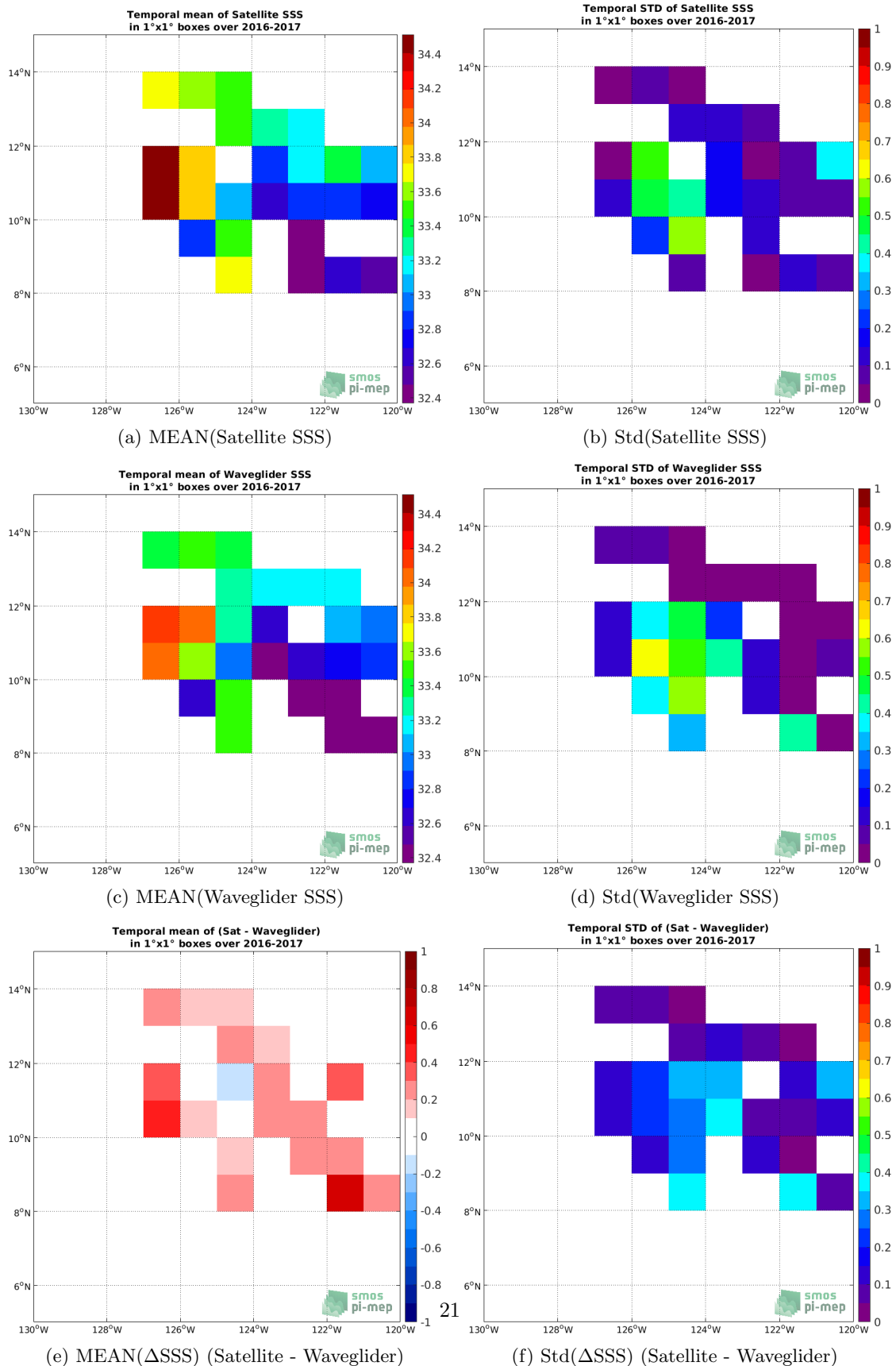
Figure 5: Temporal mean (left) and Std (right) of SSS from SMOS SSS L3 v317 - Monthly - 25 km (CATDS-CPDC) (top), Waveglider (middle), and of \Delta SSS (Satellite - Waveglider). Only match-up pairs are used to generate these maps.
