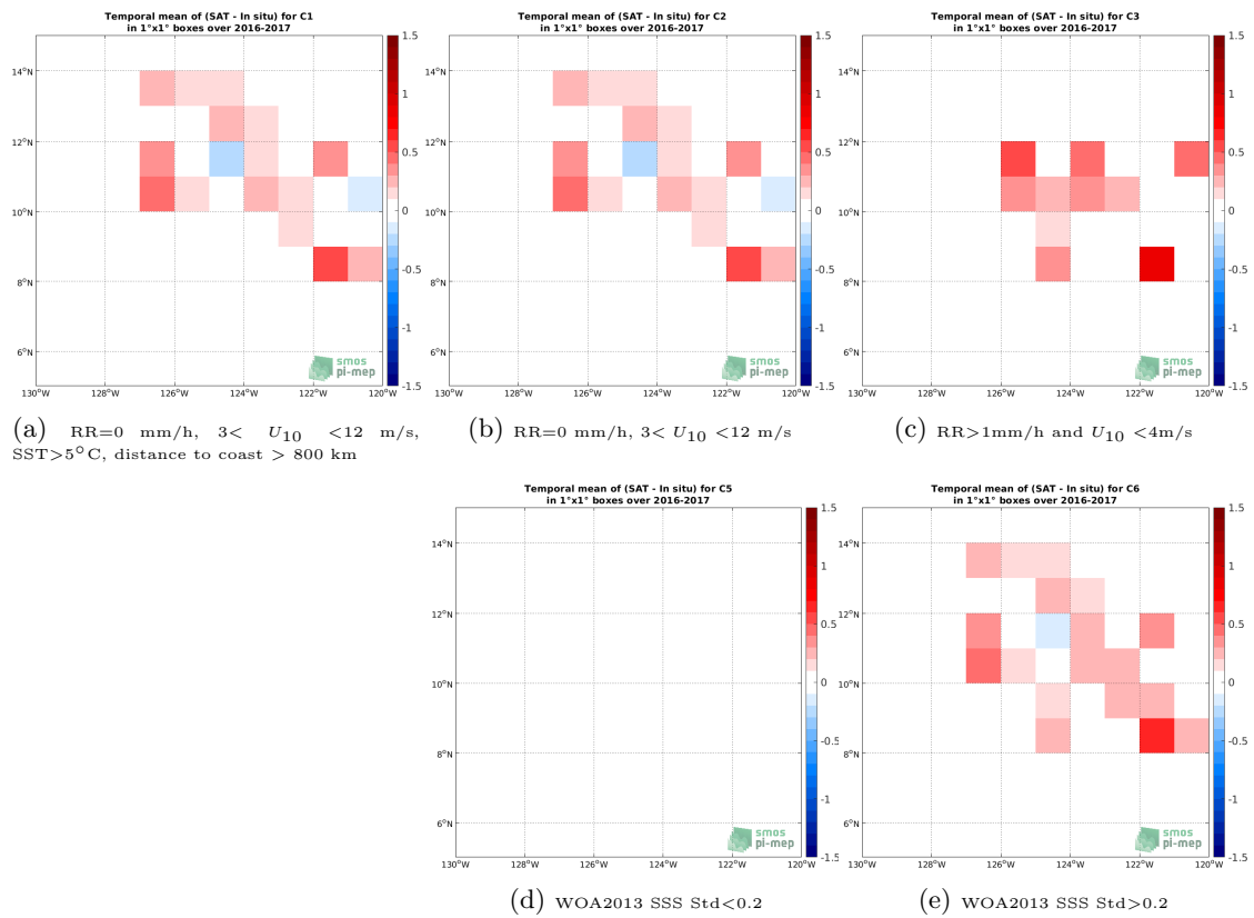
Figure 11: Temporal mean gridded over spatial boxes of size 1^\circ \times 1^\circ of \Delta\text{SSS} (SMOS SSS L3 v317 - Monthly - 25 km (CATDS-CPDC) - Waveglider) for 5 different subdatasets corresponding to:RR=0 mm/h, 3 < U_{10} < 12 m/s, SST >5^\circ\text{C} , distance to coast > 800 km (a), RR=0 mm/h, 3 < U_{10} < 12 m/s (b), RR >1 mm/h and U_{10} < 4 m/s (c), WOA2013 SSS Std <0.2 (d), WOA2013 SSS Std >0.2 (e).
