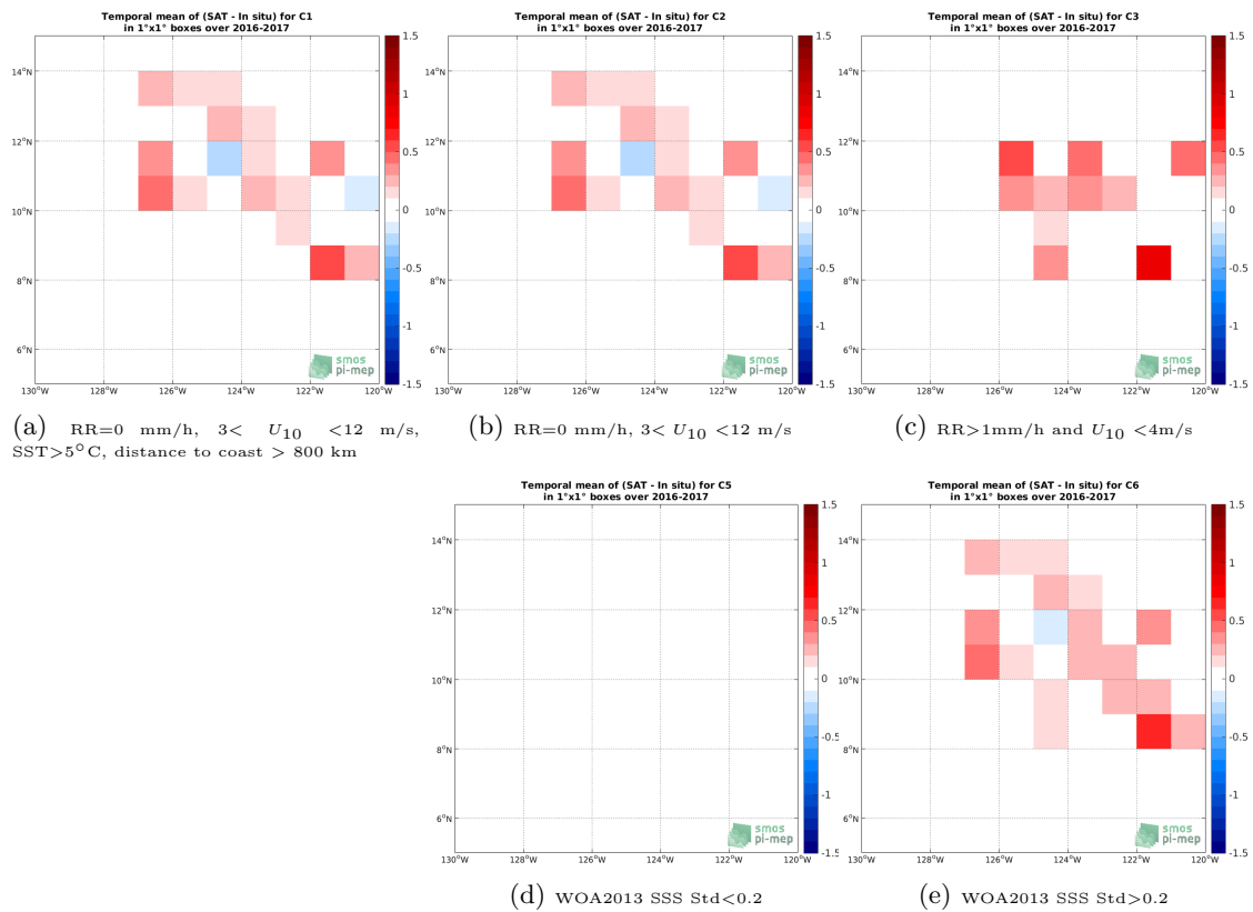
Figure 12: Temporal mean gridded over spatial boxes of size 1^\circ \times 1^\circ of \Delta SSS (SMOS SSS L3 v317 - Monthly - 25 km (CATDS-CPDC) - Waveglider) for 5 different subdatasets corresponding to:RR=0 mm/h, 3 < U_{10} < 12 m/s, SST >5^\circ C, distance to coast > 800 km (a), RR=0 mm/h, 3 < U_{10} < 12 m/s (b), RR >1 mm/h and U_{10} < 4 m/s (c), WOA2013 SSS Std <0.2 (d), WOA2013 SSS Std >0.2 (e).
