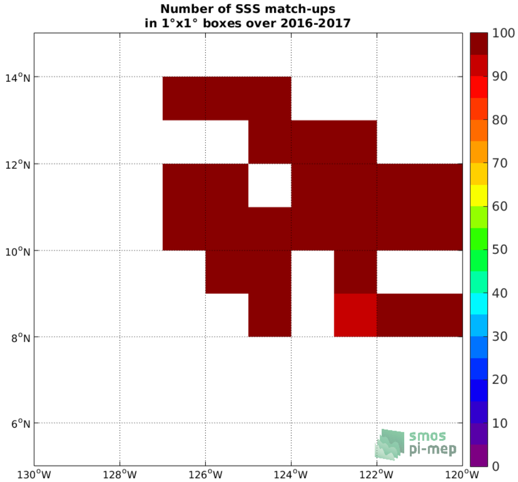
Figure 4: Number of SSS match-ups between Waveglider SSS and the SMOS SSS L3 v317 - Monthly - 25 km (CATDS-CPDC) SSS product for the SPURS 2 Pi-MEP region over 1°x1° boxes and for the full satellite product period.
