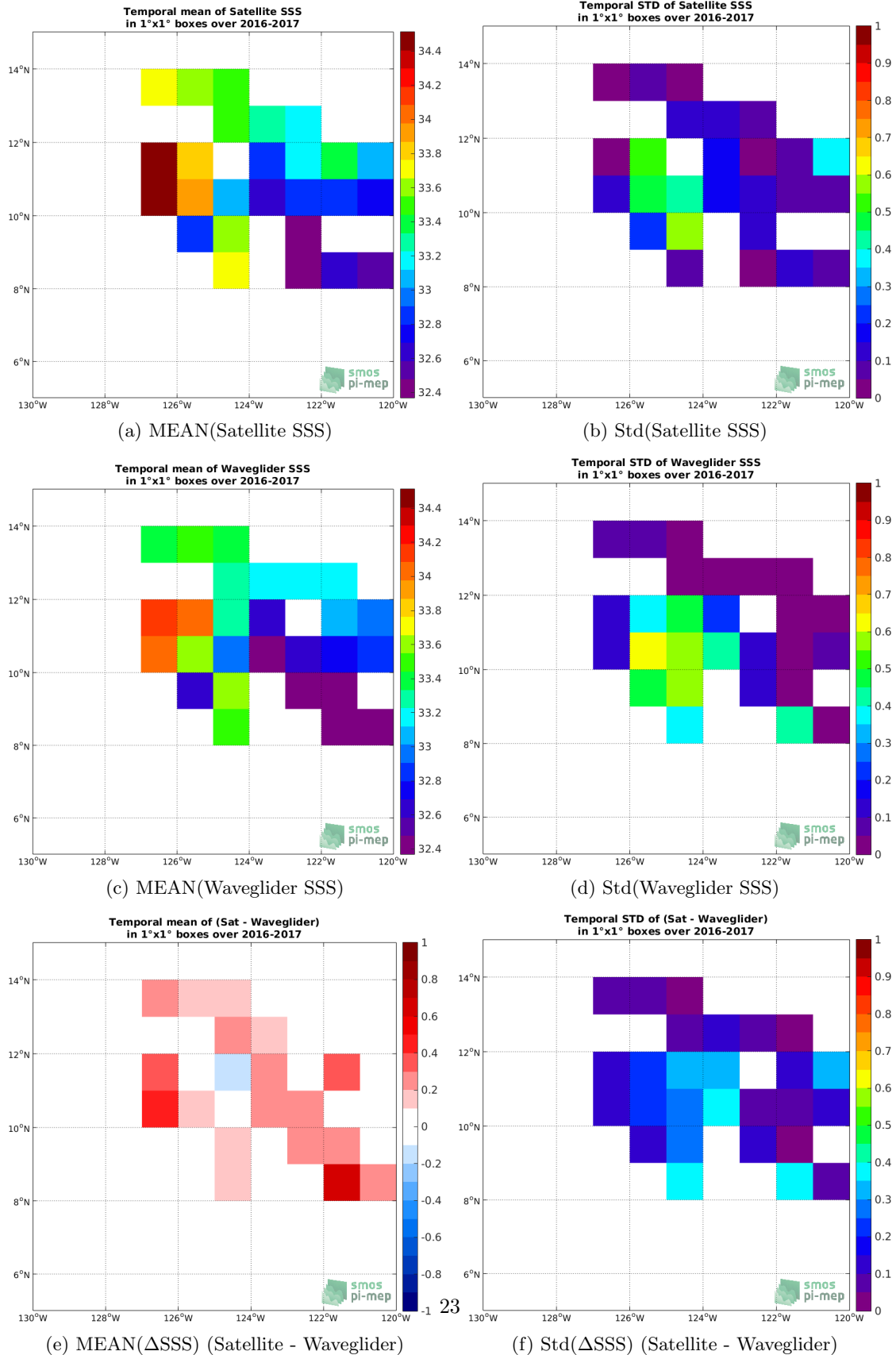
Figure 6: Temporal mean (left) and Std (right) of SSS from SMOS SSS L3 v317 - Monthly - 25 km (CATDS-CPDC) (top), Waveglider (middle), and of \Delta SSS (Satellite - Waveglider). Only match-up pairs are used to generate these maps.
