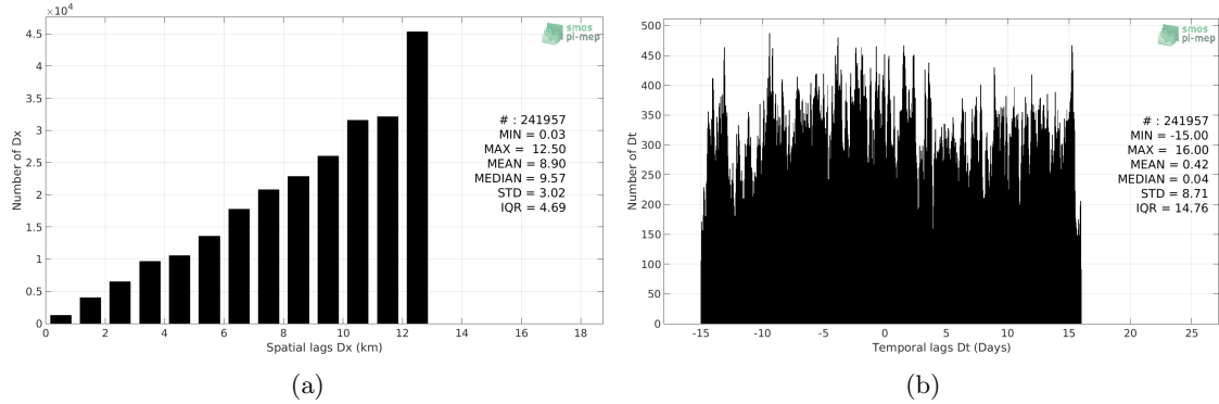
Figure 5: Histograms of the spatial (a) and temporal (b) lags between the time of the Waveglider measurements and the date of the corresponding SMOS SSS L3 v317 - Monthly - 25 km (CATDS-CPDC) SSS product.
