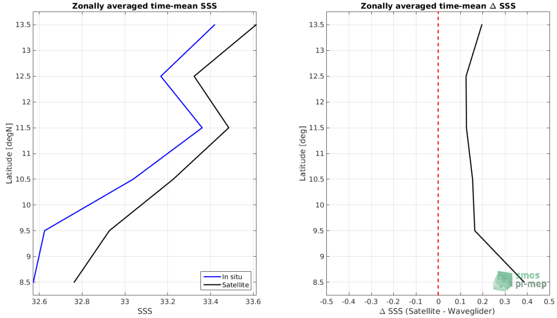
Figure 8: Left panel: Zonal mean SSS from SMOS SSS L3 v317 - Monthly - 25 km (CATDS-CPDC) satellite product (black) and from Waveglider (blue). Right panel: Zonal mean of \Delta SSS (Satellite - Waveglider) for all the collected Pi-MEP match-up pairs estimated over the full satellite product period.
