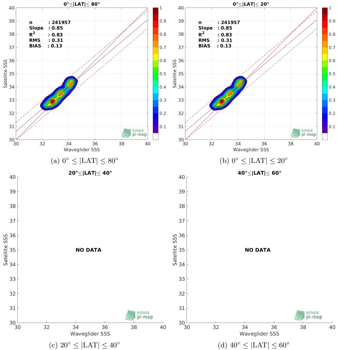
Figure 9: Contour maps of the concentration of SMOS SSS L3 v317 - Monthly - 25 km (CATDS-CPDC) SSS (y-axis) versus Waveglider SSS (x-axis) at match-up pairs for different latitude bands. For each plot, the red line shows x=y . The black thin and dashed lines indicate a linear fit through the data cloud and the \pm 95\% confidence levels, respectively. The number match-up pairs n , the slope and R^2 coefficient of the linear fit, the root mean square (RMS) and the mean bias between satellite and in situ data are indicated for each latitude band in each plots.
