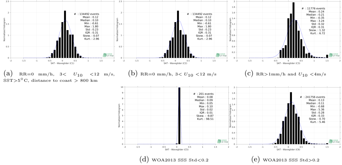
Figure 13: Normalized histogram of \Delta SSS (SMOS SSS L3 v317 - Monthly - 25 km (CATDS-CPDC) - Waveglider) for 5 different subdatasets corresponding to: RR=0 mm/h, 3 < U_{10} < 12 m/s, SST > 5°C, distance to coast > 800 km (a), RR=0 mm/h, 3 < U_{10} < 12 m/s (b), RR > 1mm/h and U_{10} < 4 m/s (c), WOA2013 SSS Std < 0.2 (d), WOA2013 SSS Std > 0.2 (e).
