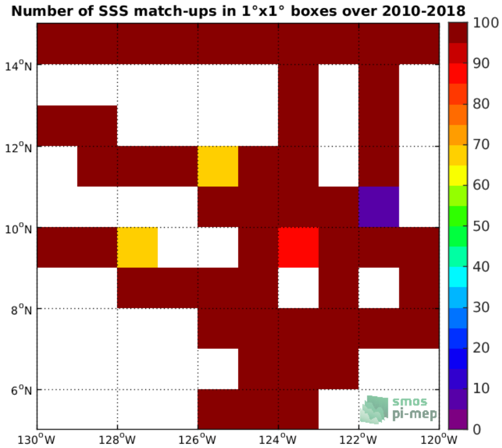
Figure 4: Number of SSS match-ups between TSG-SAMOS SSS and the SMOS-L3-CATDS-CPDC-V317-MONTHLY-25KM SSS product for the SPURS 2 Pi-MEP region over 1°x1° boxes and for the full satellite product period.
