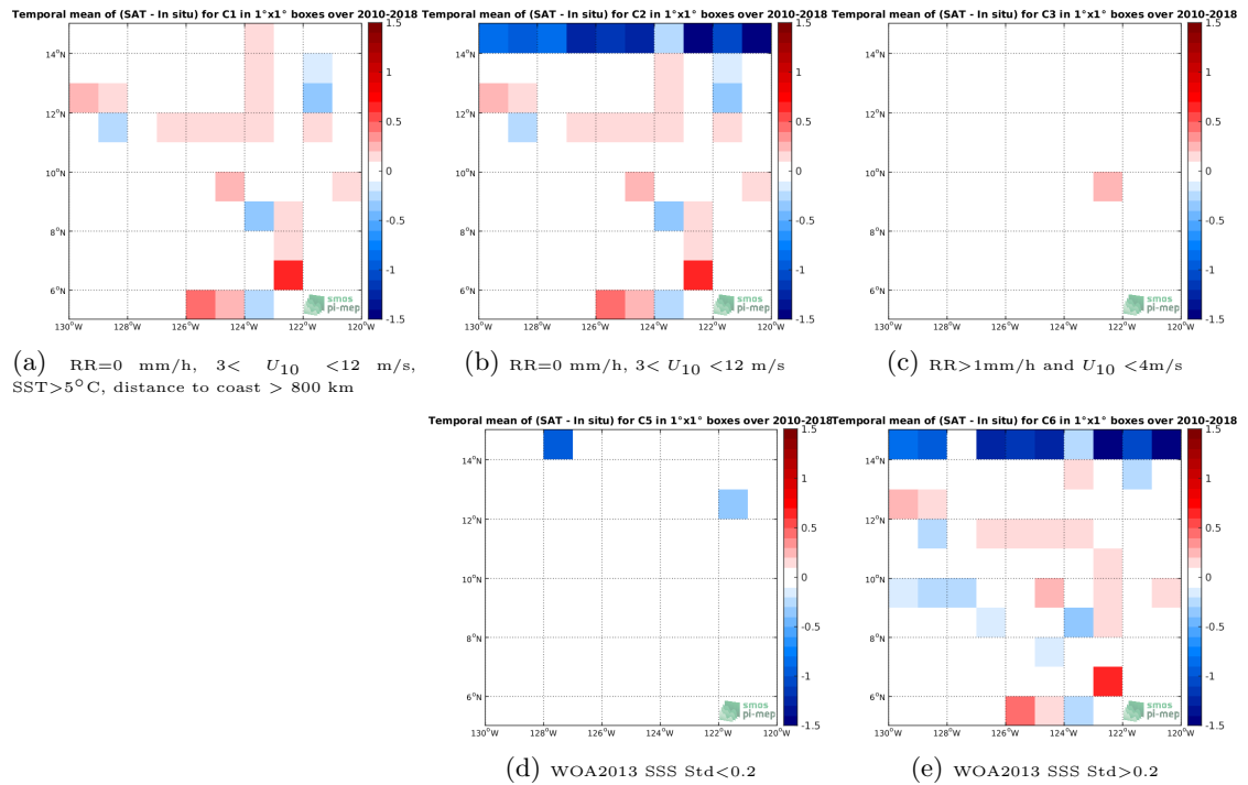
Figure 12: Temporal mean gridded over spatial boxes of size 1^\circ \times 1^\circ of \Delta SSS (SMOS-L3-CATDS-CPDC-V317-MONTHLY-25KM - TSG-SAMOS) for 5 different subdatasets corresponding to: RR=0 mm/h, 3 < U_{10} < 12 m/s, SST > 5^\circ C , distance to coast > 800 km (a), RR=0 mm/h, 3 < U_{10} < 12 m/s (b), RR > 1 mm/h and U_{10} < 4 m/s (c), WOA2013 SSS Std < 0.2 (d), WOA2013 SSS Std > 0.2 (e).
