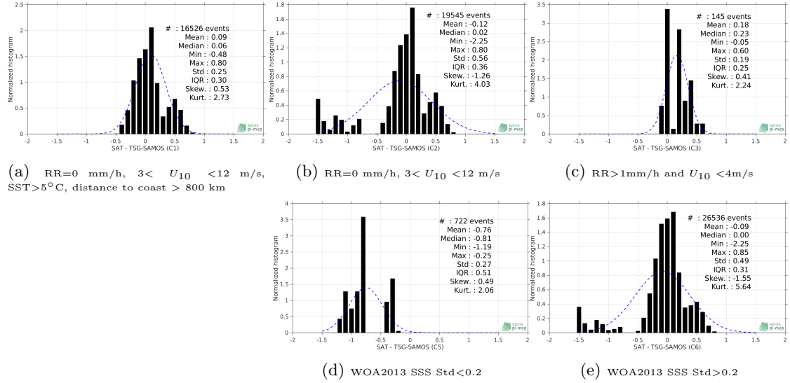
Figure 13: Normalized histogram of \Delta\text{SSS} (SMOS-L3-CATDS-CPDC-V317-MONTHLY-25KM - TSG-SAMOS) for 5 different subdatasets corresponding to: RR=0 mm/h, 3 < U_{10} < 12 m/s, SST>5°C, distance to coast > 800 km (a), RR=0 mm/h, 3 < U_{10} < 12 m/s (b), RR>1mm/h and U_{10} < 4 m/s (c), WOA2013 SSS Std<0.2 (d), WOA2013 SSS Std>0.2 (e).
