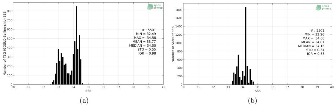
Figure 2: Histograms of SSS from TSG (GOSUD-Sailing-ship) (a) and SMOS SSS L3 v317 - Monthly - 25 km (CATDS-CPDC) (b) considering all match-up pairs per bins of 0.1 over the SPURS 2 Pi-MEP region and for the full satellite product period.
