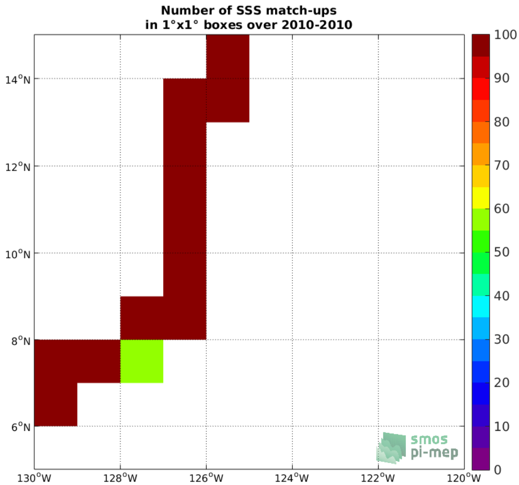
Figure 4: Number of SSS match-ups between TSG (GOSUD-Sailing-ship) SSS and the SMOS SSS L3 v317 - Monthly - 25 km (CATDS-CPDC) SSS product for the SPURS 2 Pi-MEP region over 1°x1° boxes and for the full satellite product period.
