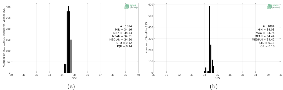
Figure 2: Histograms of SSS from TSG-GOSUD-Research-vessel (a) and SMOS-L3-CATDS-CPDC-V317-MONTHLY-25KM (b) considering all match-up pairs per bins of 0.1 over the SPURS 2 Pi-MEP region and for the full satellite product period.
