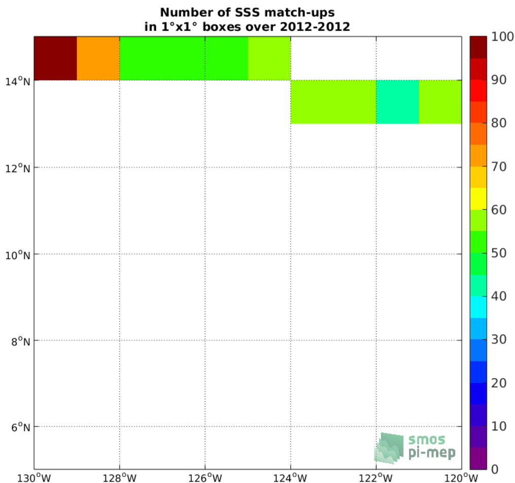
Figure 4: Number of SSS match-ups between TSG-GOSUD-Research-vessel SSS and the SMOS-L3-CATDS-CPDC-V317-MONTHLY-25KM SSS product for the SPURS 2 Pi-MEP region over 1°x1° boxes and for the full satellite product period.
