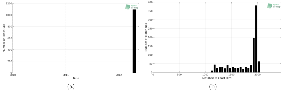
Figure 1: Number of match-ups between TSG-GOSUD-Research-vessel and SMOS-L3-CATDS-CPDC-V317-MONTHLY-25KM SSS as a function of time (a) and as function of the distance to coast (b) over the SPURS 2 Pi-MEP region and for the full satellite product period.
