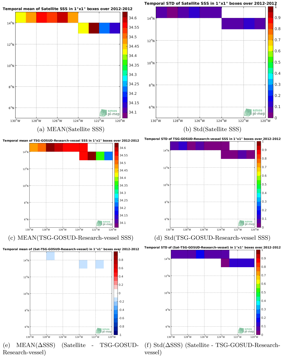
Figure 6: Temporal mean (left) and Std (right) of SSS from SMOS-L3-CATDS-CPDC-V317-MONTHLY-25KM (top), TSG-GOSUD-Research-vessel (middle), and of \Delta SSS (Satellite - TSG-GOSUD-Research-vessel). Only match-up pairs are used to generate these maps.
