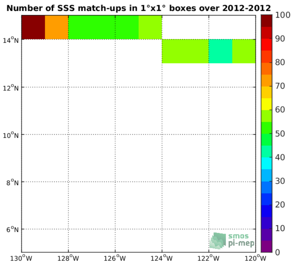
Figure 4: Number of SSS match-ups between TSG-GOSUD-Research-vessel SSS and the SMOS-L3-CATDS-CPDC-V317-MONTHLY-25KM SSS product for the SPURS 2 Pi-MEP region over 1°x1° boxes and for the full satellite product period.
