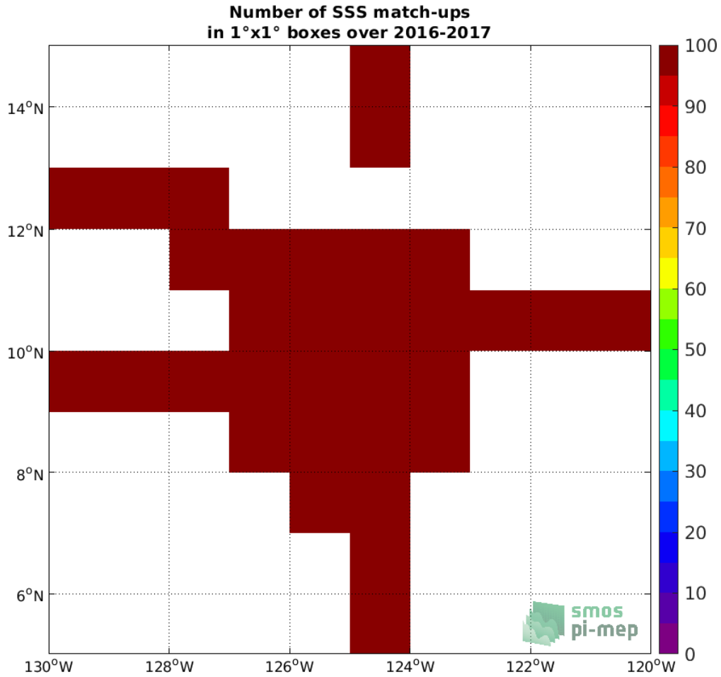
Figure 3: Number of SSS match-ups between Salinity Snake SSS and the SMOS SSS L3 v317 - Monthly - 25 km (CATDS-CPDC) SSS product for the SPURS 2 Pi-MEP region over 1°x1° boxes and for the full satellite product period.
