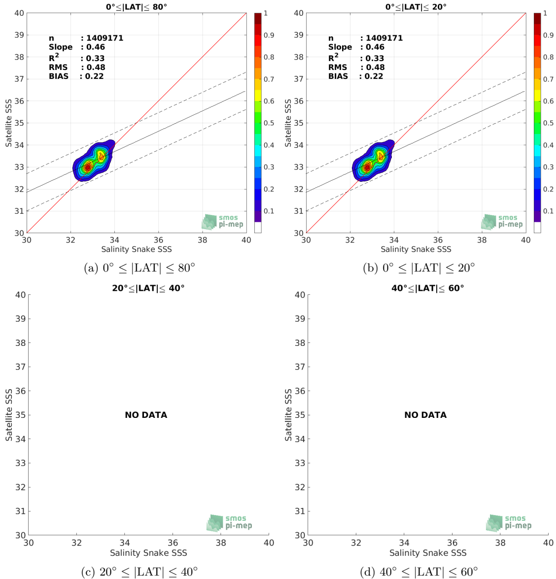
Figure 8: Contour maps of the concentration of SMOS SSS L3 v317 - Monthly - 25 km (CATDS-CPDC) SSS (y-axis) versus Salinity Snake SSS (x-axis) at match-up pairs for different latitude bands. For each plot, the red line shows x=y . The black thin and dashed lines indicate a linear fit through the data cloud and the \pm 95\% confidence levels, respectively. The number match-up pairs n , the slope and R^2 coefficient of the linear fit, the root mean square (RMS) and the mean bias between satellite and in situ data are indicated for each latitude band in each plots.
