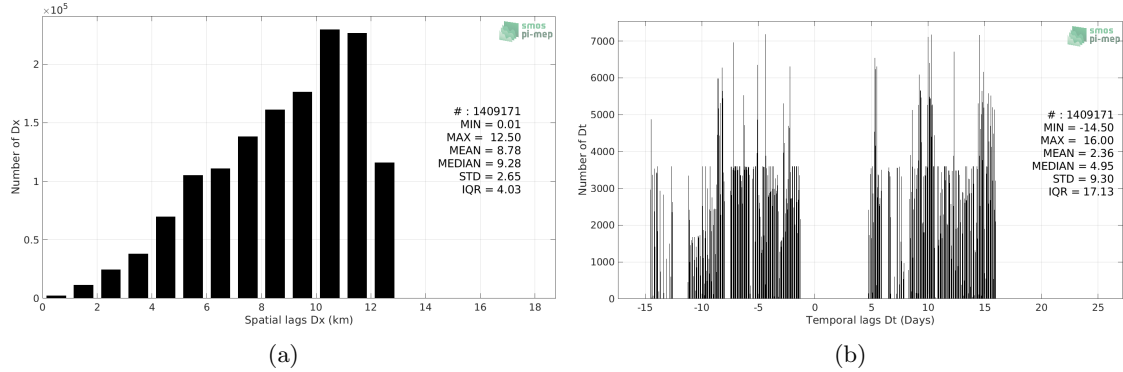
Figure 4: Histograms of the spatial (a) and temporal (b) lags between the location/time of the Salinity Snake measurement and the date of the corresponding SMOS SSS L3 v317 - Monthly - 25 km (CATDS-CPDC) SSS pixel.
