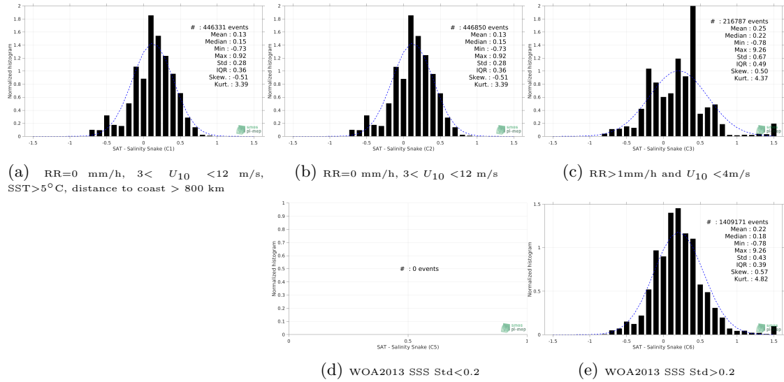
Figure 12: Normalized histogram of \Delta SSS (SMOS SSS L3 v317 - Monthly - 25 km (CATDS-CPDC) - Salinity Snake) for 5 different subdatasets corresponding to: RR=0 mm/h, 3 < U_{10} < 12 m/s, SST > 5°C, distance to coast > 800 km (a), RR=0 mm/h, 3 < U_{10} < 12 m/s (b), RR > 1mm/h and U_{10} < 4 m/s (c), WOA2013 SSS Std < 0.2 (d), WOA2013 SSS Std > 0.2 (e).
