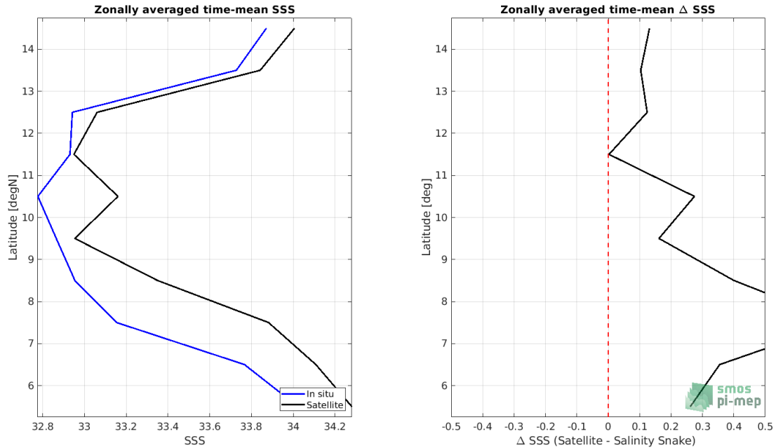
Figure 7: Left panel: Zonal mean SSS from SMOS SSS L3 v317 - Monthly - 25 km (CATDS-CPDC) satellite product (black) and from Salinity Snake (blue). Right panel: Zonal mean of \Delta SSS (Satellite - Salinity Snake) for all the collected Pi-MEP match-up pairs estimated over the full satellite product period.
