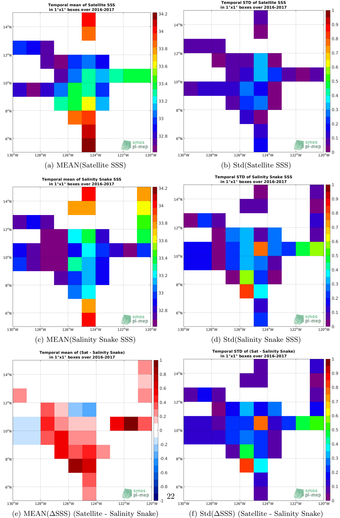
Figure 5: Temporal mean (left) and Std (right) of SSS from SMOS SSS L3 v317 - Monthly - 25 km (CATDS-CPDC) (top), Salinity Snake (middle), and of \Delta SSS (Satellite - Salinity Snake). Only match-up pairs are used to generate these maps.
