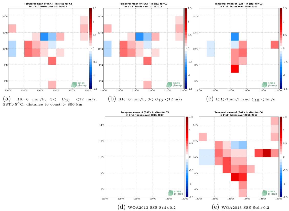
Figure 11: Temporal mean gridded over spatial boxes of size 1^\circ \times 1^\circ of \Delta SSS (SMOS SSS L3 v317 - Monthly - 25 km (CATDS-CPDC) - Salinity Snake) for 5 different subdatasets corresponding to:RR=0 mm/h, 3 < U_{10} < 12 m/s, SST >5^\circ C, distance to coast > 800 km (a), RR=0 mm/h, 3 < U_{10} < 12 m/s (b), RR >1 mm/h and U_{10} < 4 m/s (c), WOA2013 SSS Std <0.2 (d), WOA2013 SSS Std >0.2 (e).
