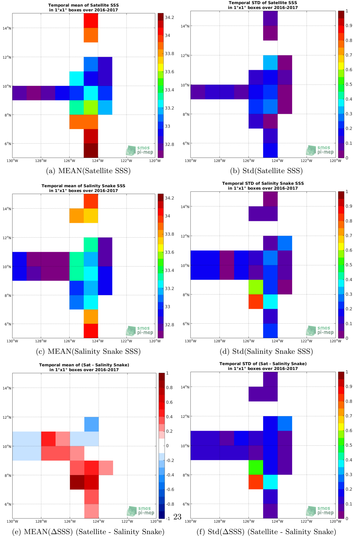
Figure 6: Temporal mean (left) and Std (right) of SSS from SMOS SSS L3 v317 - Monthly - 25 km (CATDS-CPDC) (top), Salinity Snake (middle), and of \Delta SSS (Satellite - Salinity Snake). Only match-up pairs are used to generate these maps.
