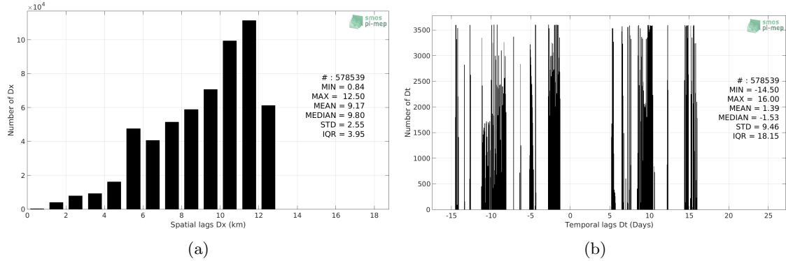
Figure 5: Histograms of the spatial (a) and temporal (b) lags between the time of the Salinity Snake measurements and the date of the corresponding SMOS SSS L3 v317 - Monthly - 25 km (CATDS-CPDC) SSS product.
