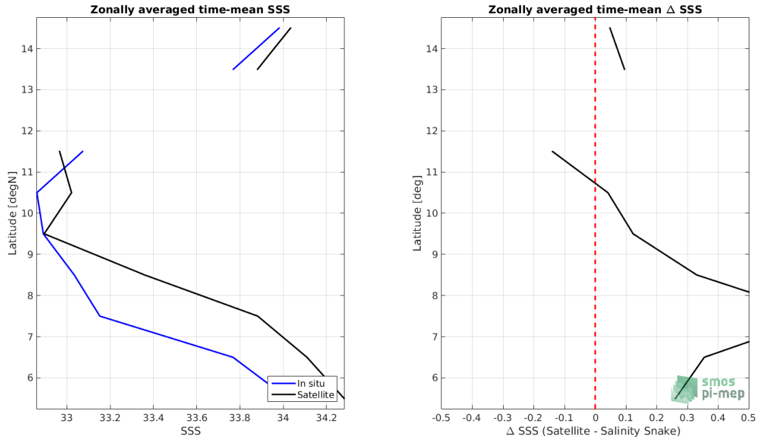
Figure 8: Left panel: Zonal mean SSS from SMOS SSS L3 v317 - Monthly - 25 km (CATDS-CPDC) satellite product (black) and from Salinity Snake (blue). Right panel: Zonal mean of \Delta SSS (Satellite - Salinity Snake) for all the collected Pi-MEP match-up pairs estimated over the full satellite product period.
