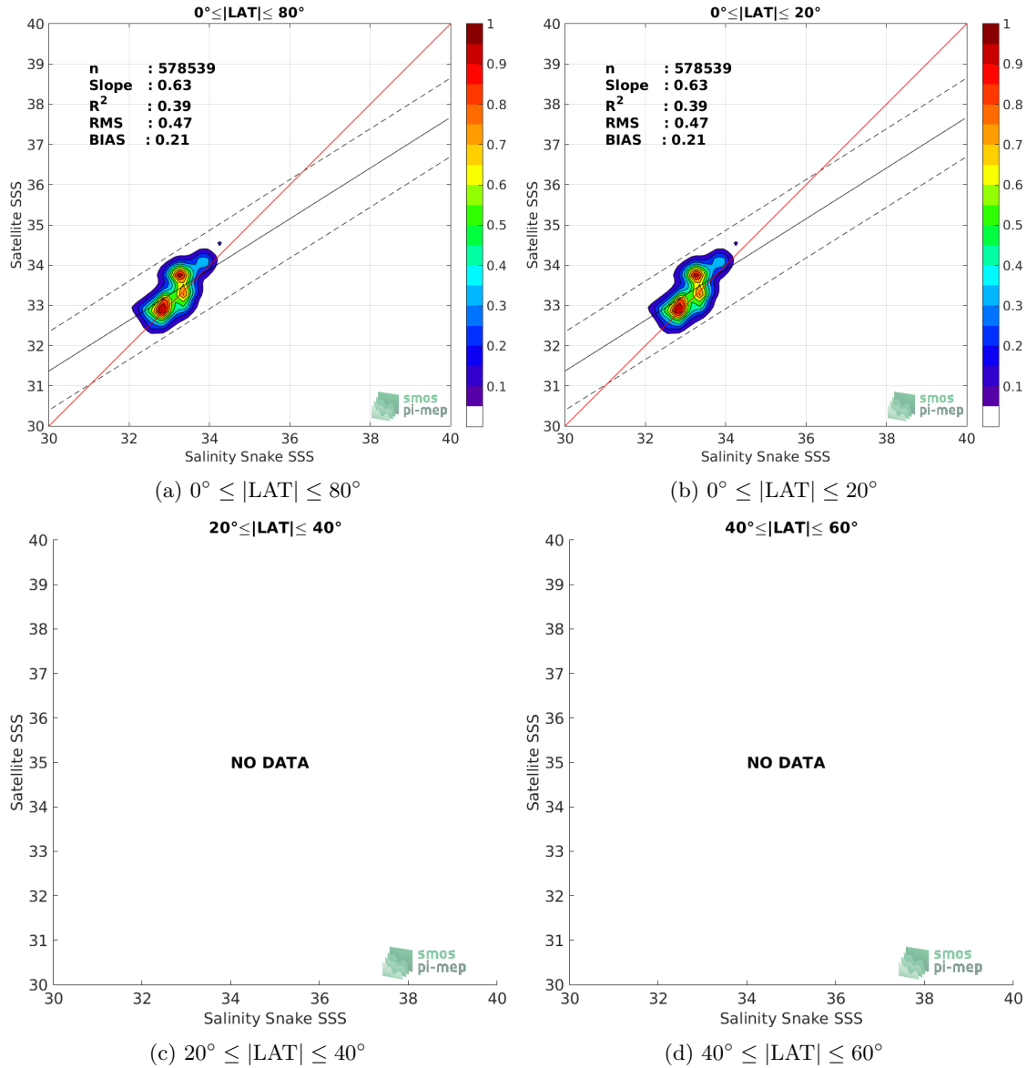
Figure 9: Contour maps of the concentration of SMOS SSS L3 v317 - Monthly - 25 km (CATDS-CPDC) SSS (y-axis) versus Salinity Snake SSS (x-axis) at match-up pairs for different latitude bands. For each plot, the red line shows x=y . The black thin and dashed lines indicate a linear fit through the data cloud and the \pm 95\% confidence levels, respectively. The number match-up pairs n , the slope and R^2 coefficient of the linear fit, the root mean square (RMS) and the mean bias between satellite and in situ data are indicated for each latitude band in each plots.
