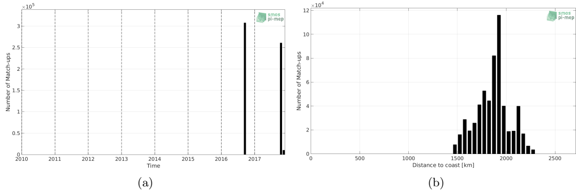
Figure 1: Number of match-ups between Salinity Snake and SMOS SSS L3 v317 - Monthly - 25 km (CATDS-CPDC) SSS as a function of time (a) and as function of the distance to coast (b) over the SPURS 2 Pi-MEP region and for the full satellite product period.
