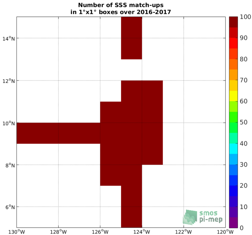
Figure 4: Number of SSS match-ups between Salinity Snake SSS and the SMOS SSS L3 v317 - Monthly - 25 km (CATDS-CPDC) SSS product for the SPURS 2 Pi-MEP region over 1°x1° boxes and for the full satellite product period.
