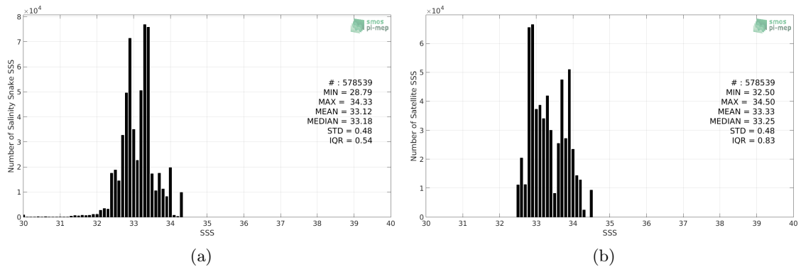
Figure 2: Histograms of SSS from Salinity Snake (a) and SMOS SSS L3 v317 - Monthly - 25 km (CATDS-CPDC) (b) considering all match-up pairs per bins of 0.1 over the SPURS 2 Pi-MEP region and for the full satellite product period.
