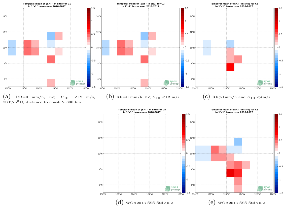
Figure 12: Temporal mean gridded over spatial boxes of size 1^\circ \times 1^\circ of \Delta SSS (SMOS SSS L3 v317 - Monthly - 25 km (CATDS-CPDC) - Salinity Snake) for 5 different subdatasets corresponding to:RR=0 mm/h, 3 < U_{10} < 12 m/s, SST >5^\circ\text{C} , distance to coast > 800 km (a), RR=0 mm/h, 3 < U_{10} < 12 m/s (b), RR >1 mm/h and U_{10} < 4 m/s (c), WOA2013 SSS Std <0.2 (d), WOA2013 SSS Std >0.2 (e).
