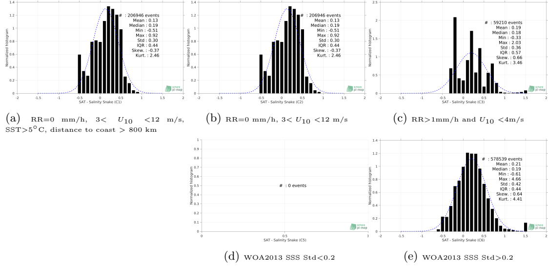
Figure 13: Normalized histogram of \Delta SSS (SMOS SSS L3 v317 - Monthly - 25 km (CATDS-CPDC) - Salinity Snake) for 5 different subdatasets corresponding to: RR=0 mm/h, 3 < U_{10} < 12 m/s, SST > 5°C, distance to coast > 800 km (a), RR=0 mm/h, 3 < U_{10} < 12 m/s (b), RR > 1mm/h and U_{10} < 4 m/s (c), WOA2013 SSS Std < 0.2 (d), WOA2013 SSS Std > 0.2 (e).
