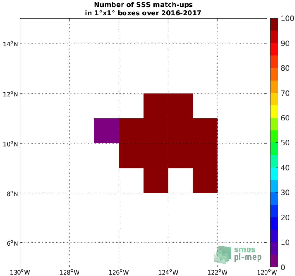
Figure 3: Number of SSS match-ups between Seaglider SSS and the SMOS SSS L3 v317 - Monthly - 25 km (CATDS-CPDC) SSS product for the SPURS 2 Pi-MEP region over 1^\circ \times 1^\circ boxes and for the full satellite product period.
