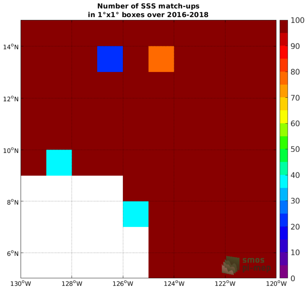
Figure 3: Number of SSS match-ups between Surface drifters SSS and the SMOS SSS L3 v317 - Monthly - 25 km (CATDS-CPDC) SSS product for the SPURS 2 Pi-MEP region over 1°x1° boxes and for the full satellite product period.
