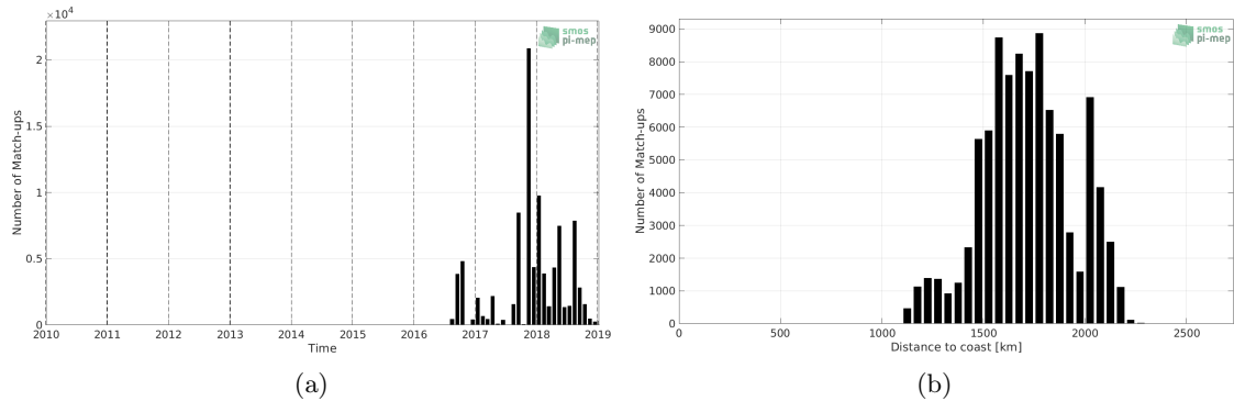
Figure 1: Number of match-ups between Surface drifters and SMOS SSS L3 v317 - Monthly - 25 km (CATDS-CPDC) SSS as a function of time (a) and as function of the distance to coast (b) over the SPURS 2 Pi-MEP region and for the full satellite product period.
