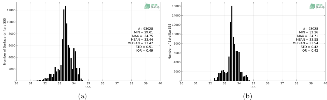
Figure 2: Histograms of SSS from Surface drifters (a) and SMOS SSS L3 v317 - Monthly - 25 km (CATDS-CPDC) (b) considering all match-up pairs per bins of 0.1 over the SPURS 2 Pi-MEP region and for the full satellite product period.
