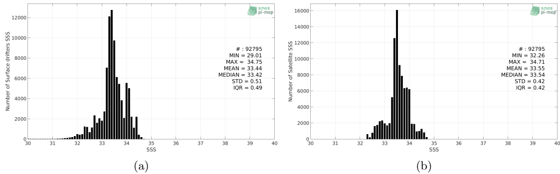
Figure 2: Histograms of SSS from Surface drifters (a) and SMOS SSS L3 v317 - Monthly - 25 km (CATDS-CPDC) (b) considering all match-up pairs per bins of 0.1 over the SPURS 2 Pi-MEP region and for the full satellite product period.
