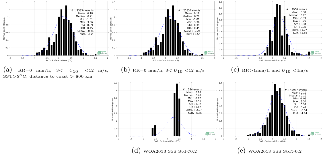
Figure 12: Normalized histogram of \Delta\text{SSS} (SMOS-L3-CATDS-CPDC-V317-MONTHLY-25KM - Surface drifters) for 5 different subdatasets corresponding to: RR=0 mm/h, 3 < U_{10} < 12 m/s, SST >5^{\circ}\text{C} , distance to coast > 800 km (a), RR=0 mm/h, 3 < U_{10} < 12 m/s (b), RR >1 mm/h and U_{10} < 4 m/s (c), WOA2013 SSS Std <0.2 (d), WOA2013 SSS Std >0.2 (e).
