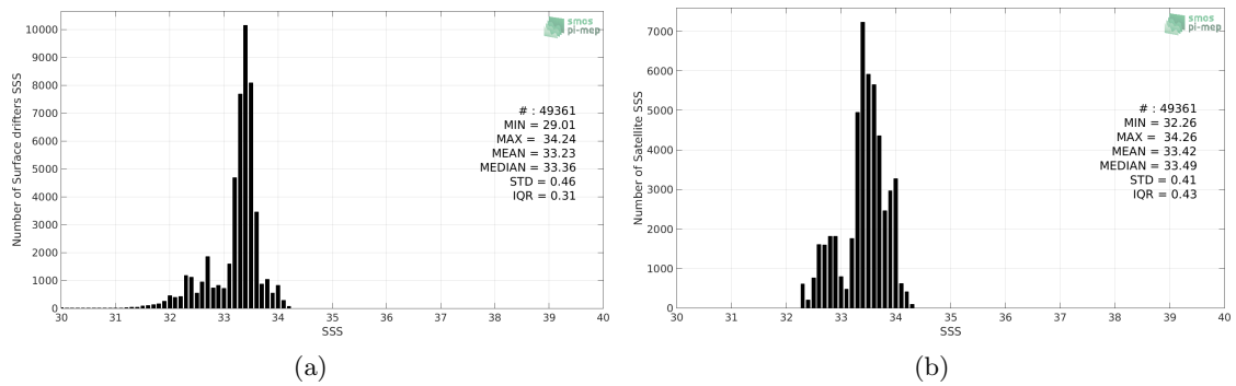
Figure 2: Histograms of SSS from Surface drifters (a) and SMOS-L3-CATDS-CPDC-V317-MONTHLY-25KM (b) considering all match-up pairs per bins of 0.1 over the SPURS 2 Pi-MEP region and for the full satellite product period.
