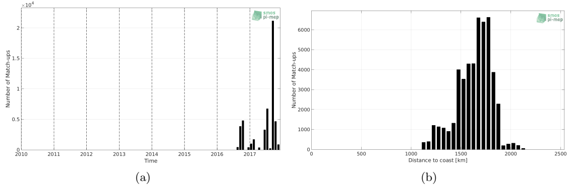
Figure 1: Number of match-ups between Surface drifters and SMOS-L3-CATDS-CPDC-V317-MONTHLY-25KM SSS as a function of time (a) and as function of the distance to coast (b) over the SPURS 2 Pi-MEP region and for the full satellite product period.
