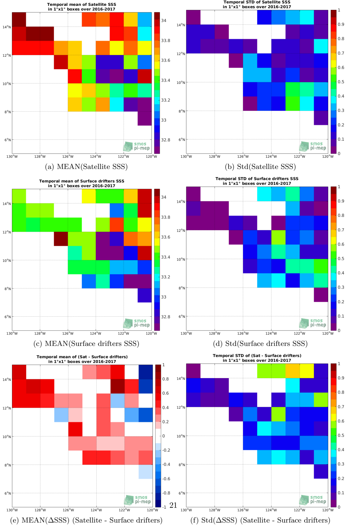
Figure 5: Temporal mean (left) and Std (right) of SSS from SMOS-L3-CATDS-CPDC-V317-MONTHLY-25KM (top), Surface drifters (middle), and of \Delta SSS (Satellite - Surface drifters). Only match-up pairs are used to generate these maps.
