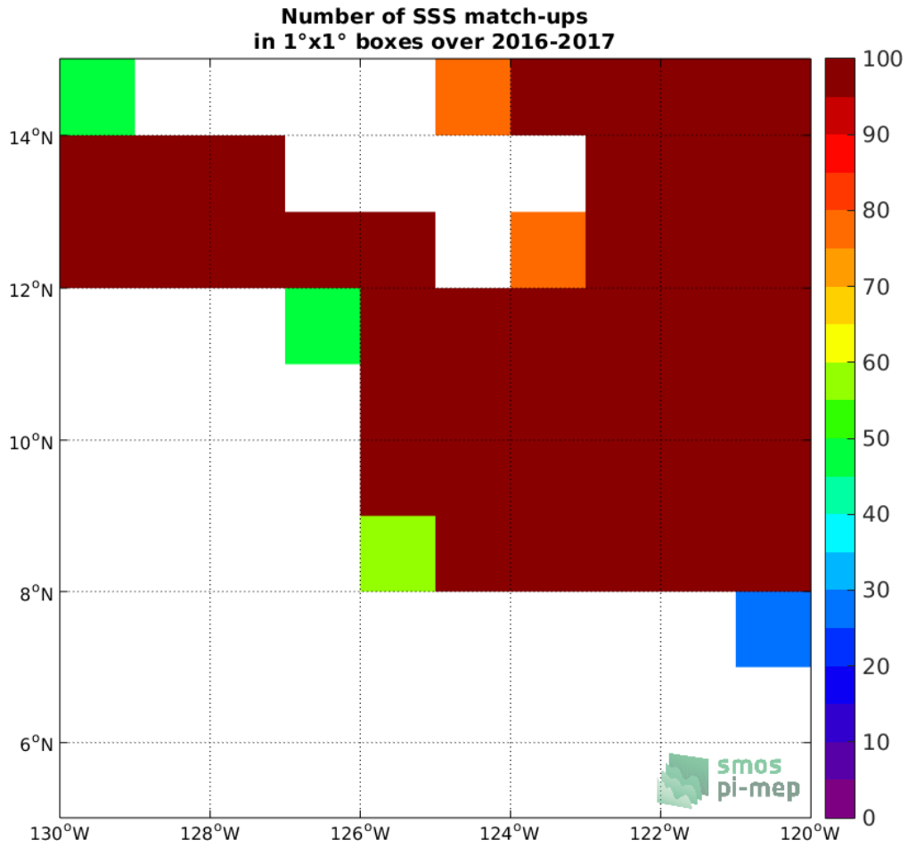
Figure 3: Number of SSS match-ups between Surface drifters SSS and the SMOS-L3-CATDS-CPDC-V317-MONTHLY-25KM SSS product for the SPURS 2 Pi-MEP region over 1°x1° boxes and for the full satellite product period.
