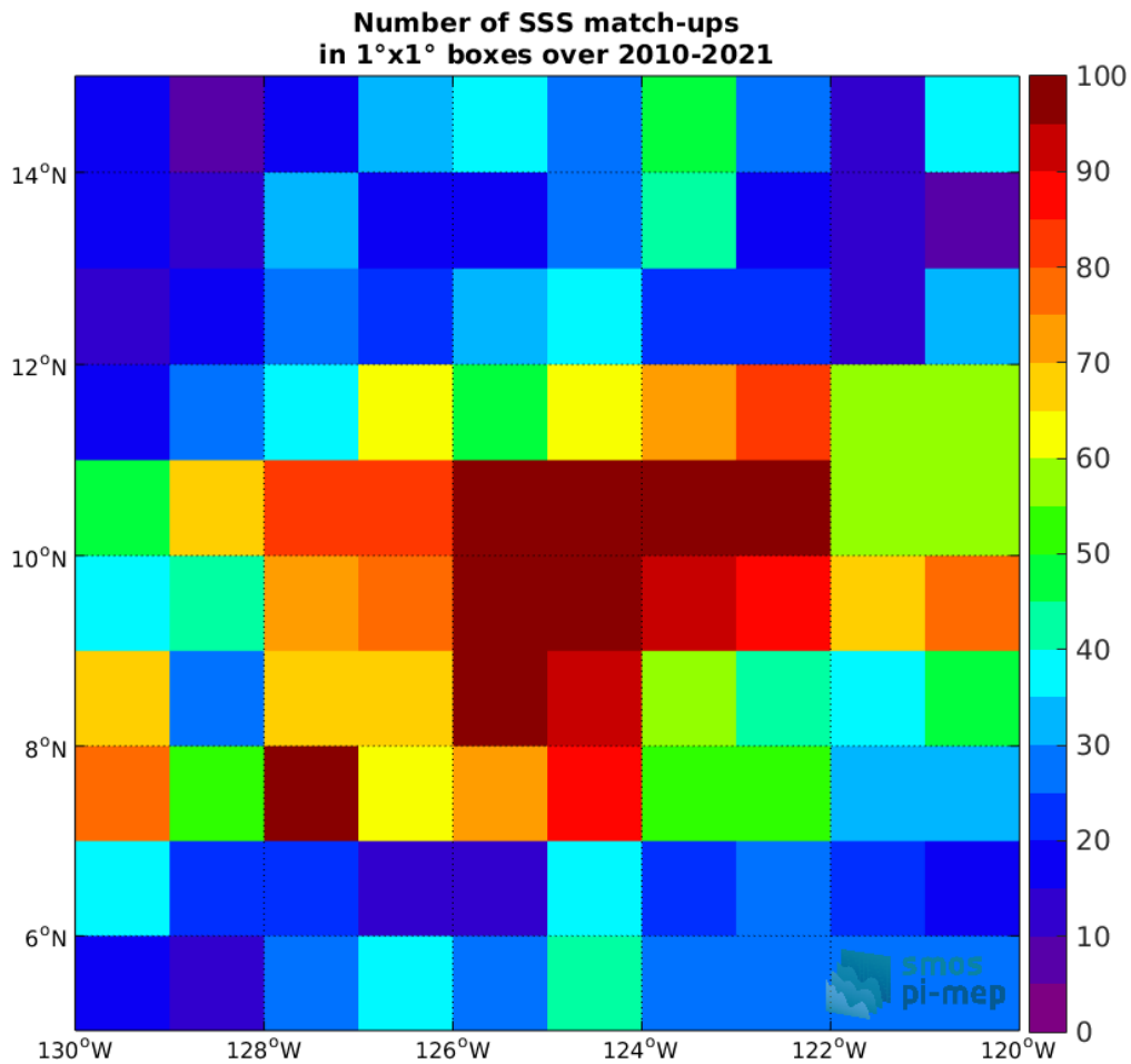
Figure 4: Number of SSS match-ups between Argo SSS and the SMOS SSS L3 v317 - Monthly - 25 km (CATDS-CPDC) SSS product for the SPURS 2 Pi-MEP region over 1°×1° boxes and for the full satellite product period.
