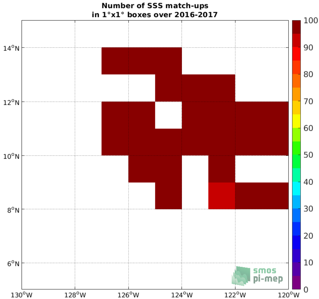
Figure 3: Number of SSS match-ups between Waveglider SSS and the SMOS SSS L3 v317 - 10 Days - 25 km (CATDS-CPDC) SSS product for the SPURS 2 Pi-MEP region over 1^\circ \times 1^\circ boxes and for the full satellite product period.
